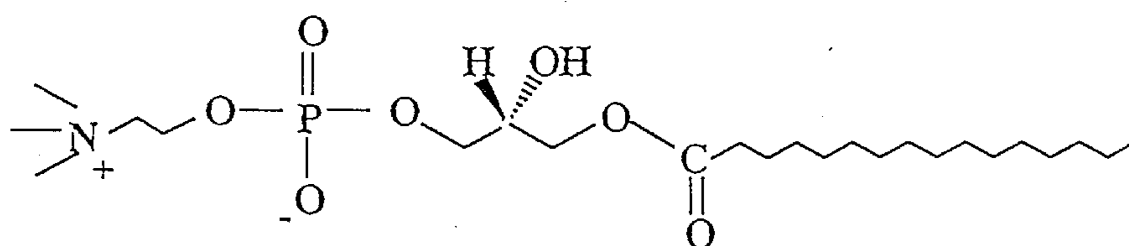
1-Palmitoyl-2-Hydroxy- sn -Glycero-3-Phosphocholine (MPPC)
