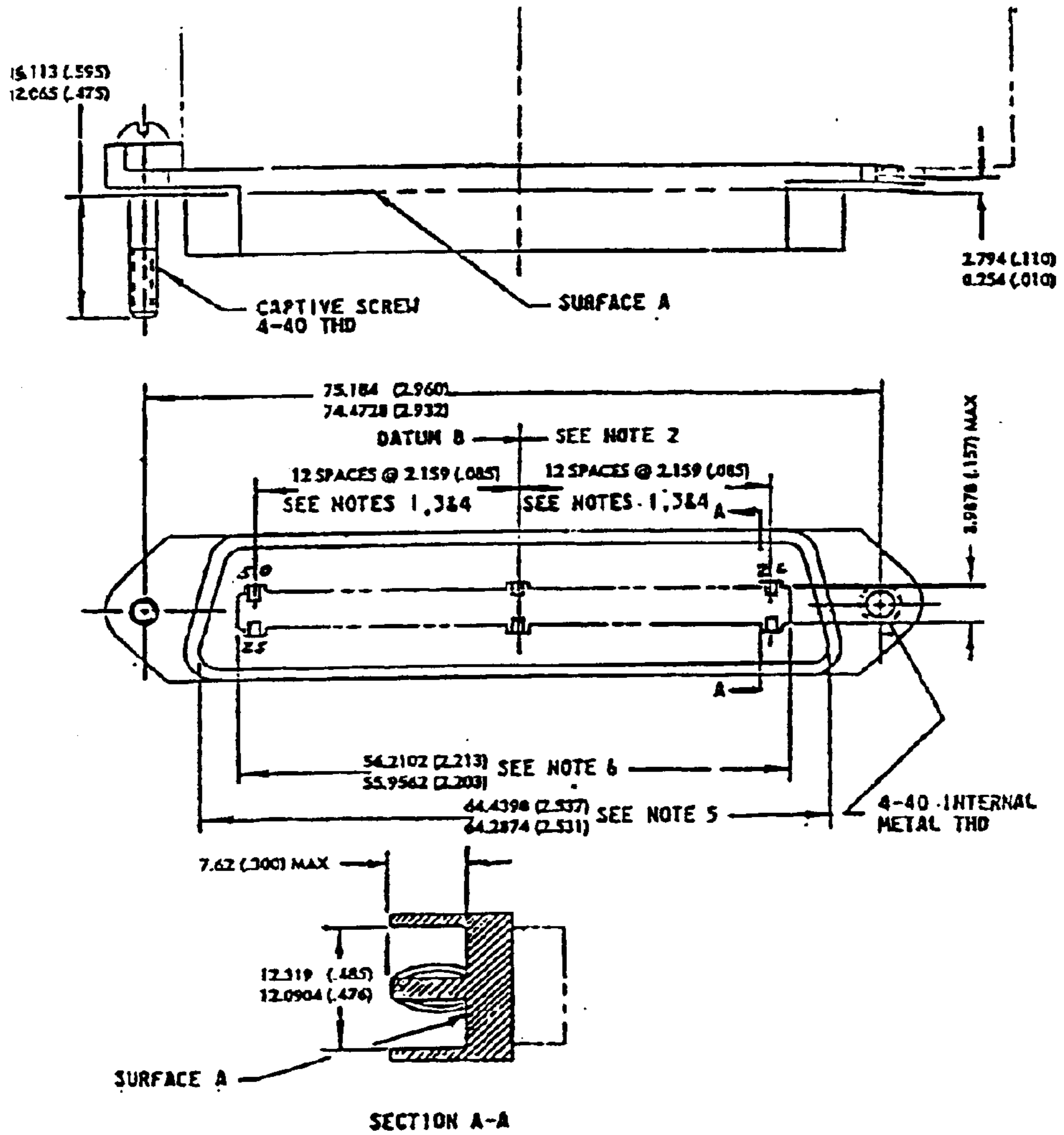
Figure 68.500(a)(1)—50 Pinless Miniature Ribbon Plug
