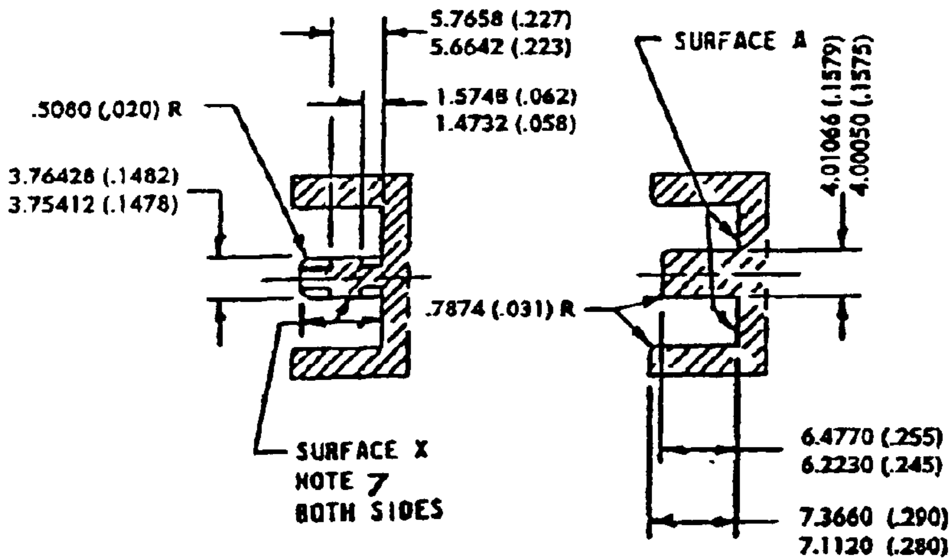
SECTION B-B
