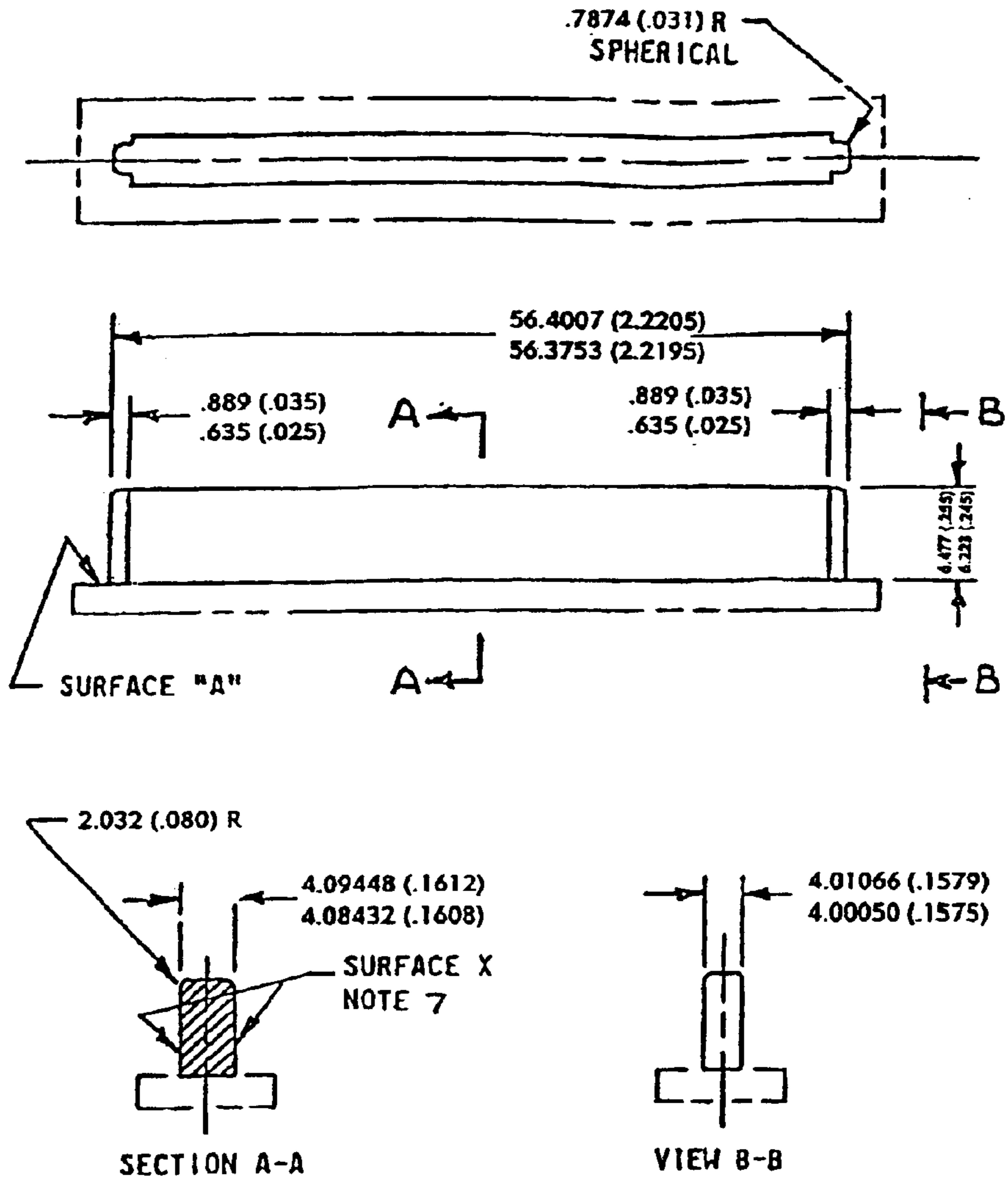
Figure 68.500(F)(2)--50 Position Miniature Ribbon Jack Sizing Gauge
