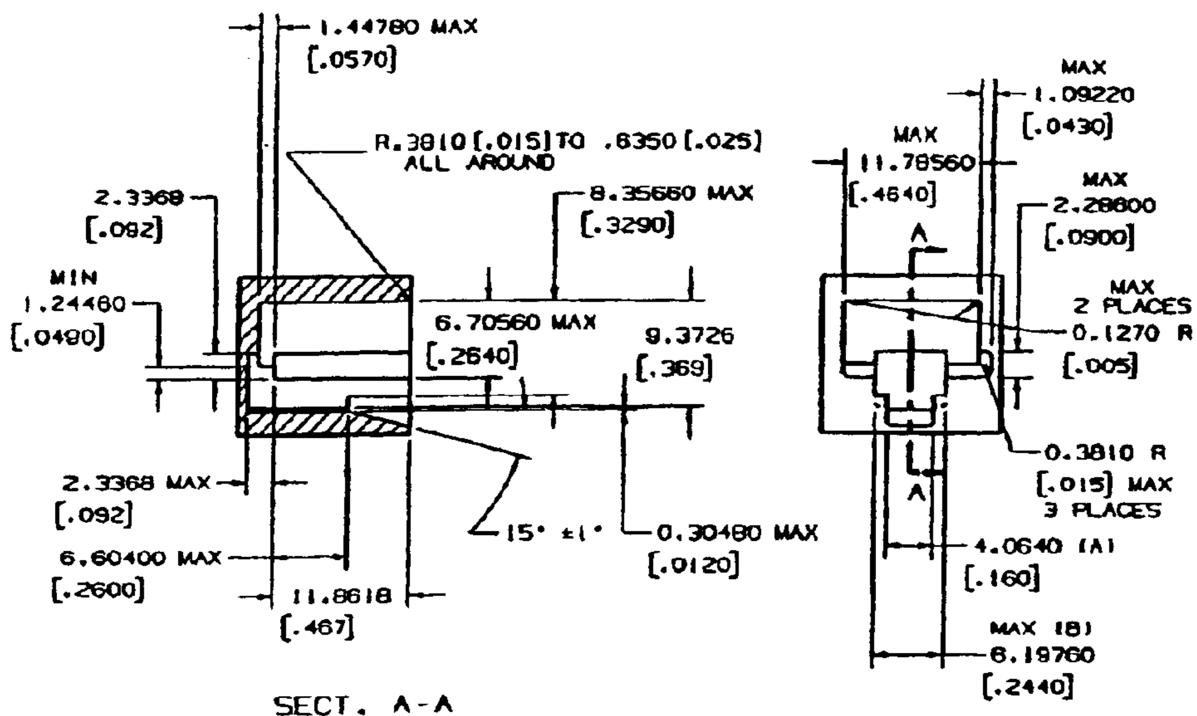
GO GAUGE
