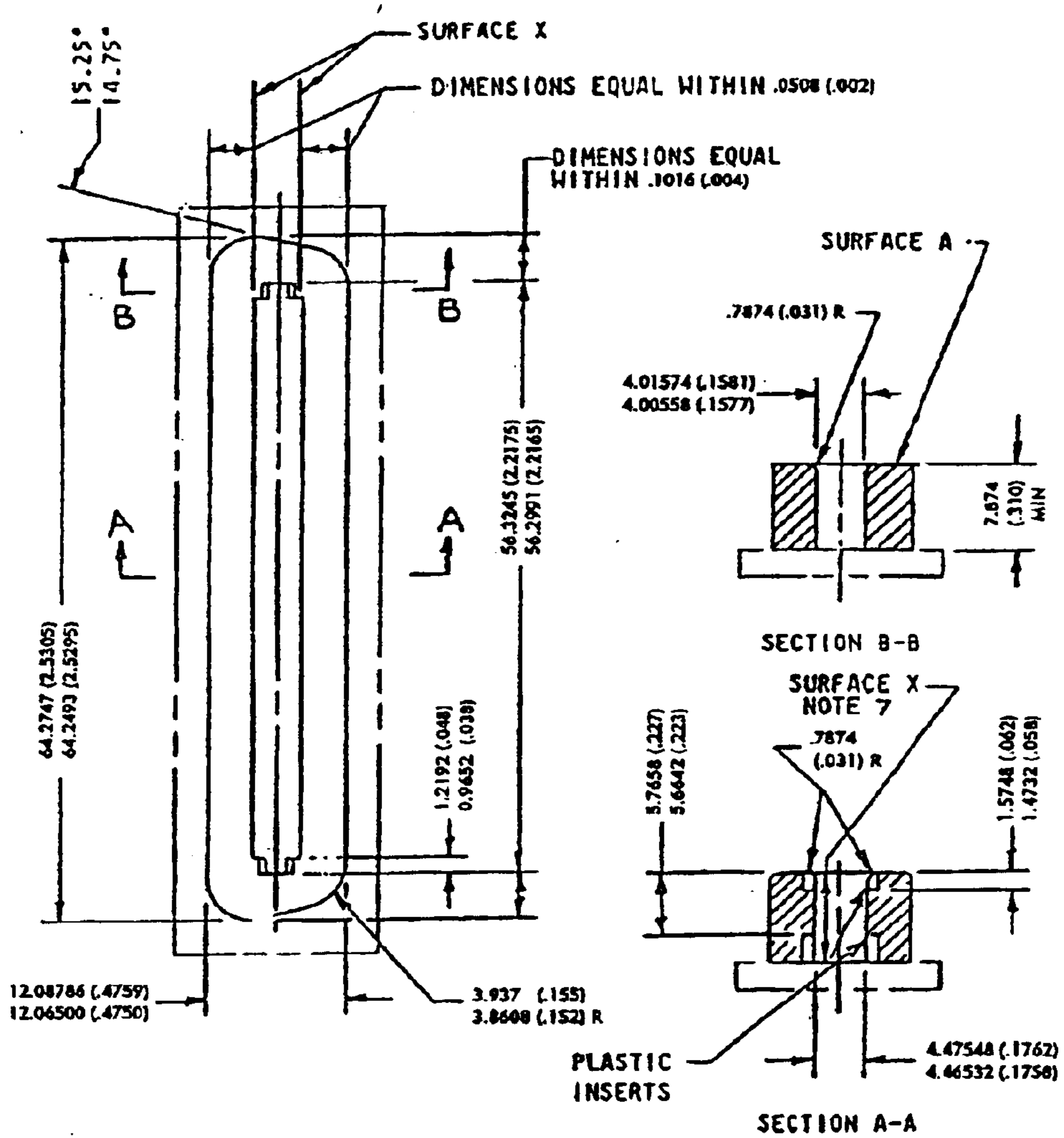
Figure 68.500(e)(3)--50 Position Miniature Ribbon Plug Continuity Gauge
