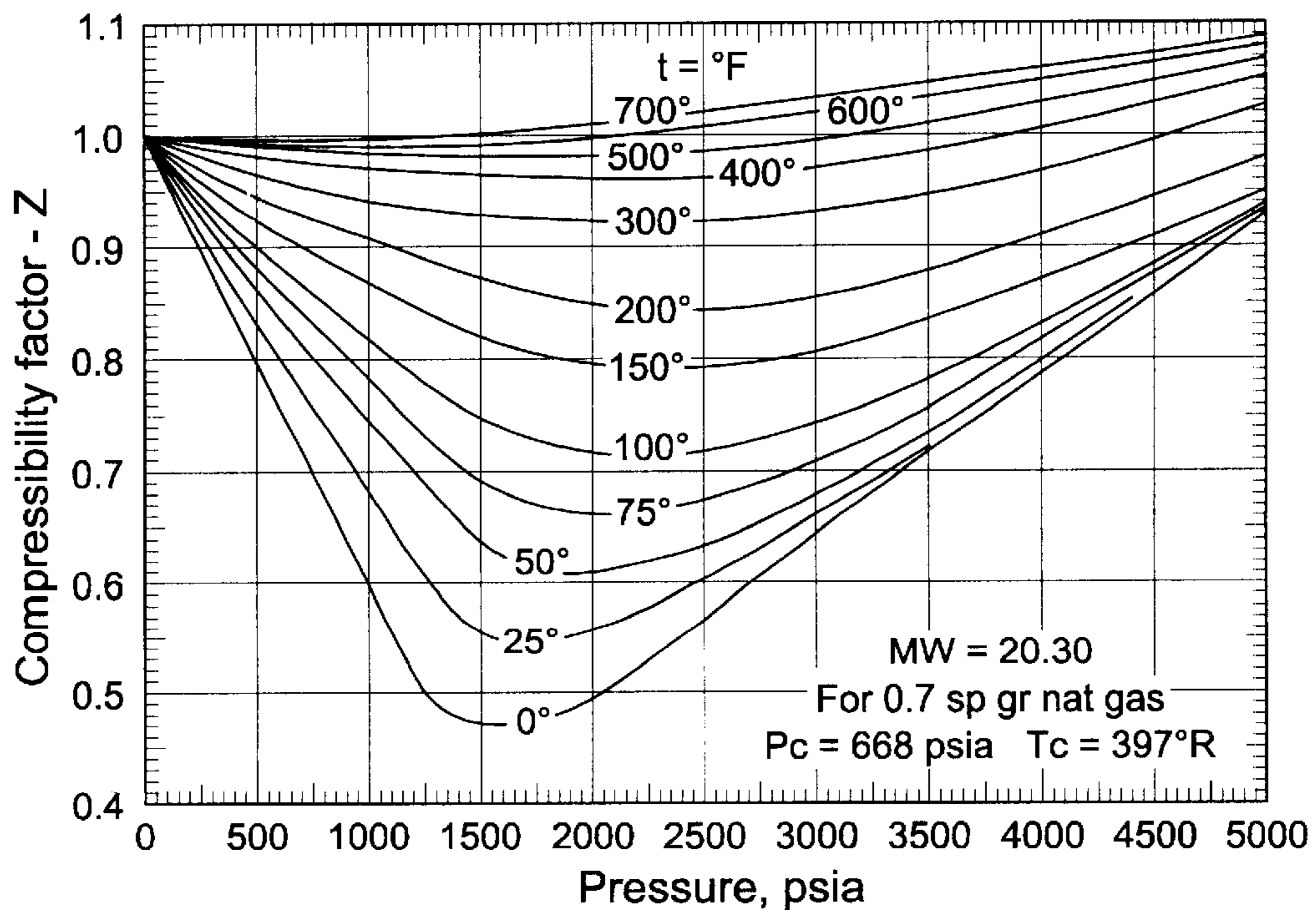
Fig. 2 Compressibility Factor for Natural Gas S. G. = 0.7
