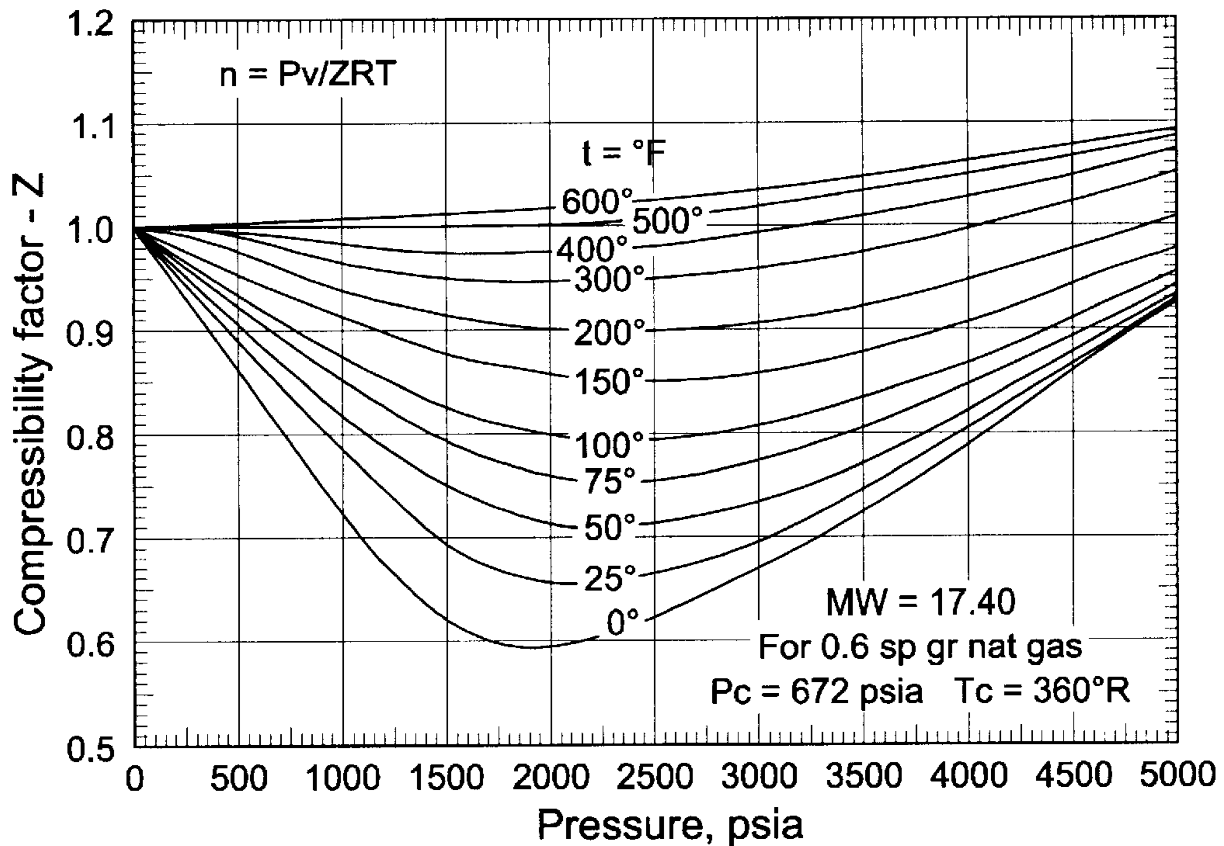
Fig. 1 Compressibility Factor for Natural Gas S. G. = 0.6
