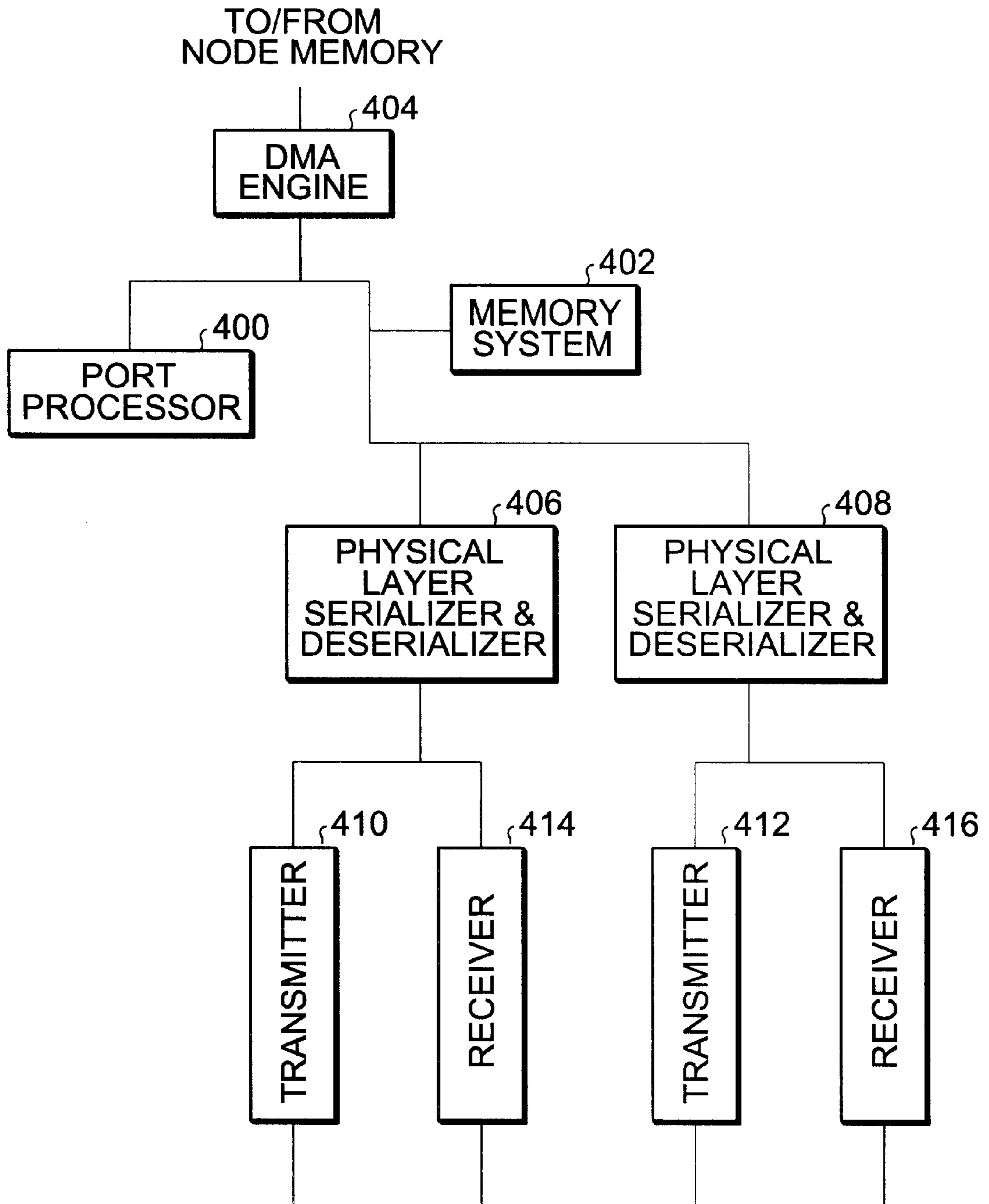
DUAL-PORT HBA BLOCK DIAGRAM
