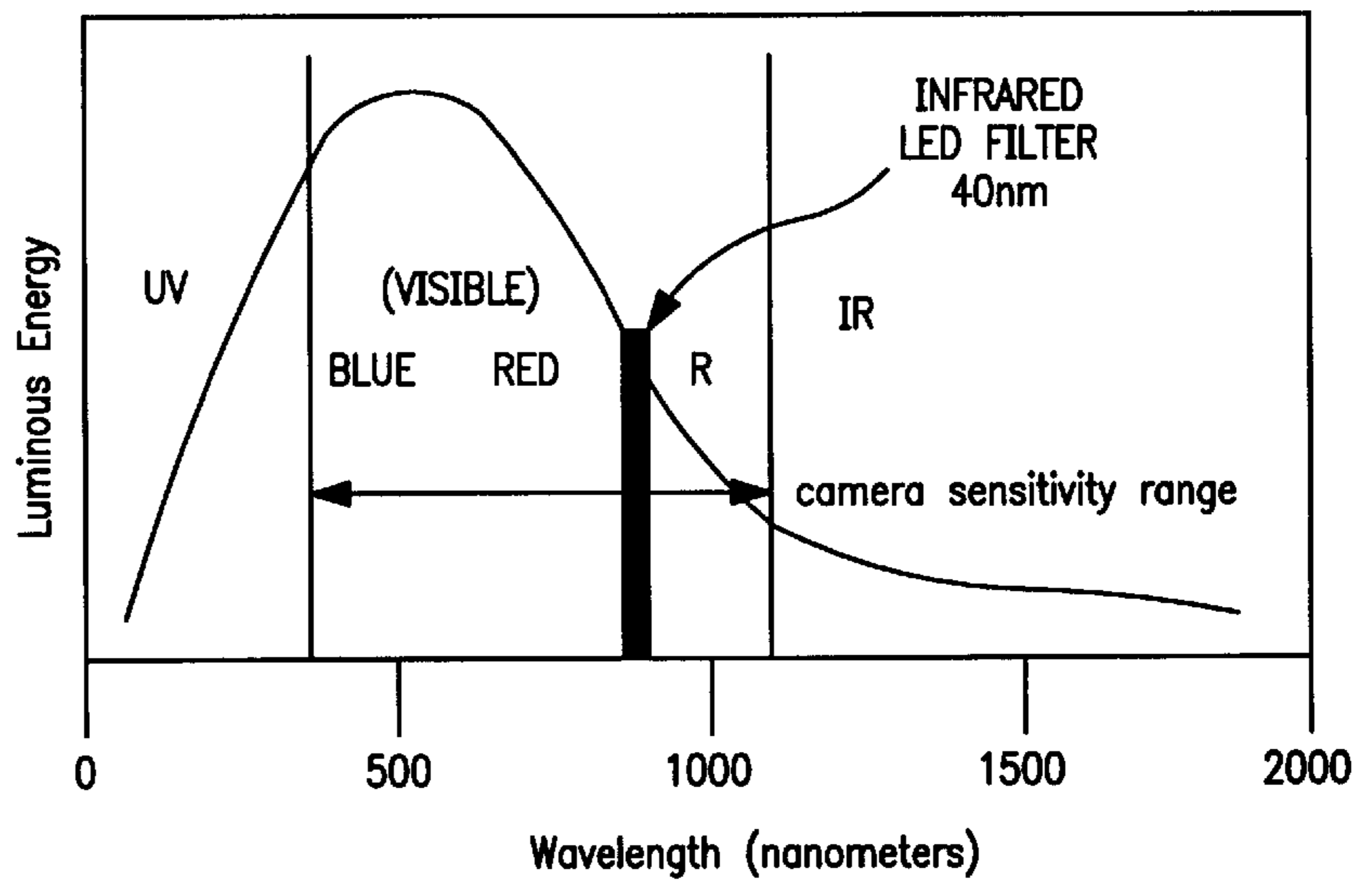
Luminance Curve for Sunlight
