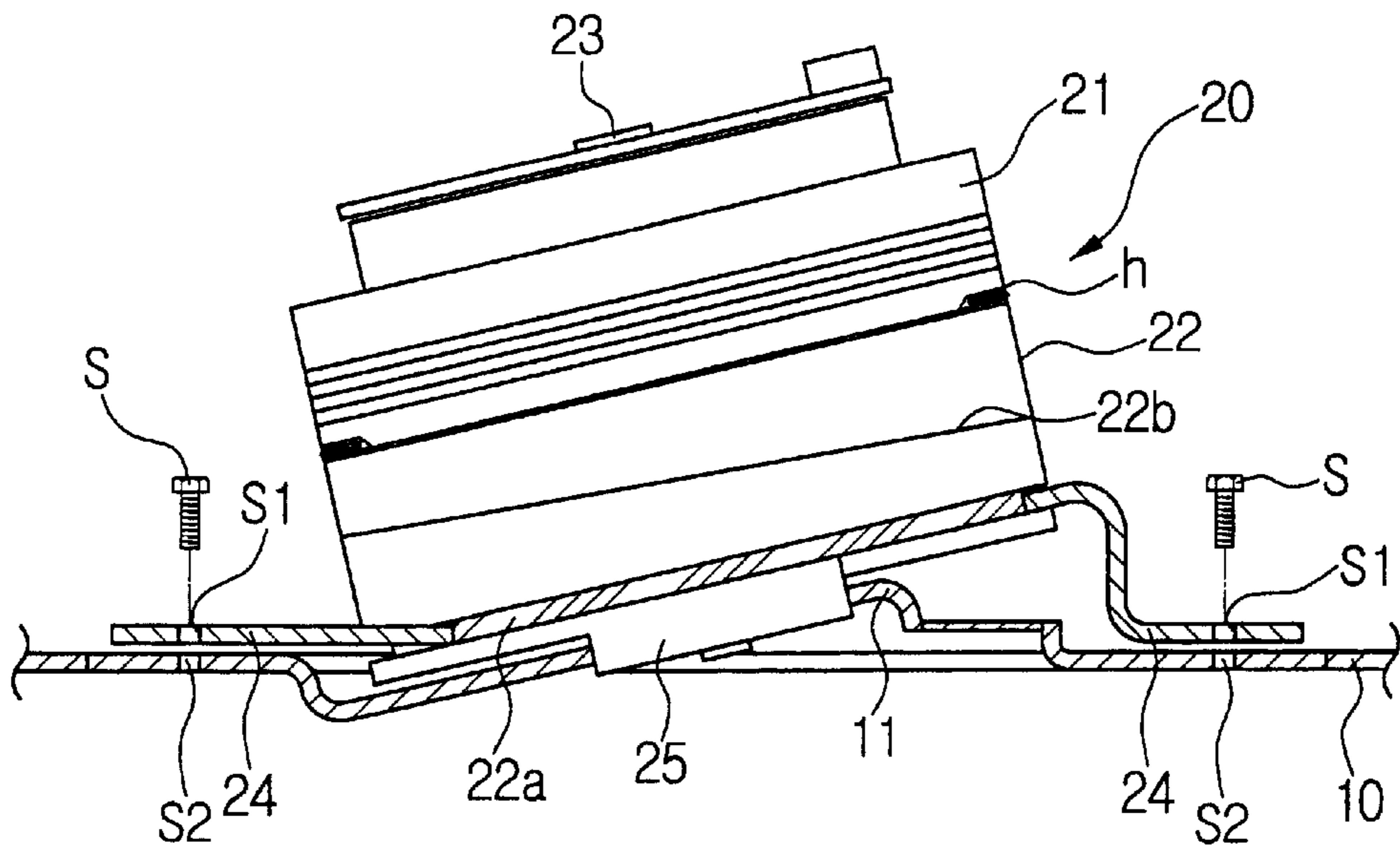
FIG. 2 (PRIOR ART)
