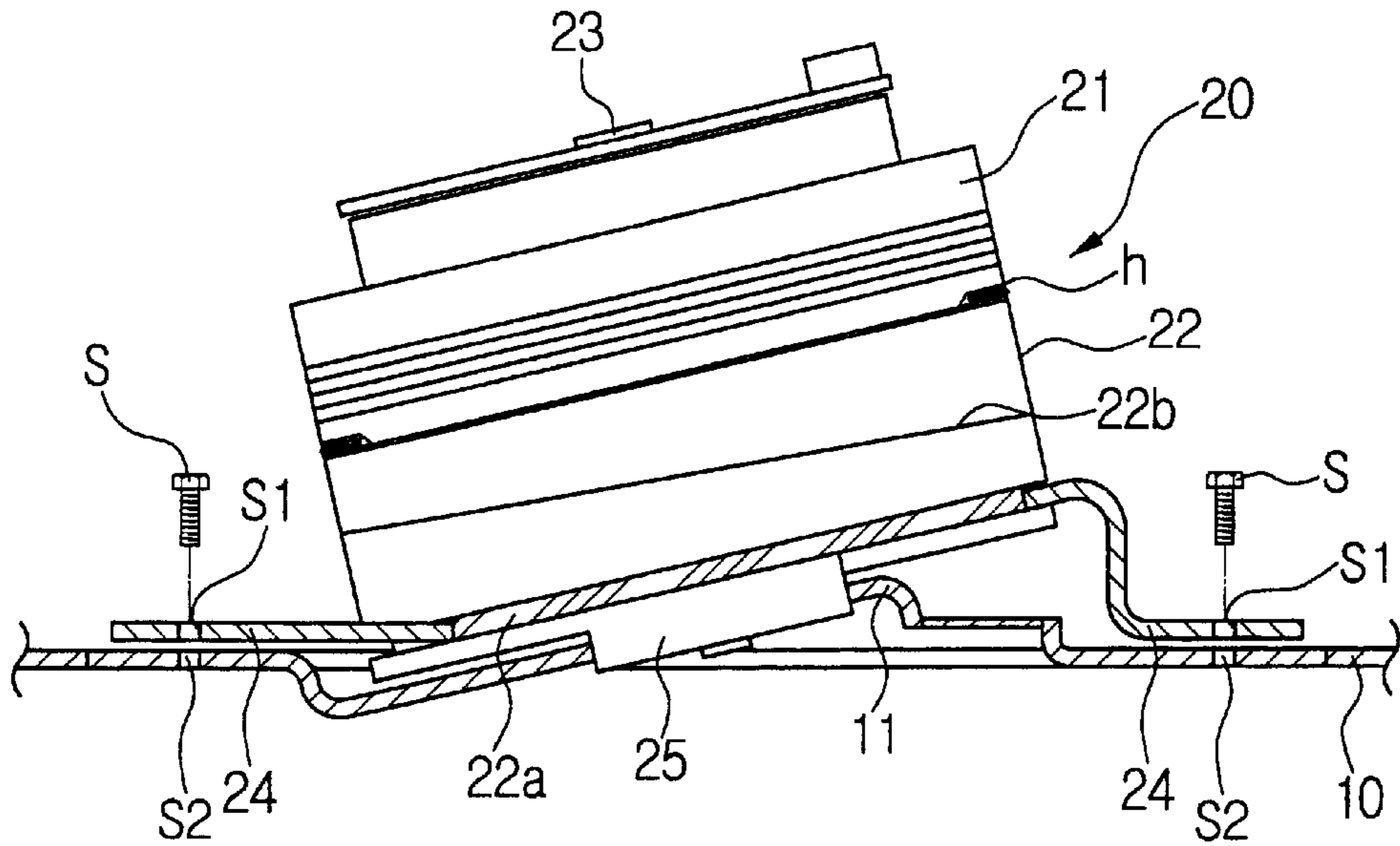
FIG. 2 (PRIOR ART)
