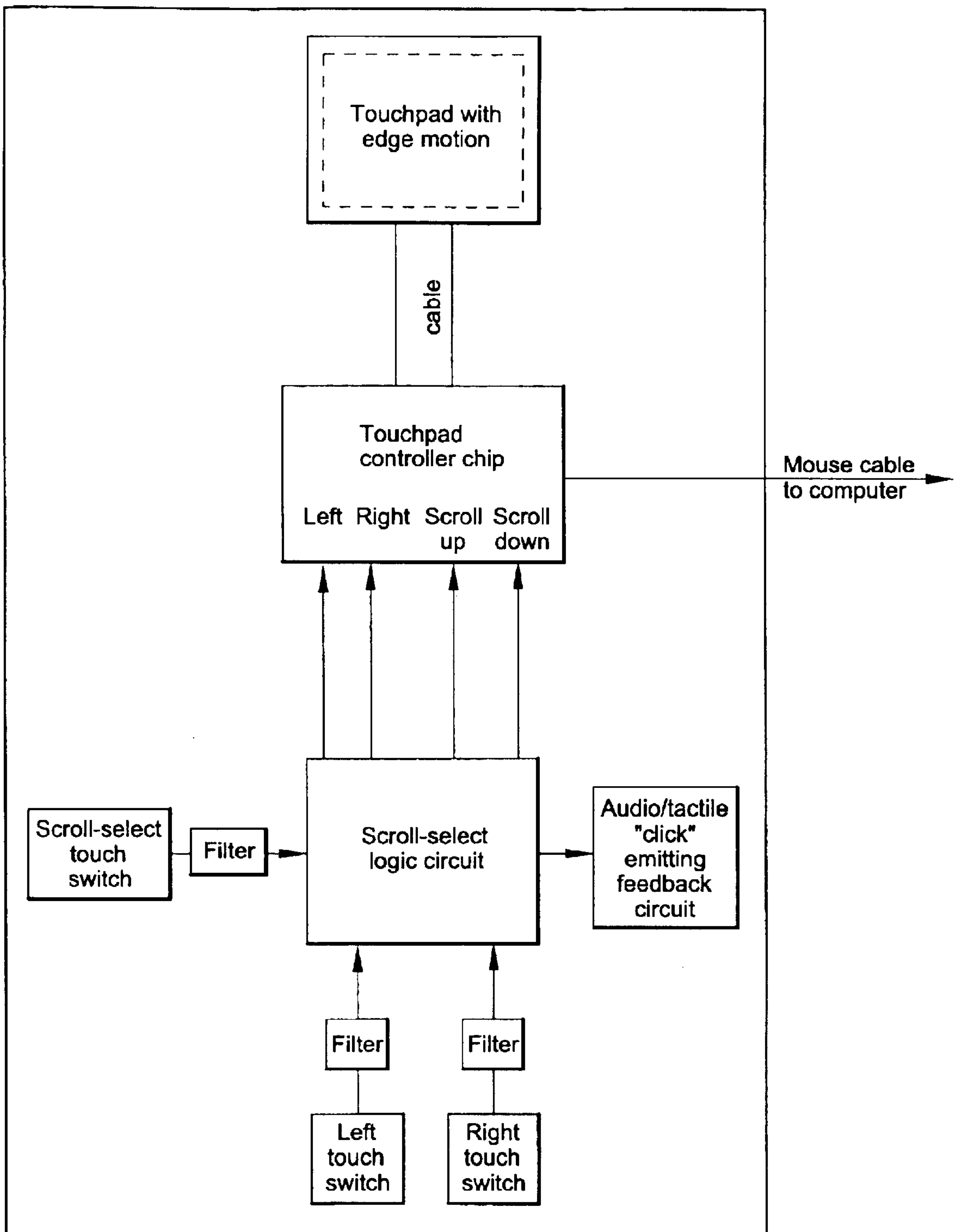
TOUCHPAD-BASED POINTING DEVICE INTERNAL CIRCUITRY BLOCK DIAGRAM
