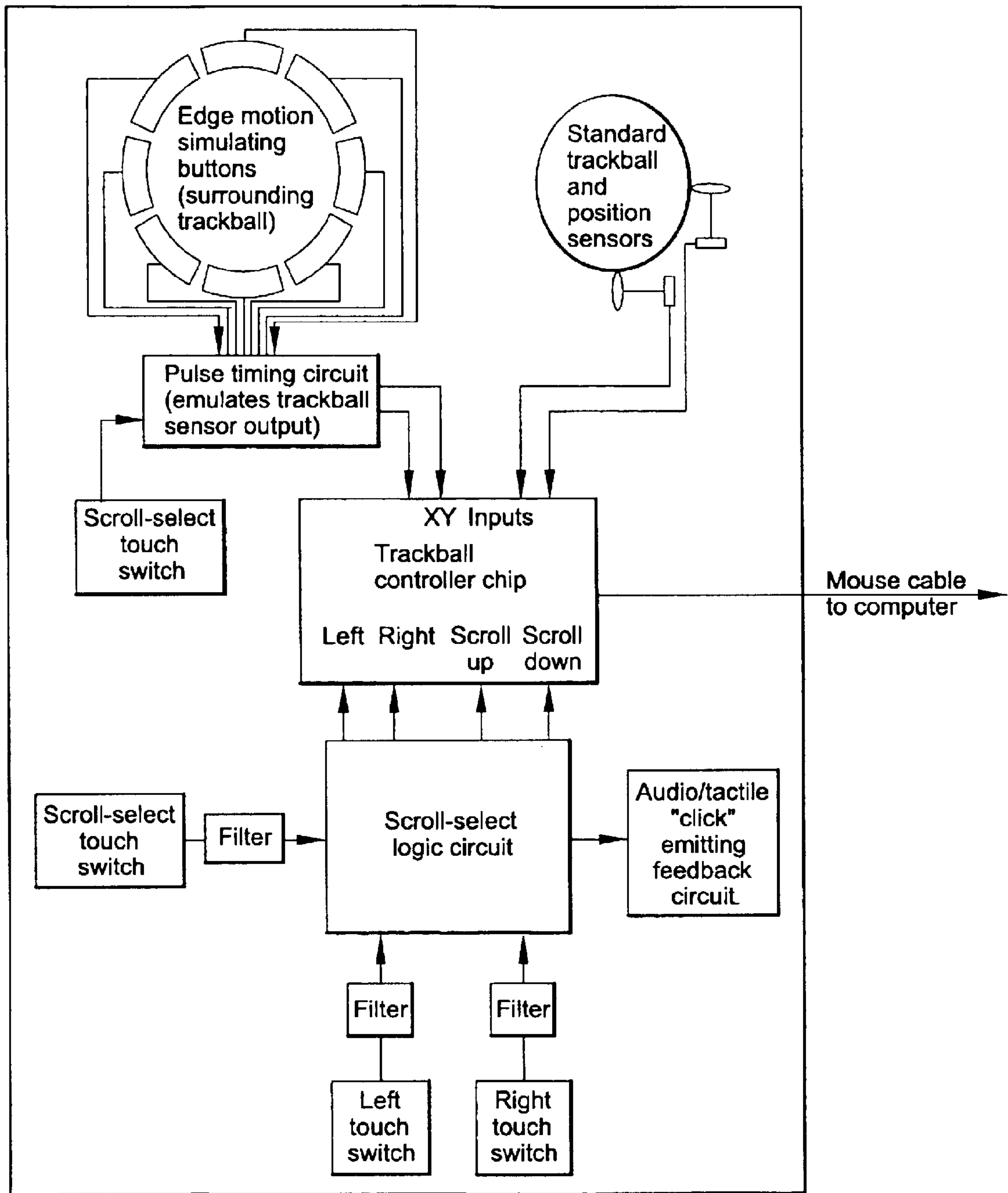
TRACK BALL-BASED POINTING DEVICE INTERNAL CIRCUITRY BLOCK DIAGRAM
