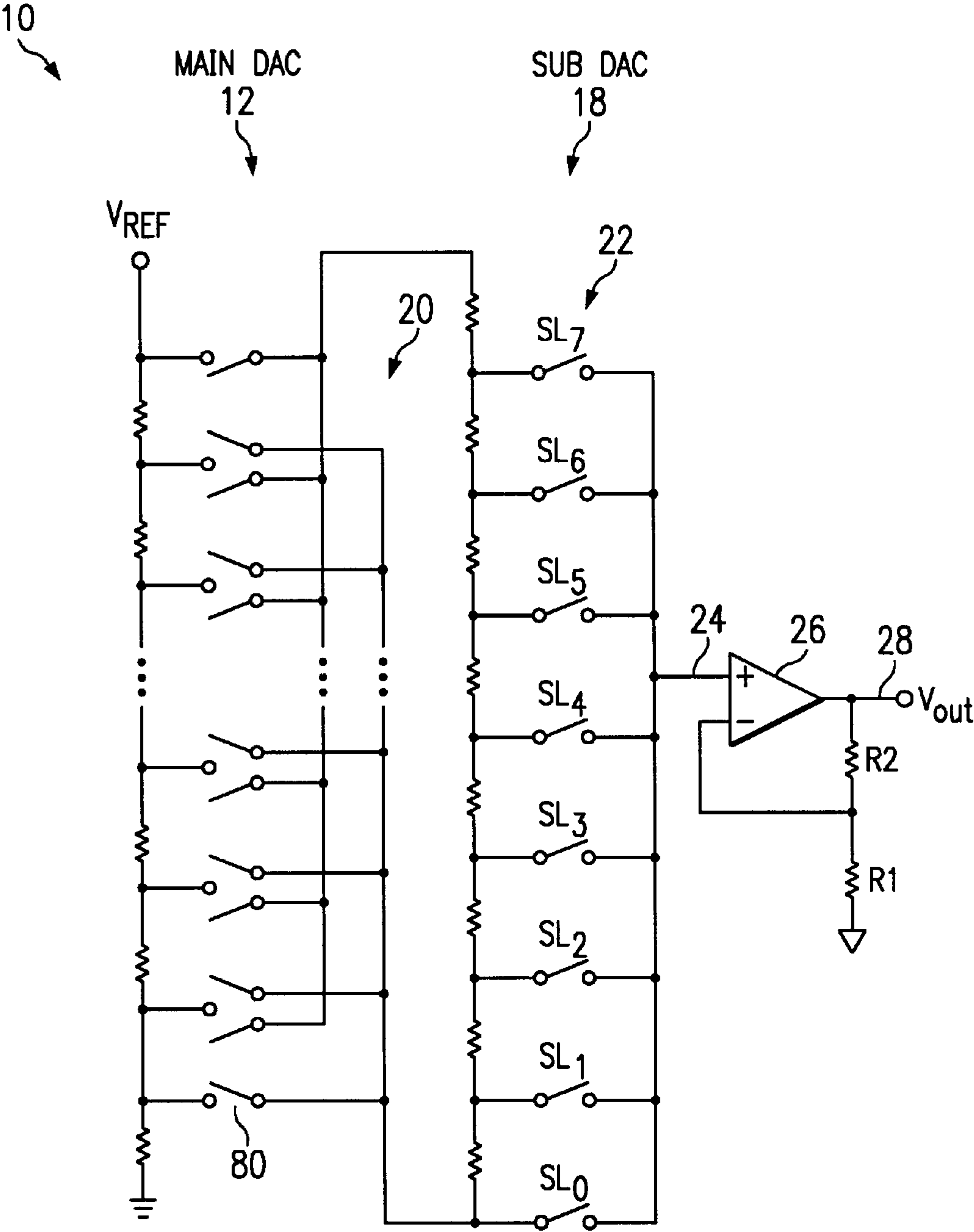
FIG. 1 (PRIOR ART)
