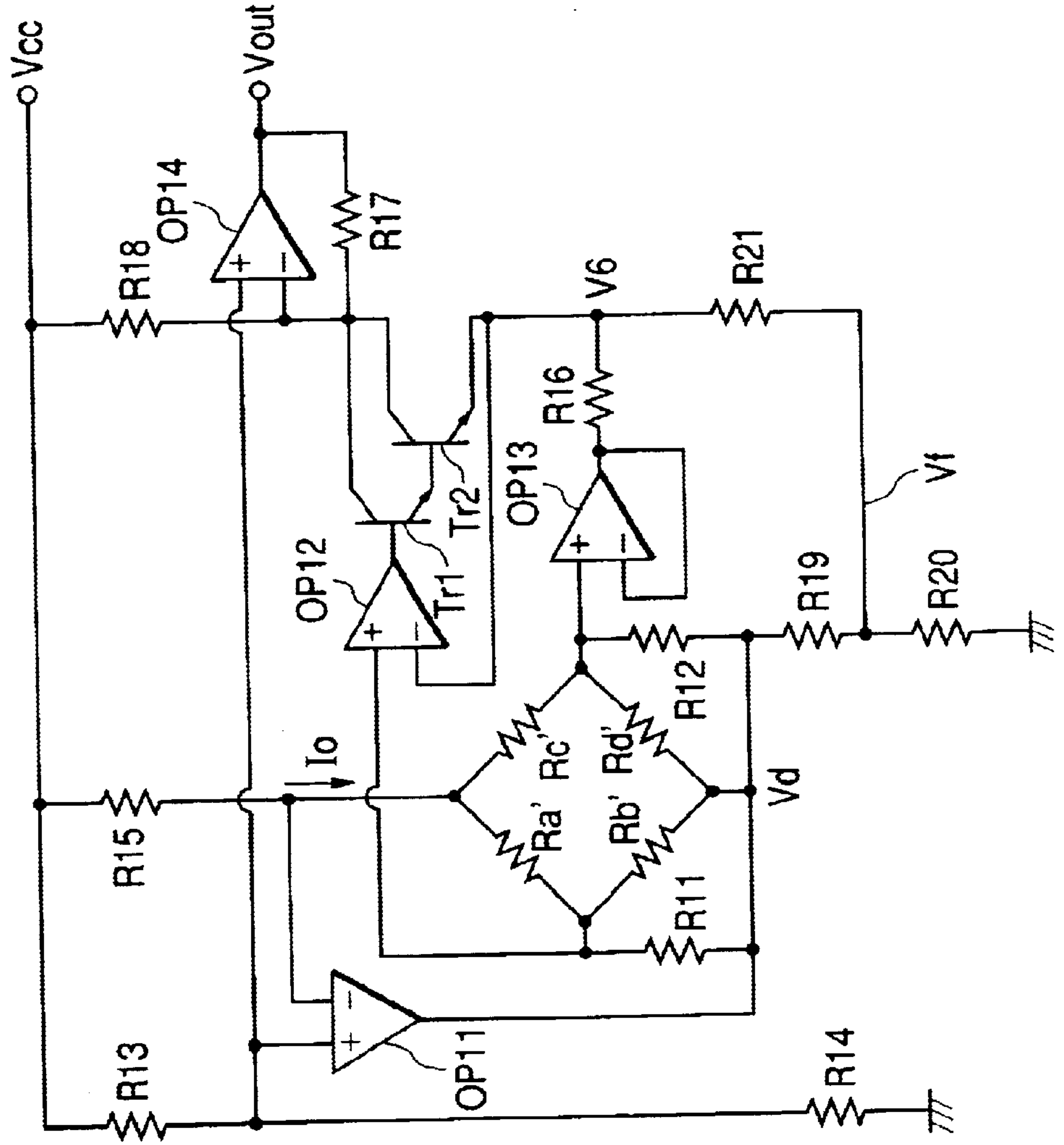
FIG. 5 PRIOR ART
