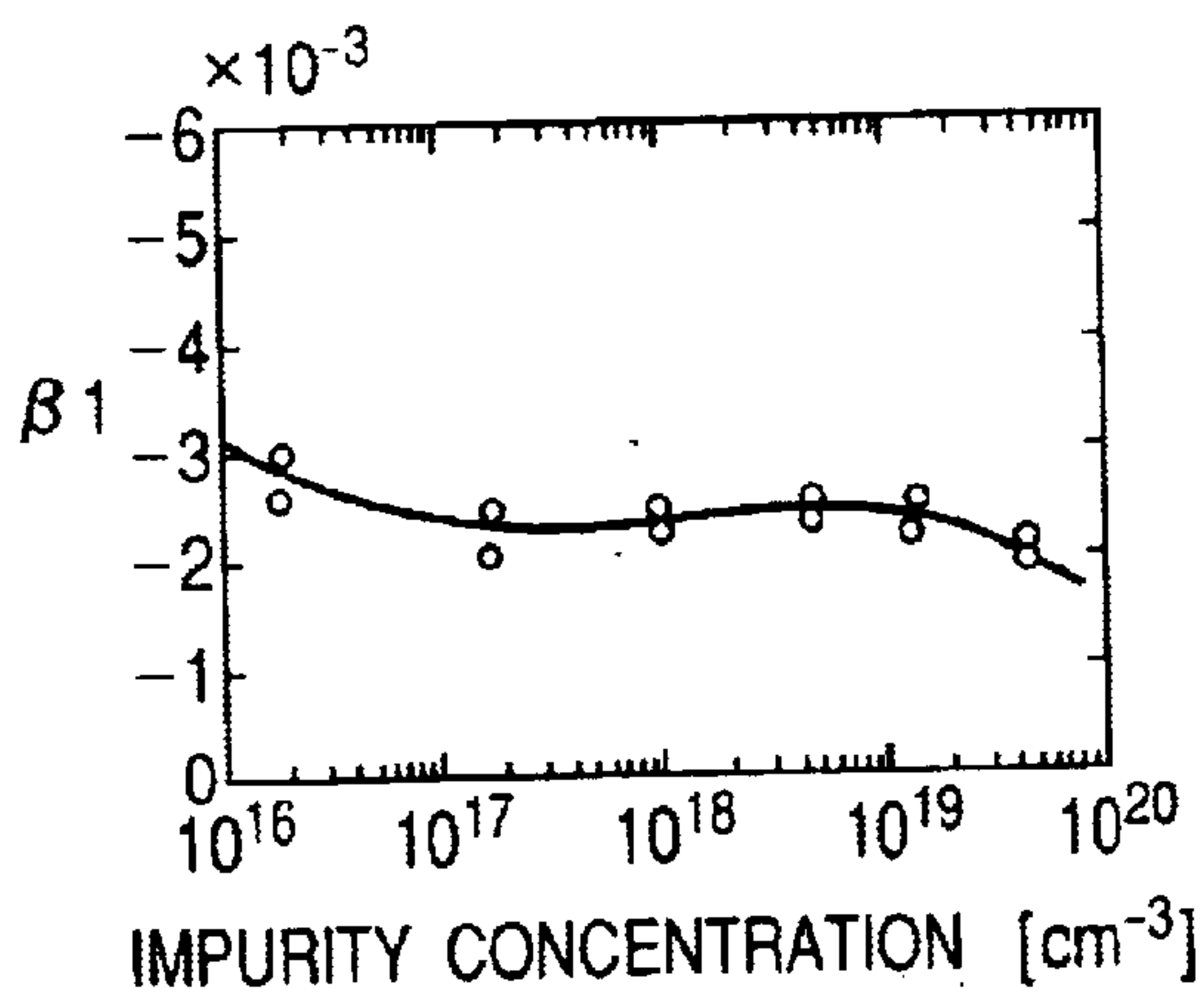
FIG. 3C PRIOR ART
