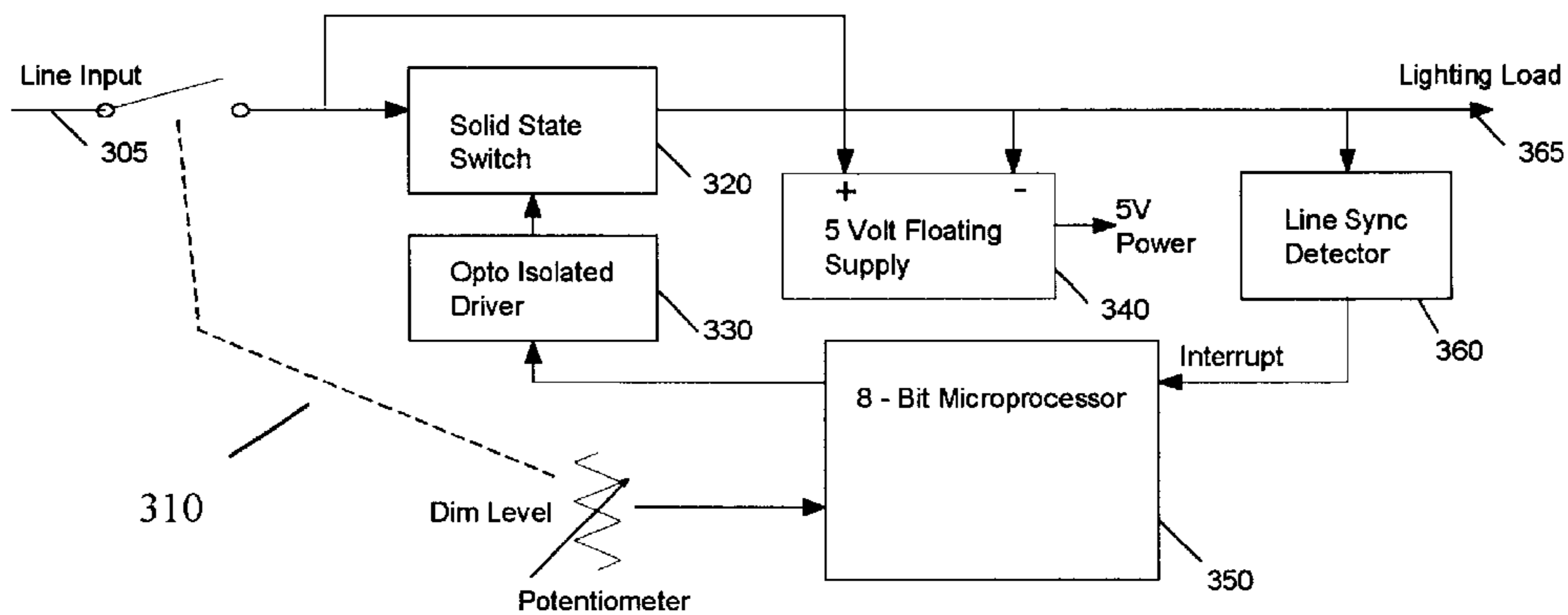
UCD Block Diagram
