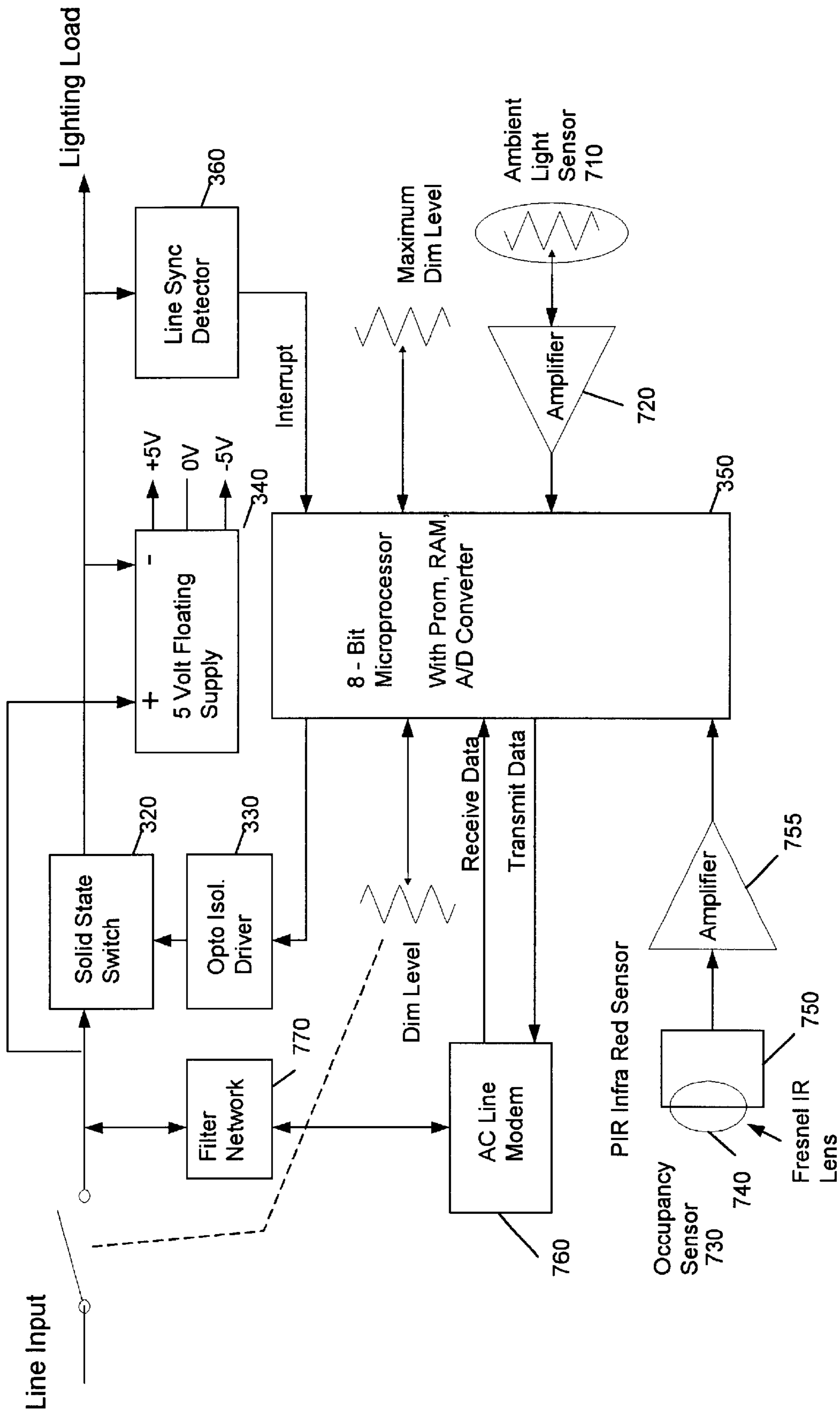
Figure 7: UC-D-2 Block Diagram
