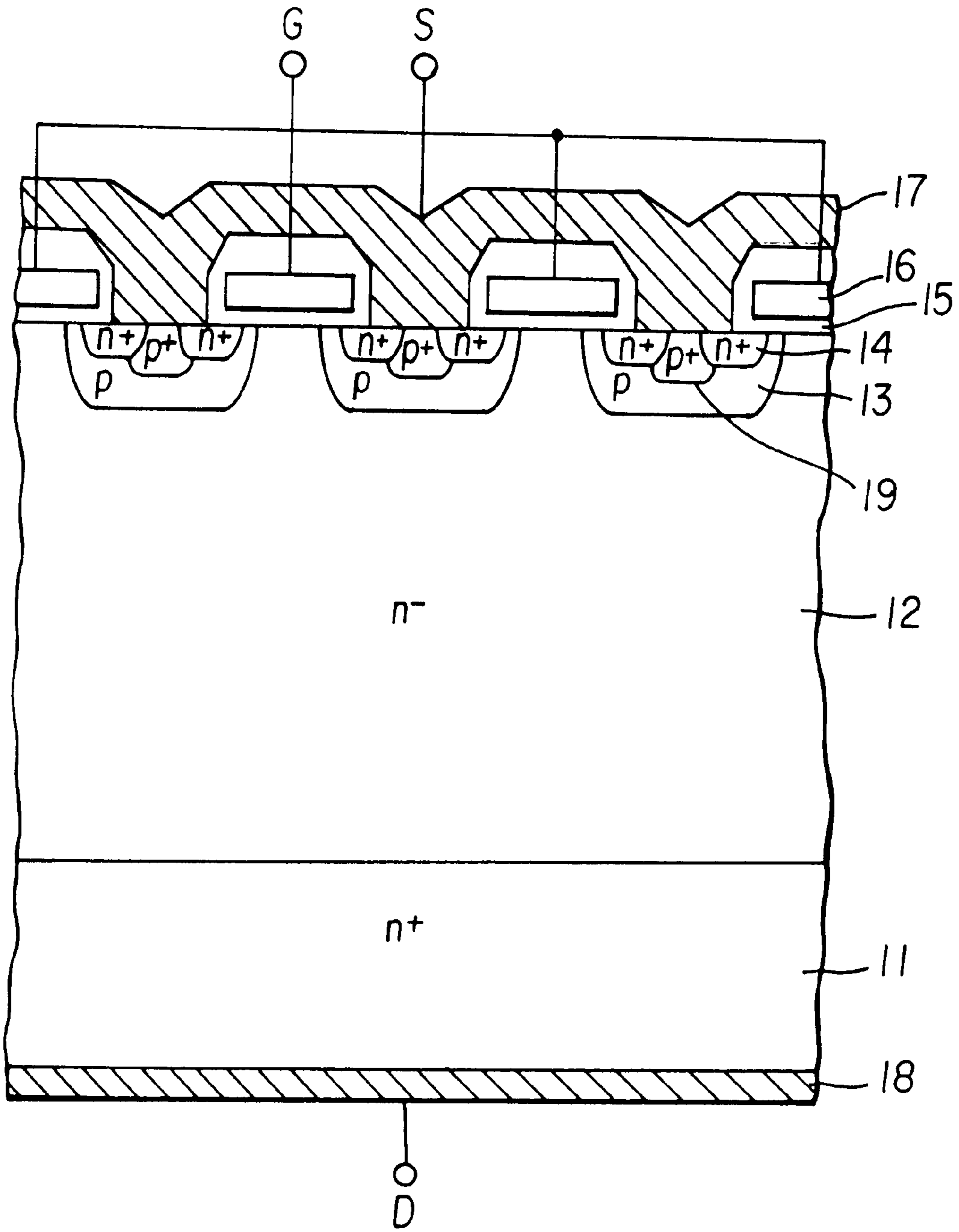
FIG. 28 (PRIOR ART)
