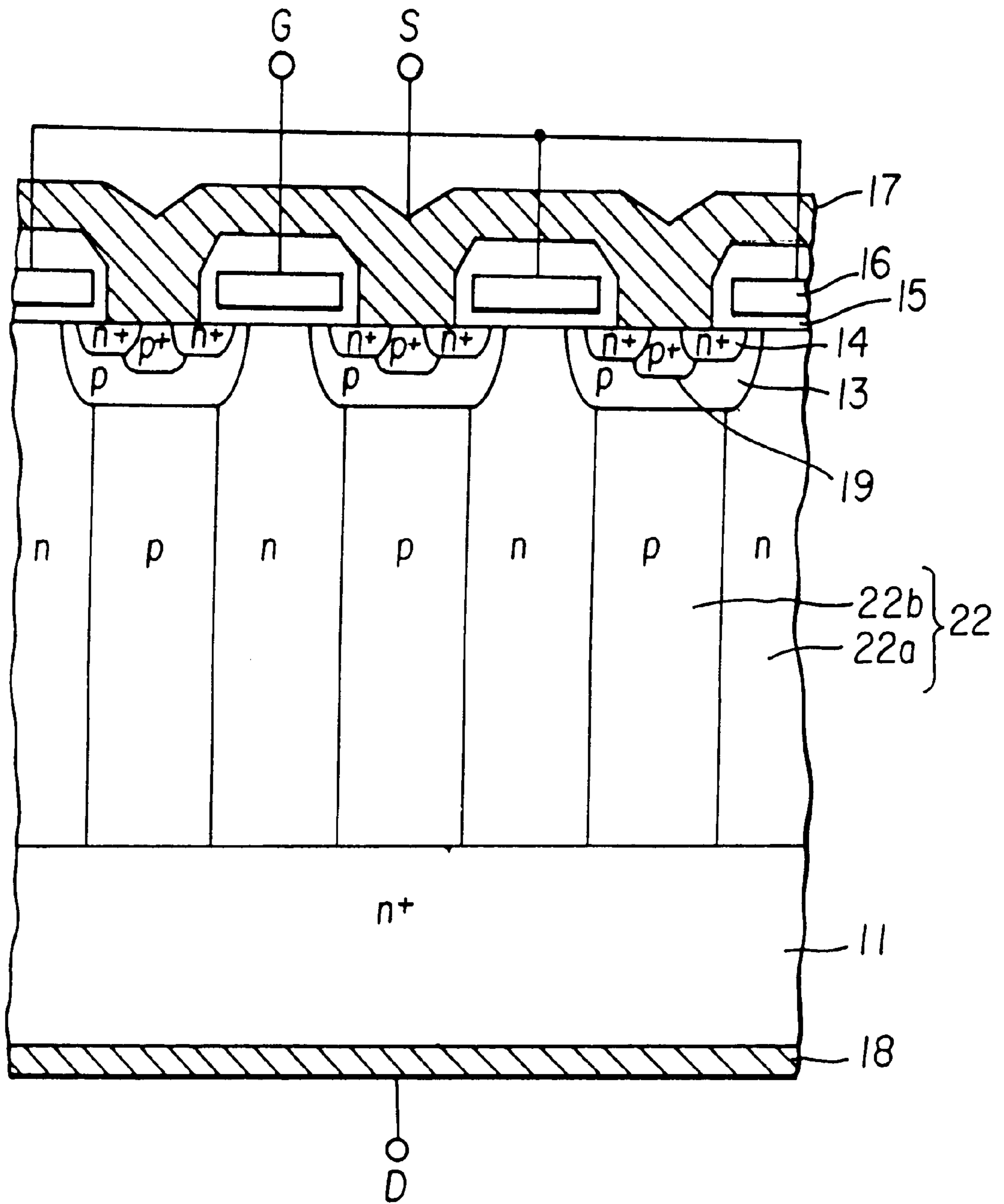
FIG. 29 (PRIOR ART)
