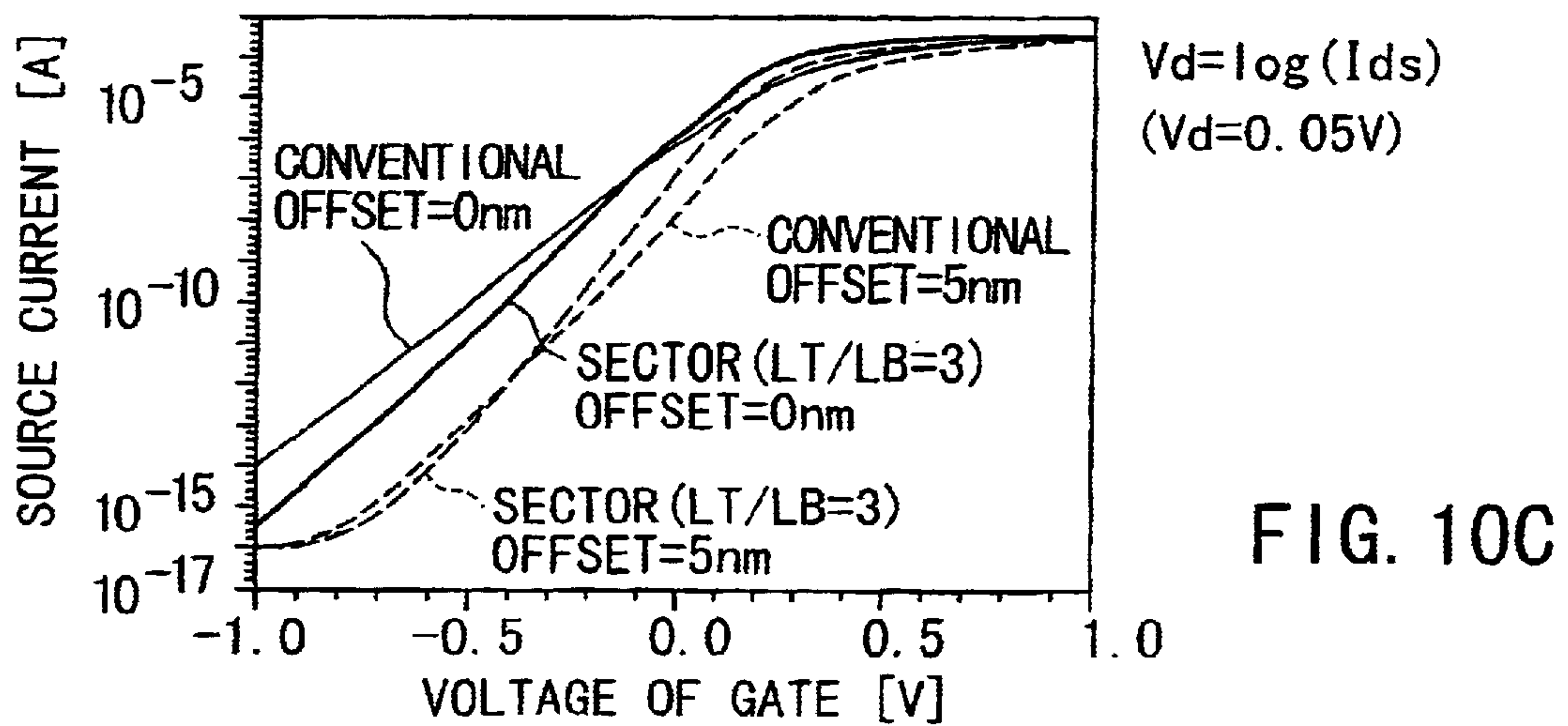
OFFSET DEPENDENCY OF V_g = I_{ds} CHARACTERISTIC ( T_{ef} = 3.0\text{nm}(\text{TiO}_2) , T = 60\text{nm} , LB = 50\text{nm} , \epsilon_r = 80 )
