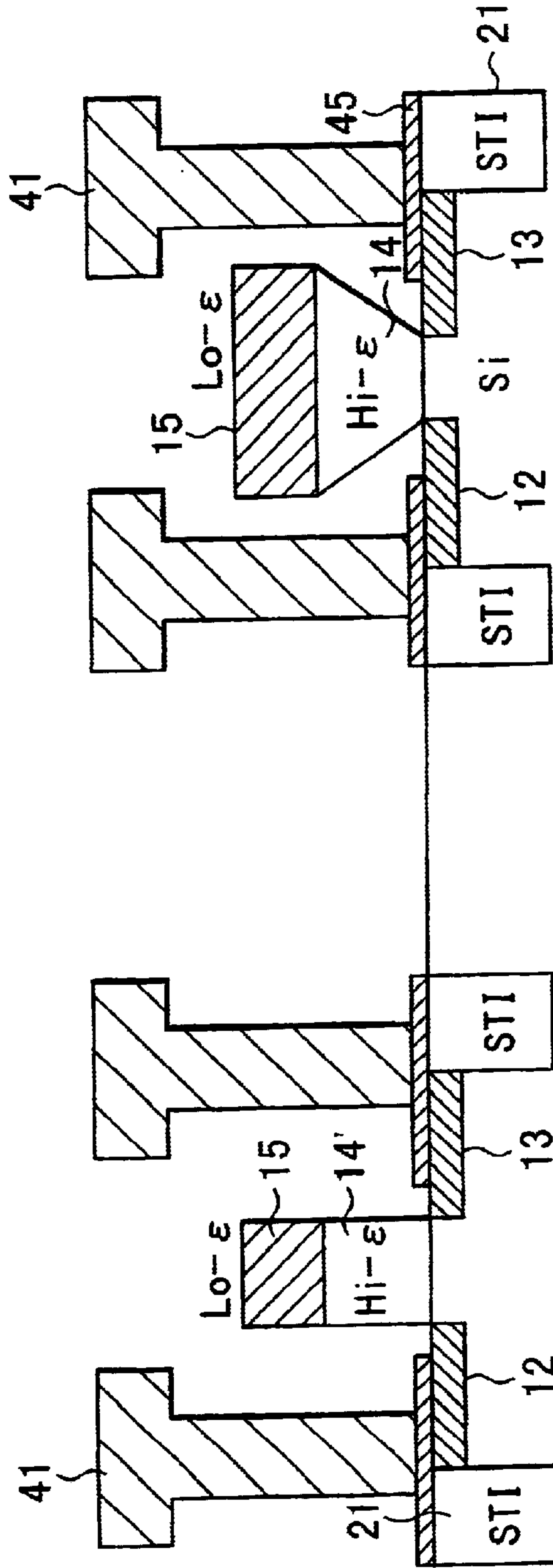
PERIPHERAL CIRCUIT SECTION
