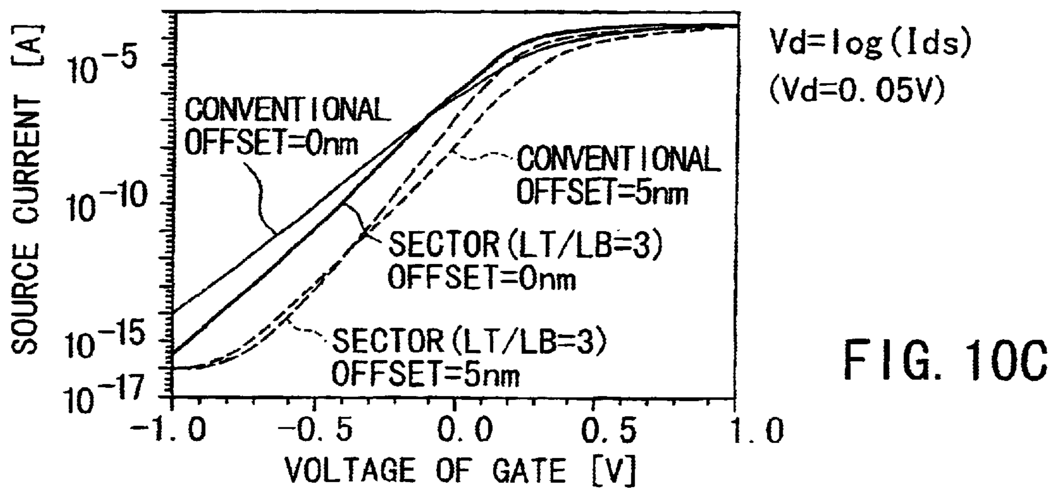
OFFSET DEPENDENCY OF V_g = I_{ds} CHARACTERISTIC ( T_{ef} = 3.0\text{nm (TiO}_2\text{)} , T = 60\text{nm} , LB = 50\text{nm} , \epsilon_r = 80 )
