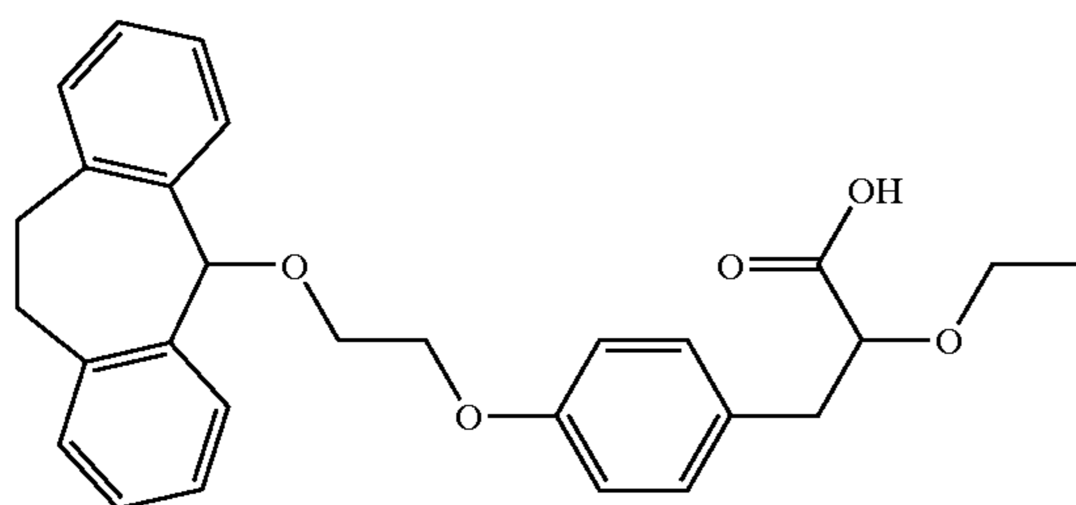
3-(4-[2-(10,11-Dihydro-5H-dibenzo[a,d]cyclohepten-5-yloxy)-ethoxy]-phenyl)-2-ethoxypropanoic acid
