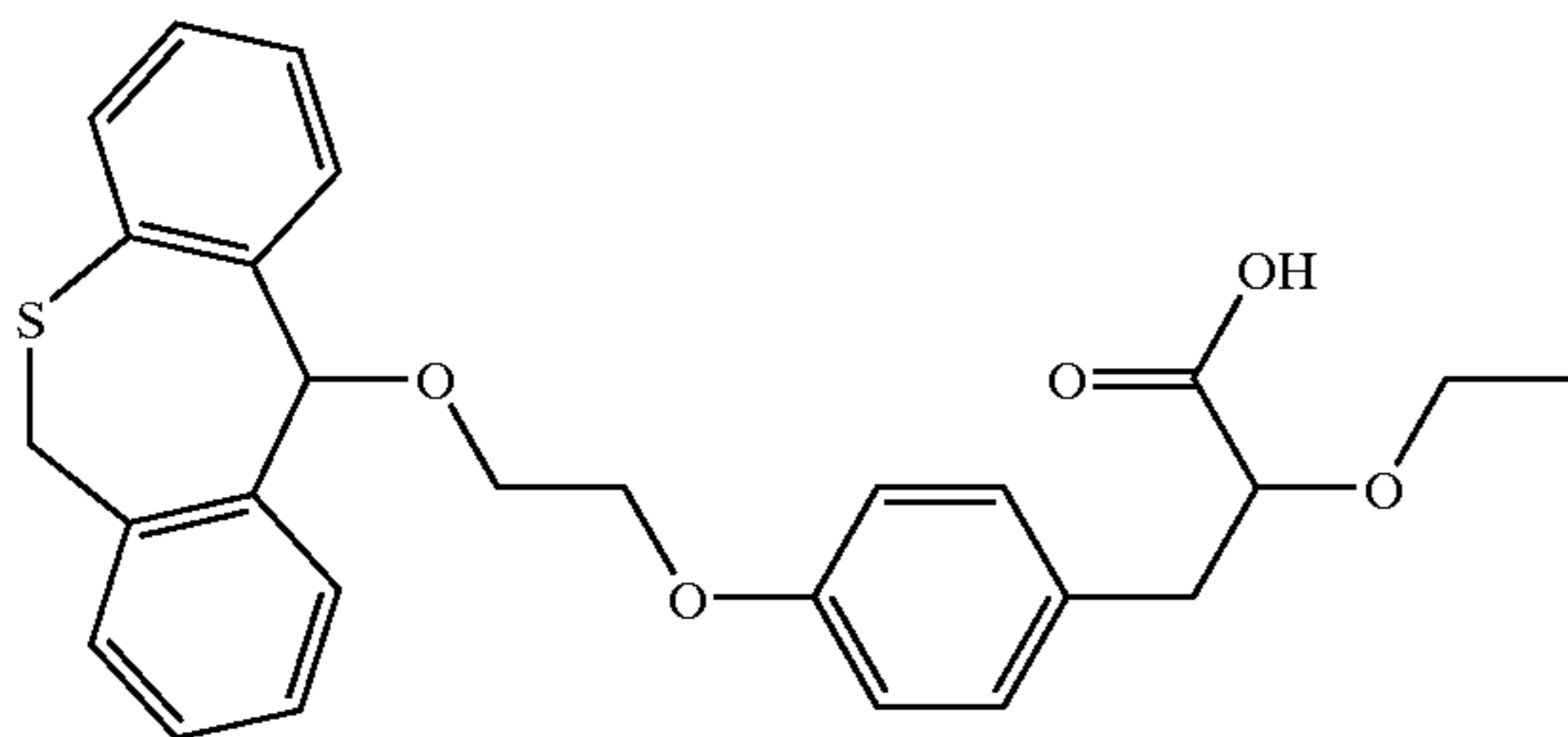
3-(4-[2-(6,11-Dihydrodibenzo[b,e]thiepin-11-yloxy)-ethoxy]-phenyl)-2-ethoxy-propionic acid
