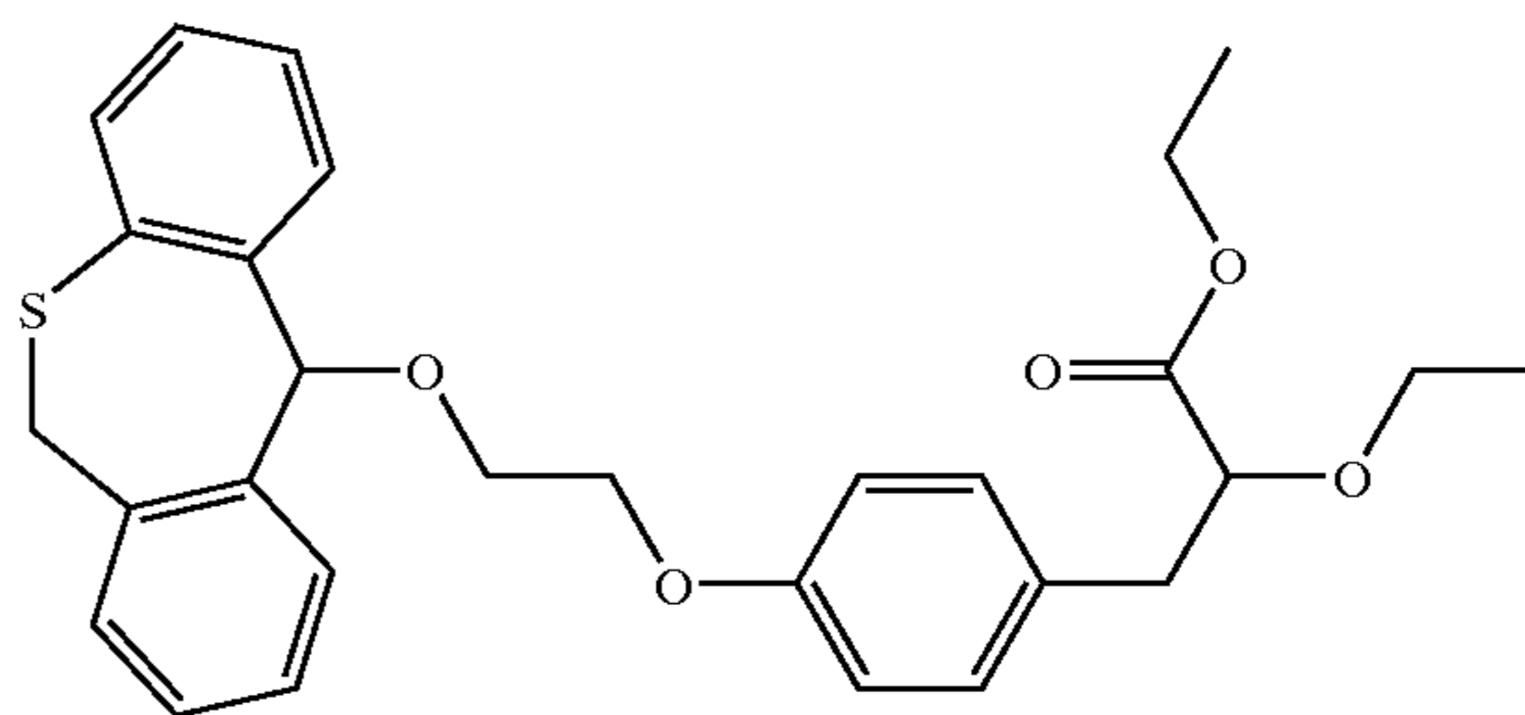
3-(4-[2-(6,11-Dihydrodibenzo[b,e]thiepin-11-yloxy)-ethoxy]-phenyl)-2-ethoxy-propionic acid ethyl ester
