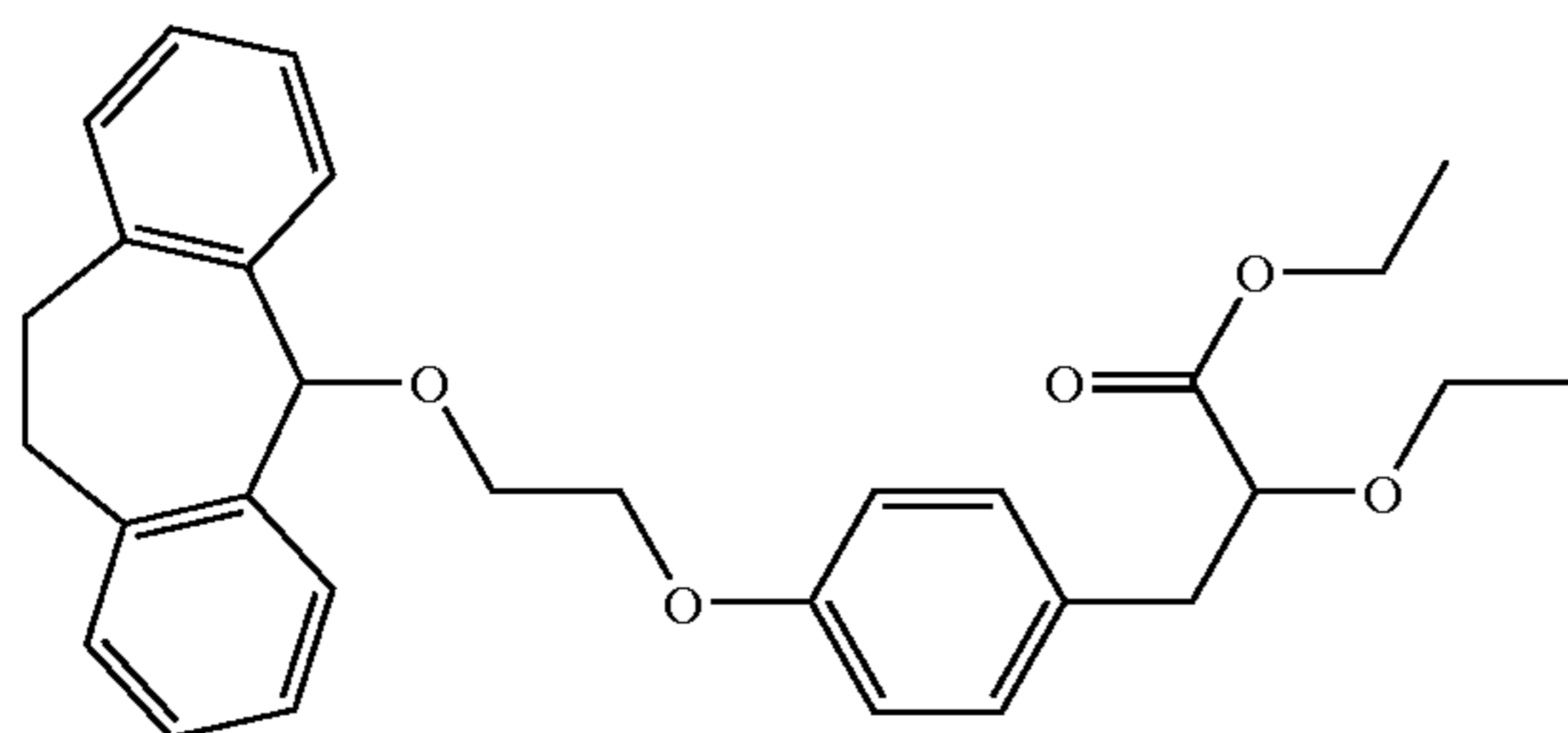
3-(4-[2-(10,11-Dihydro-5H-dibenzo[a,d]cyclohepten-5-yloxy)-ethoxy]-phenyl)-2-ethoxypropanoic acid ethyl ester
