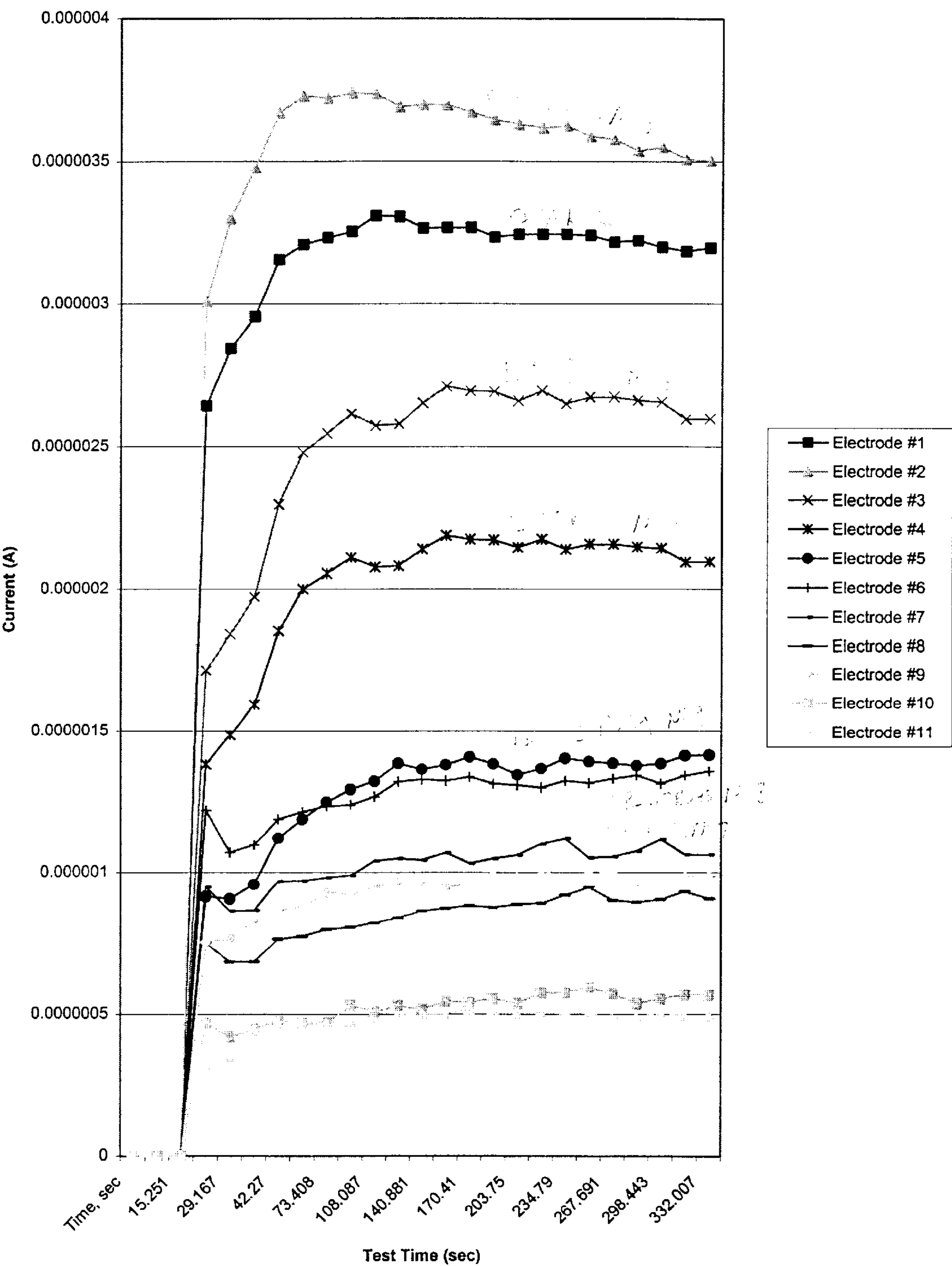
Fig. 3 Methanol Oxidation Currents of Electroplated Alloy Compositions -0.3 V vs. NHE
