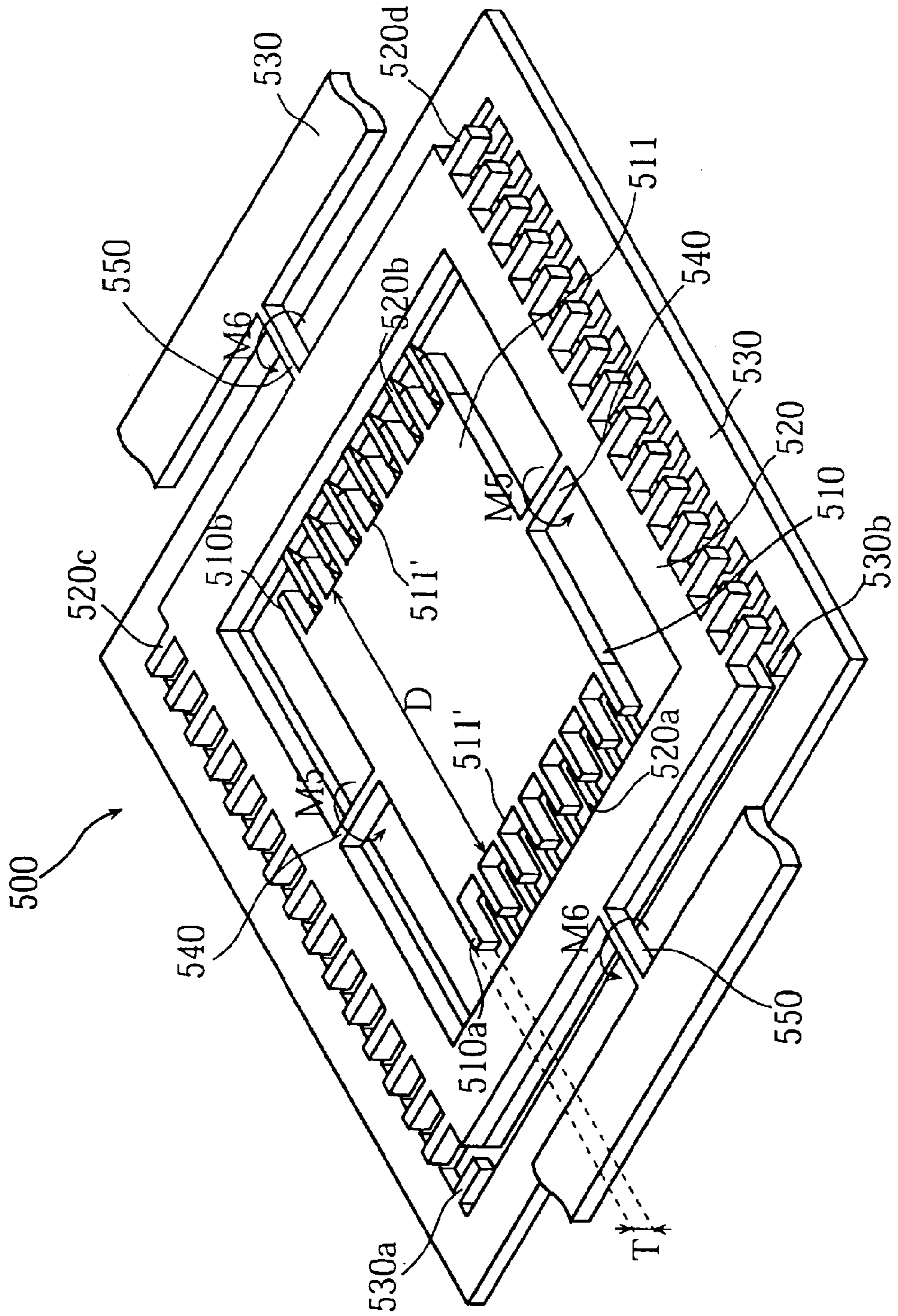
FIG. 43 PRIOR ART
