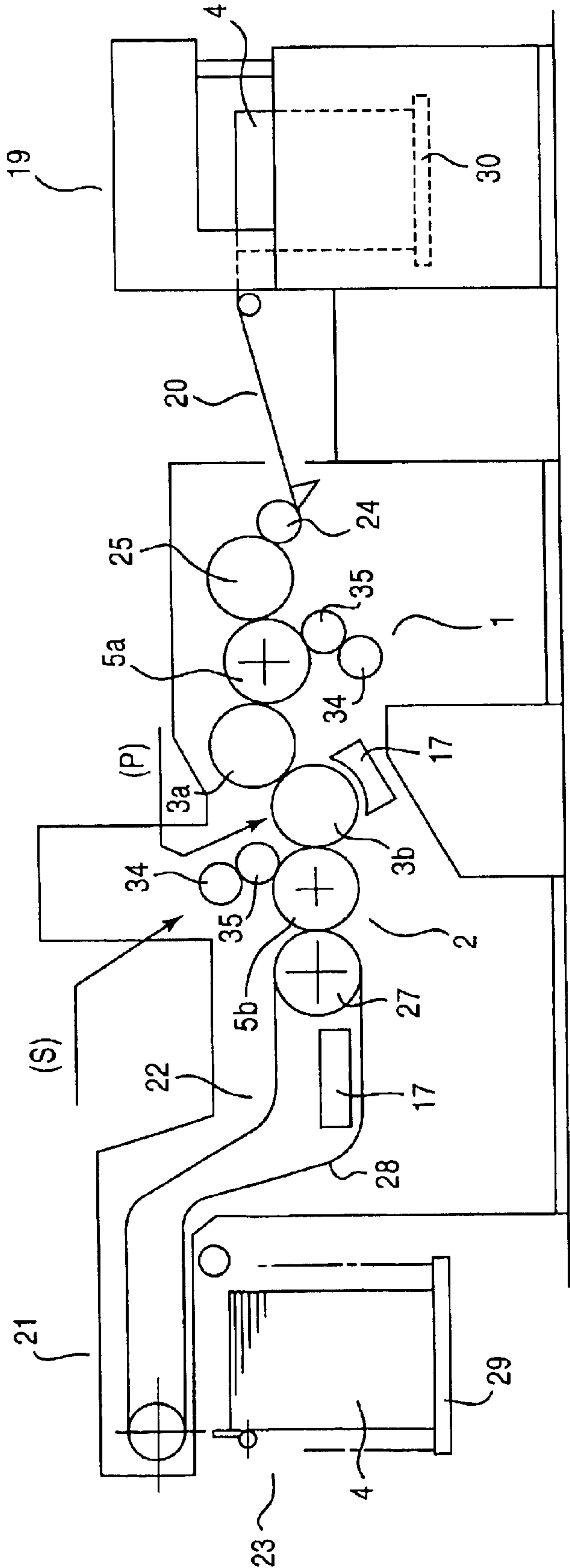
FIG. 9 PRIOR ART
