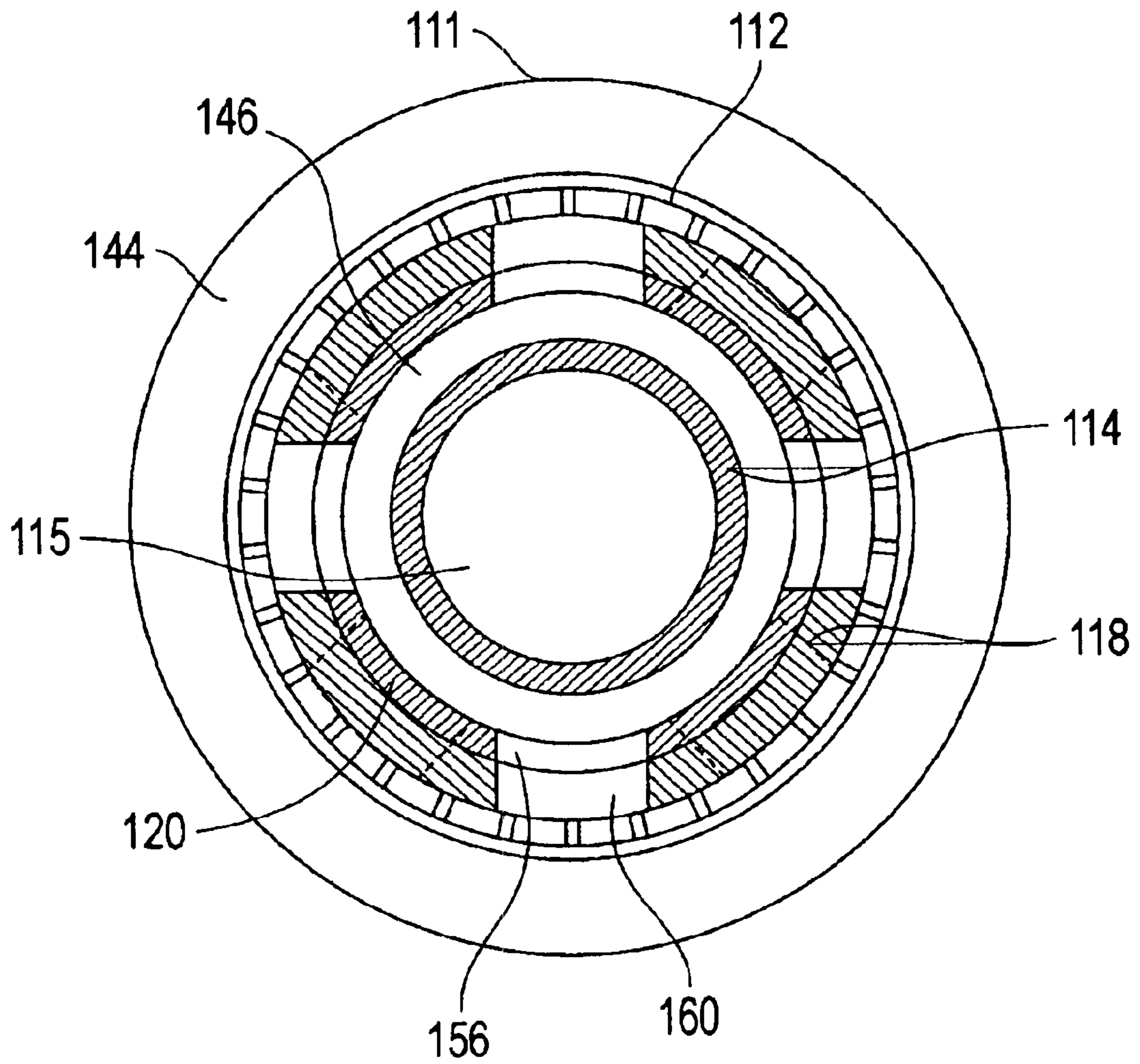
SECTION 'A-A'
