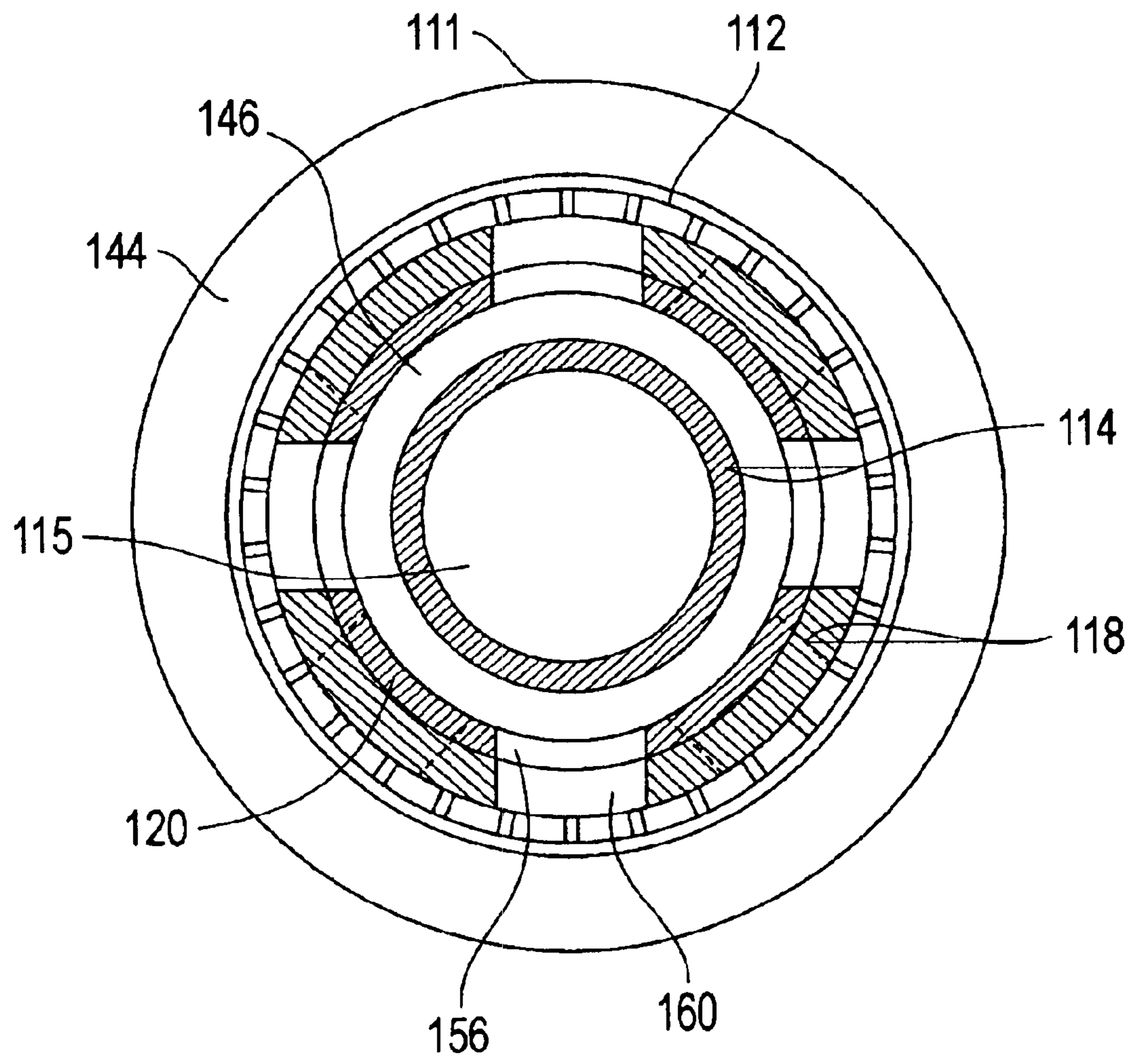
SECTION 'A-A'
