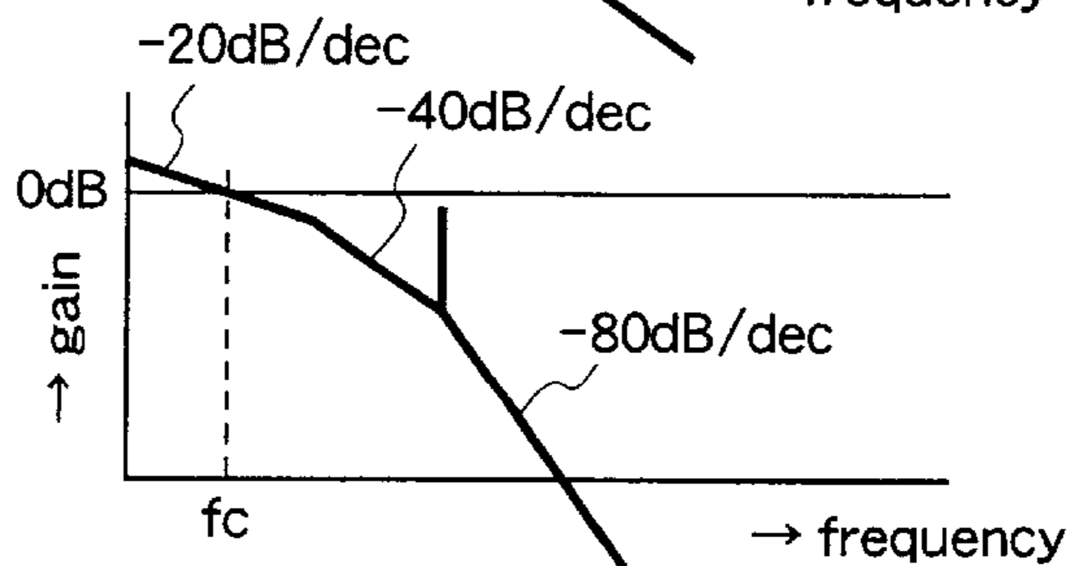
Fig.18 (e) open-loop characteristics of whole changed spot position control
