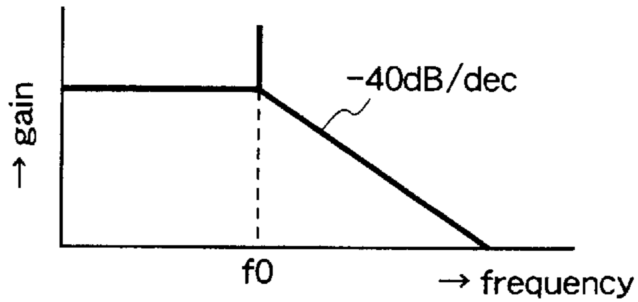
Fig.18 (a) open-loop gain characteristics without spot position loop filter 111
