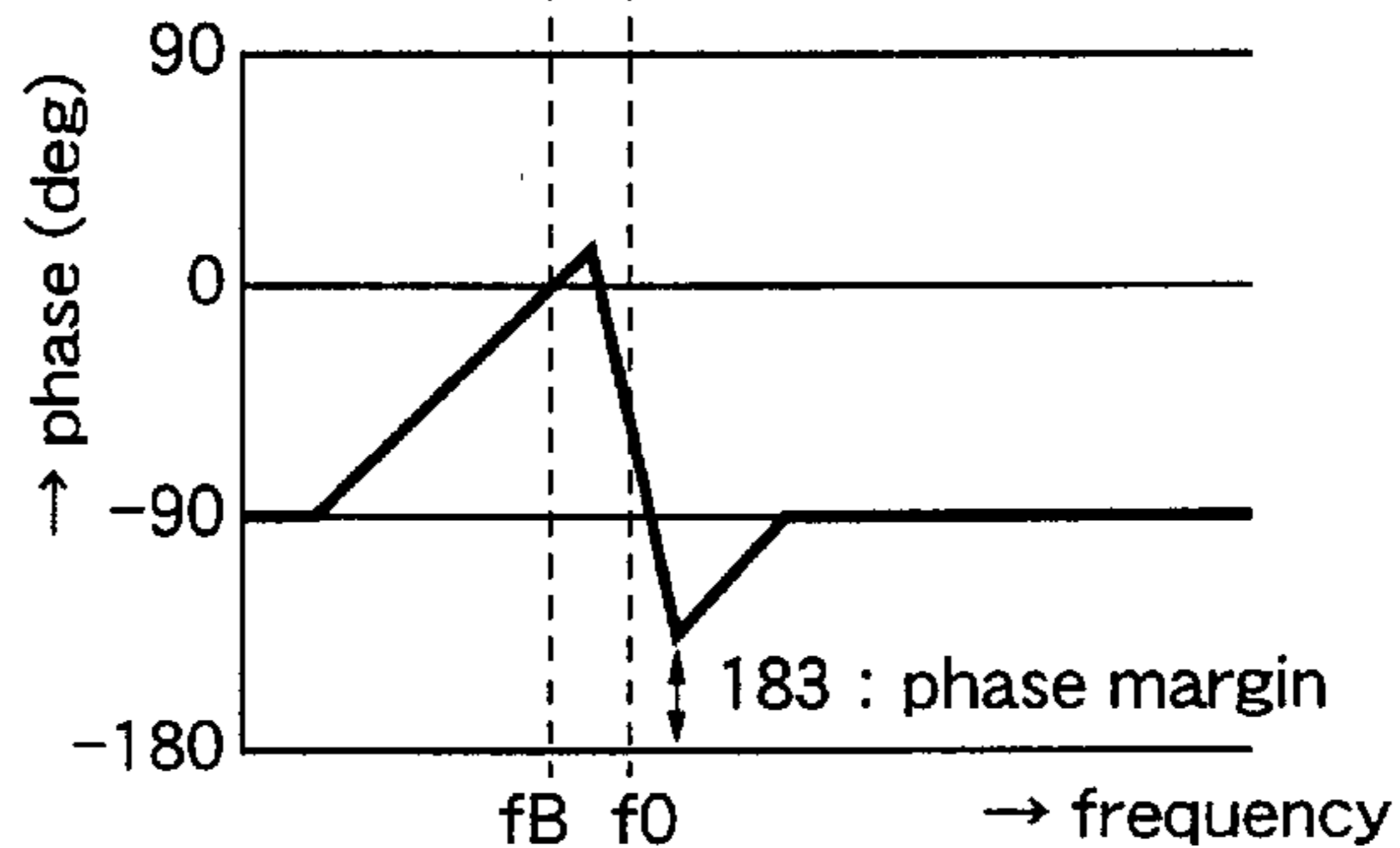
Fig.20 (e) phase characteristics of whole spot position control
