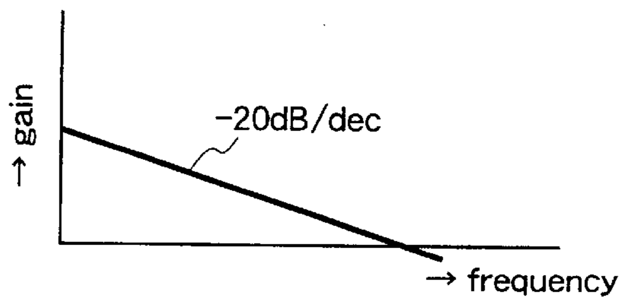
Fig.19 (b) gain characteristics of spot position loop filter 111
