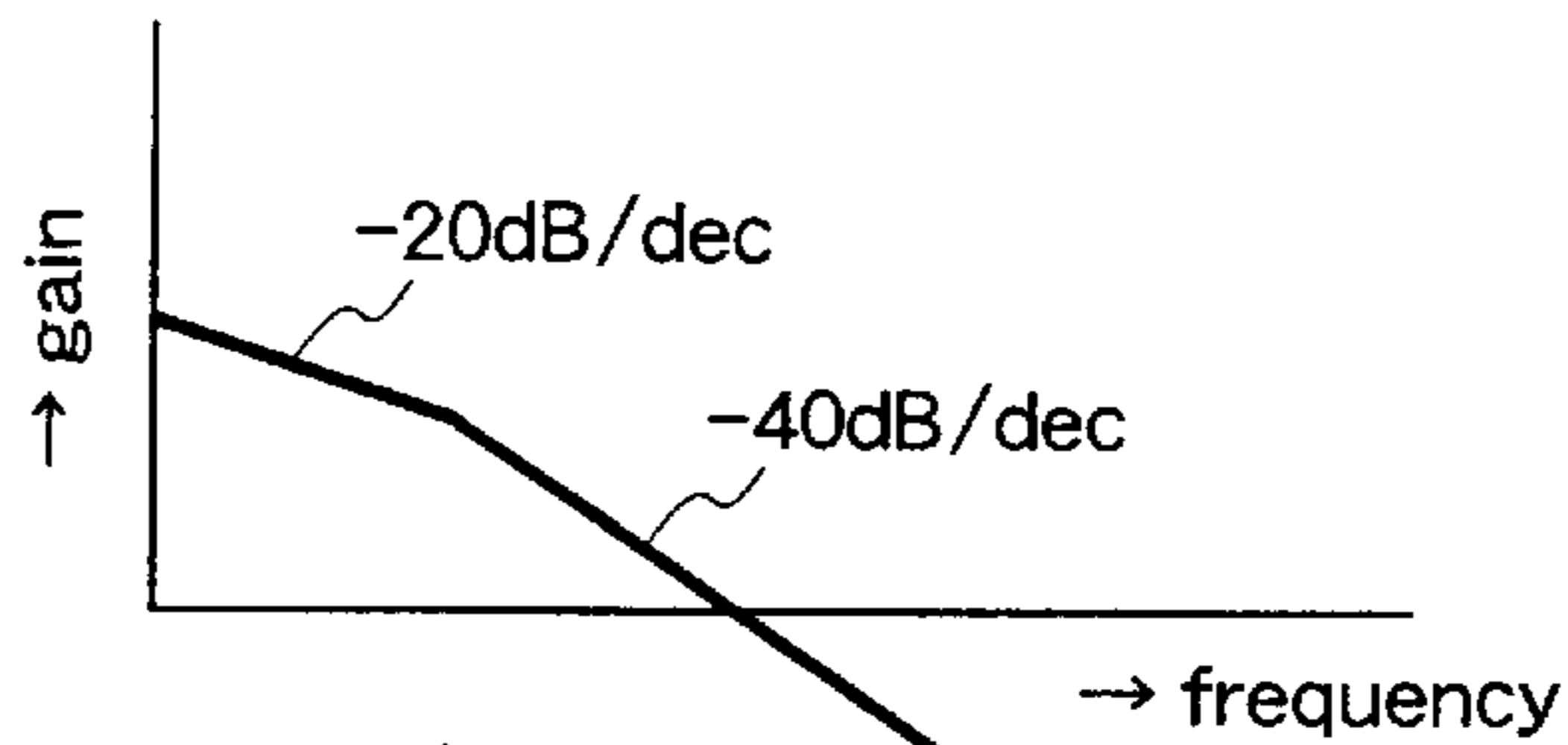
Fig.18 (d) gain characteristics of changed spot position loop filter 111
