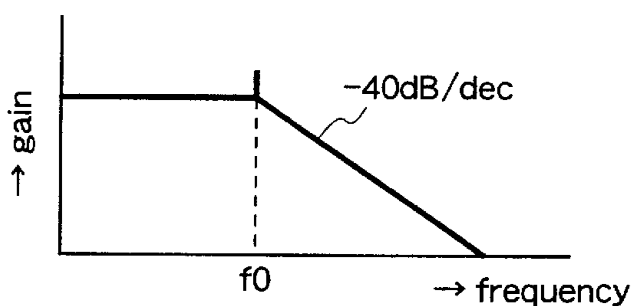
Fig.17 (a) open-loop gain characteristics without spot position loop filter 111
