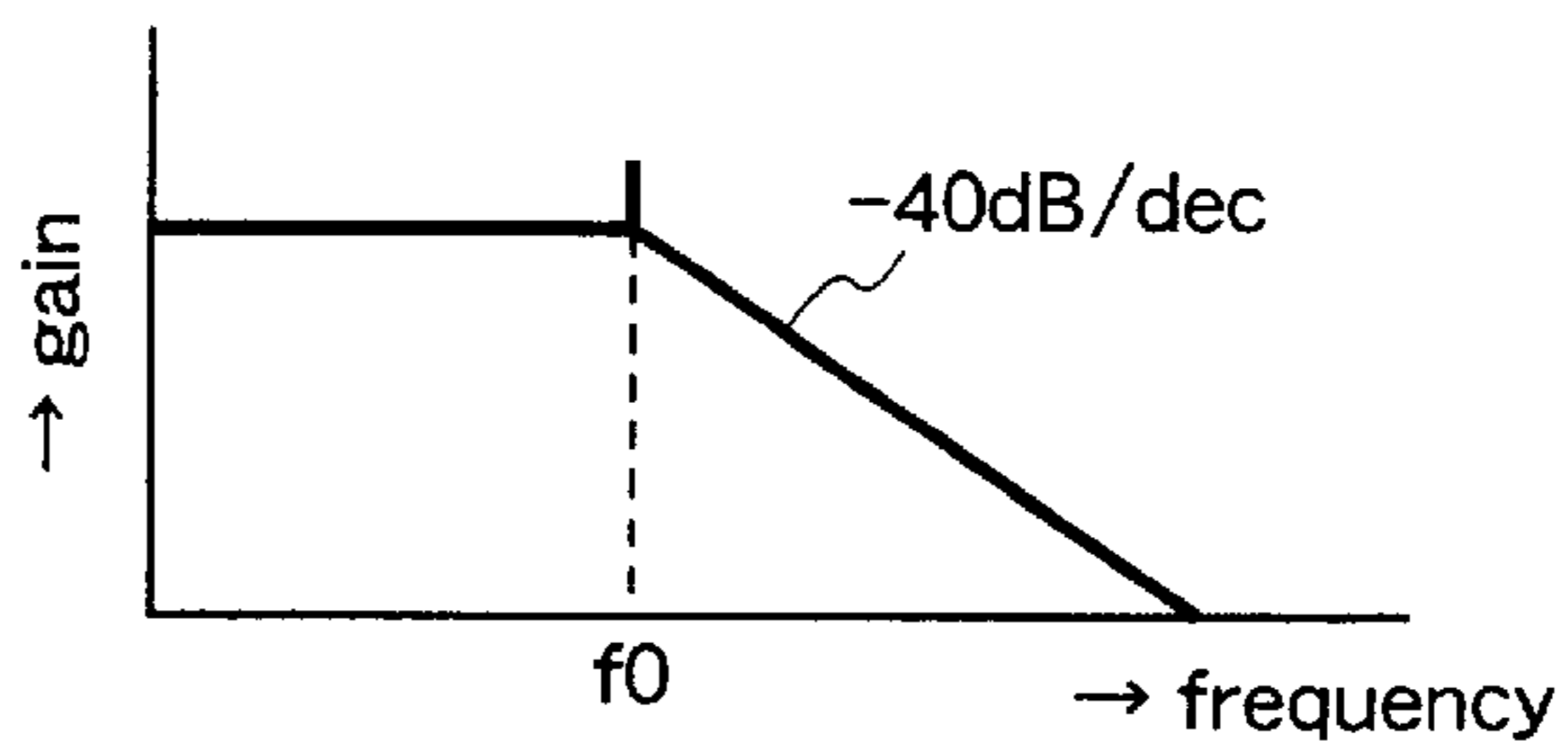
Fig.15 (a) open-loop gain characteristics without spot position loop filter 111
