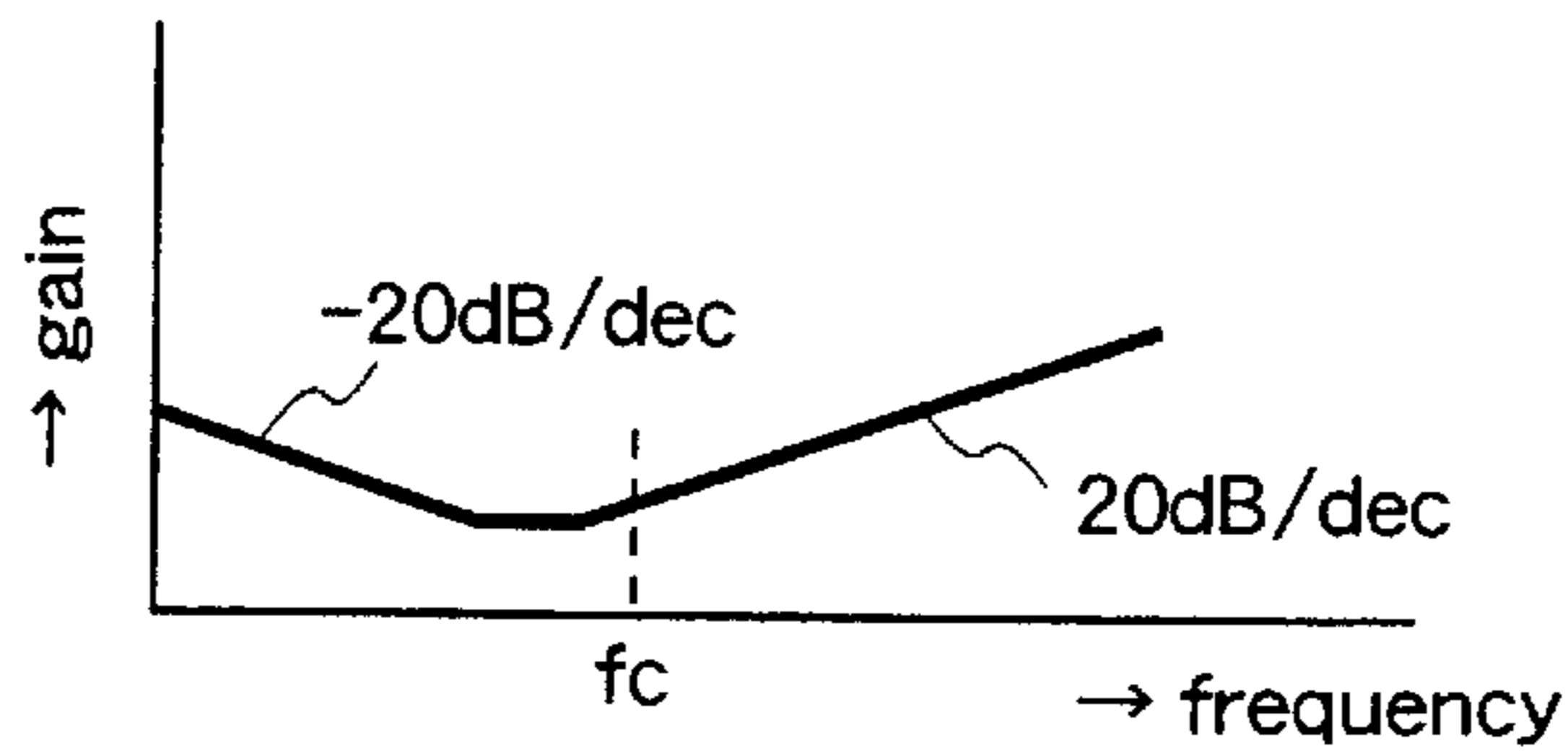
Fig.19 (d) gain characteristics of spot position loop filter 111
