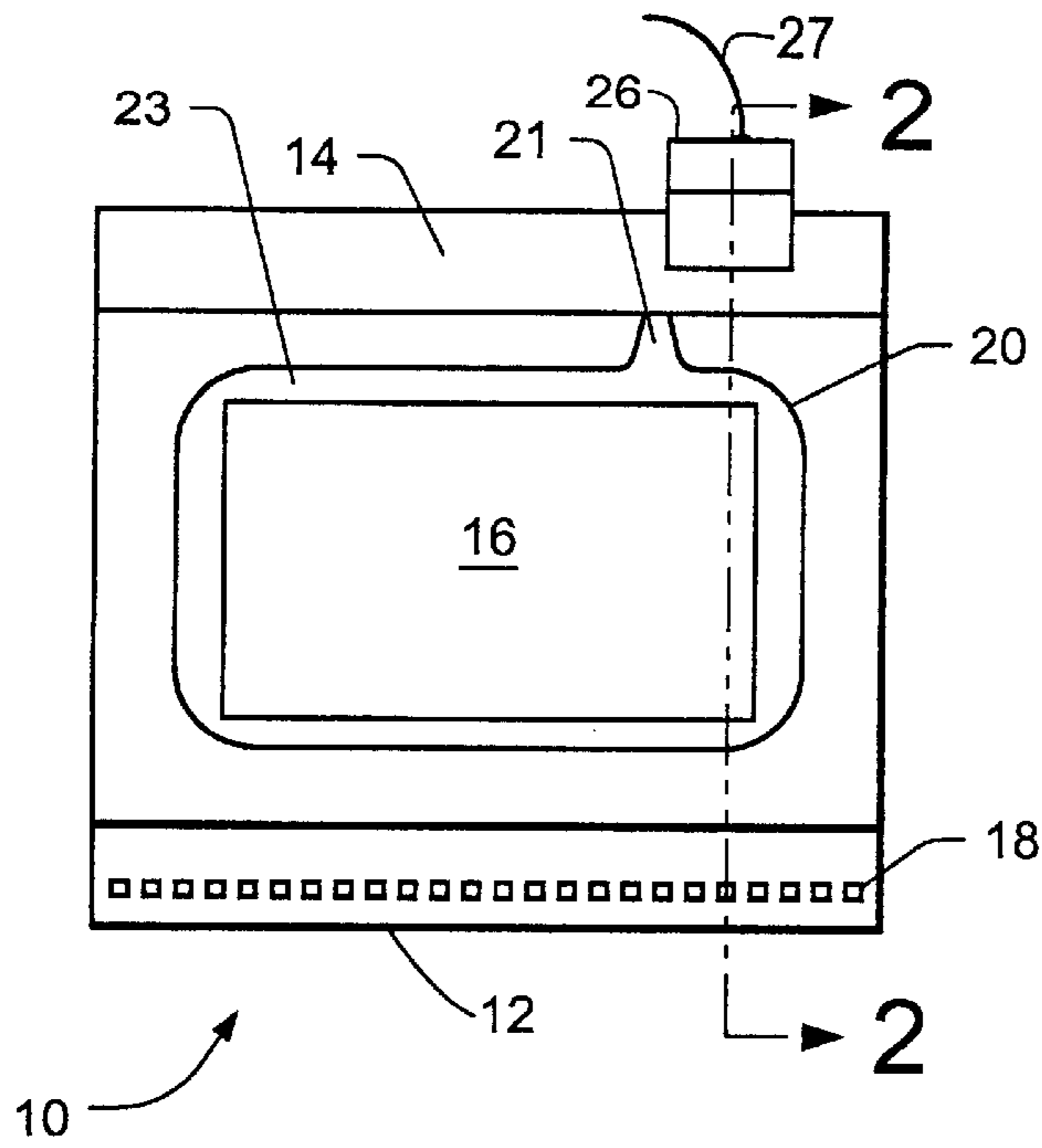
FIG. 1 (PRIOR ART)
