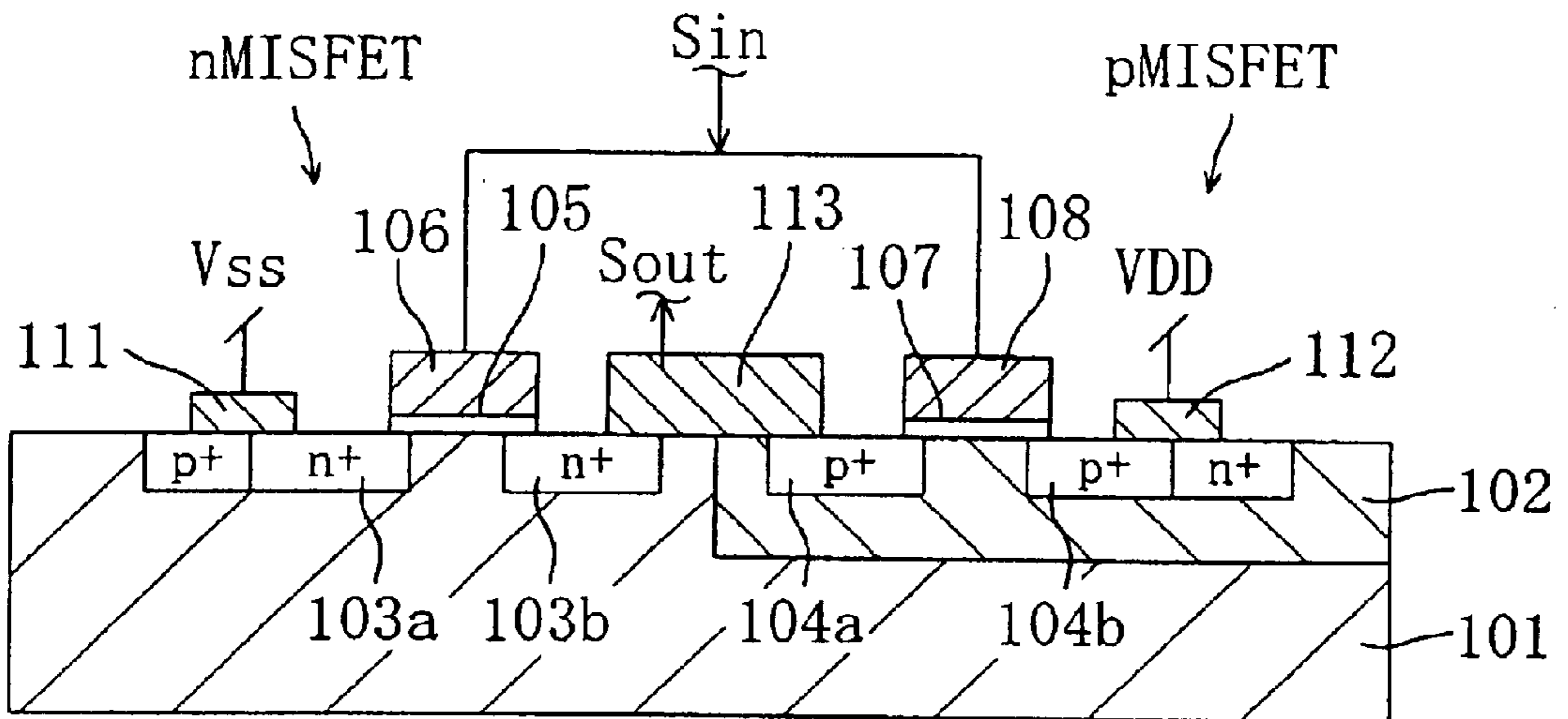
Fig. 13 PRIOR ART
