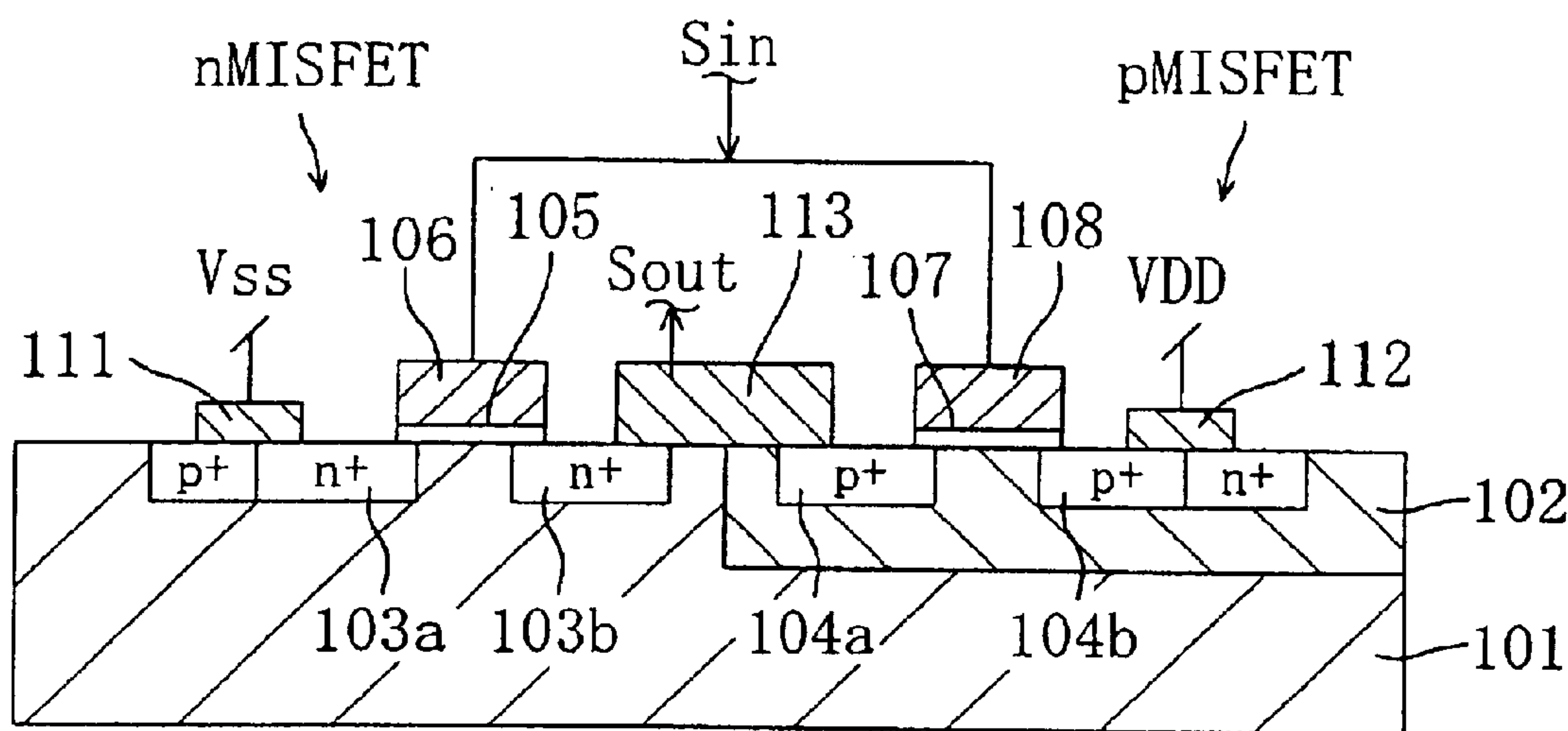
Fig. 13 PRIOR ART
