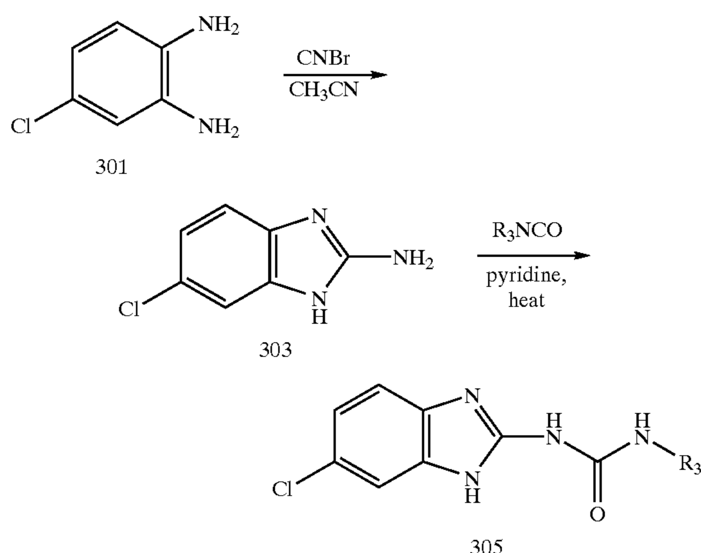
Reaction Scheme 3:
