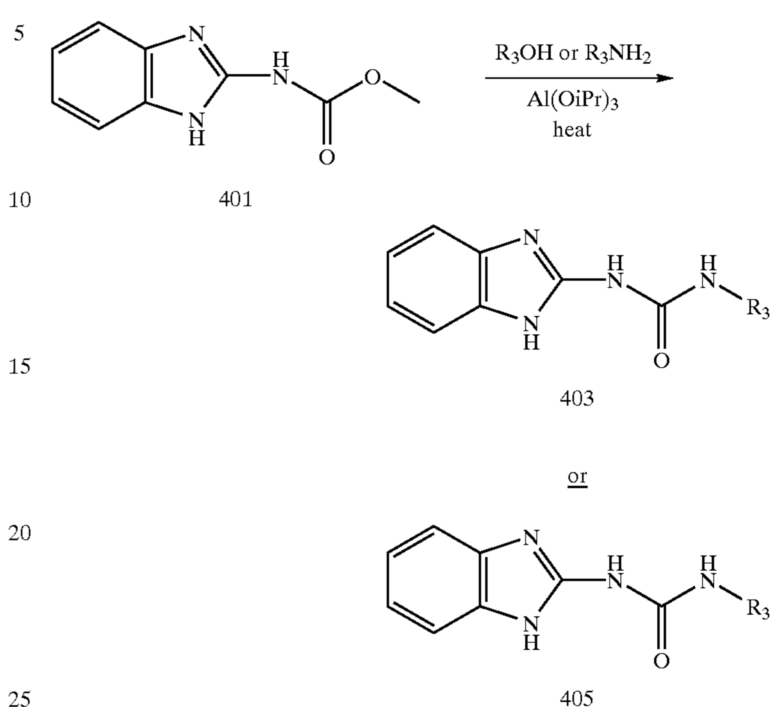
Reaction Scheme 4:
