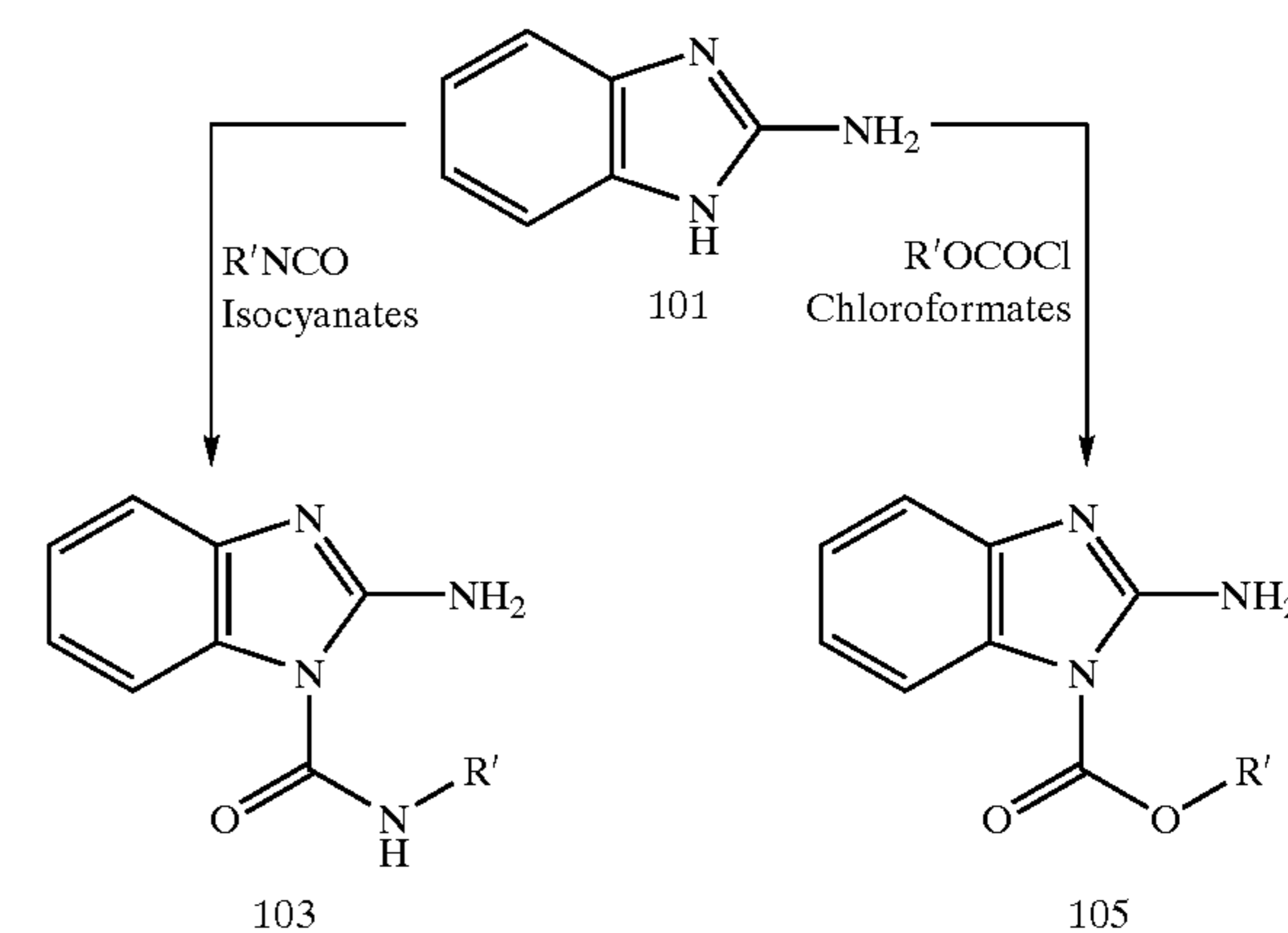
Reaction Scheme 1:
