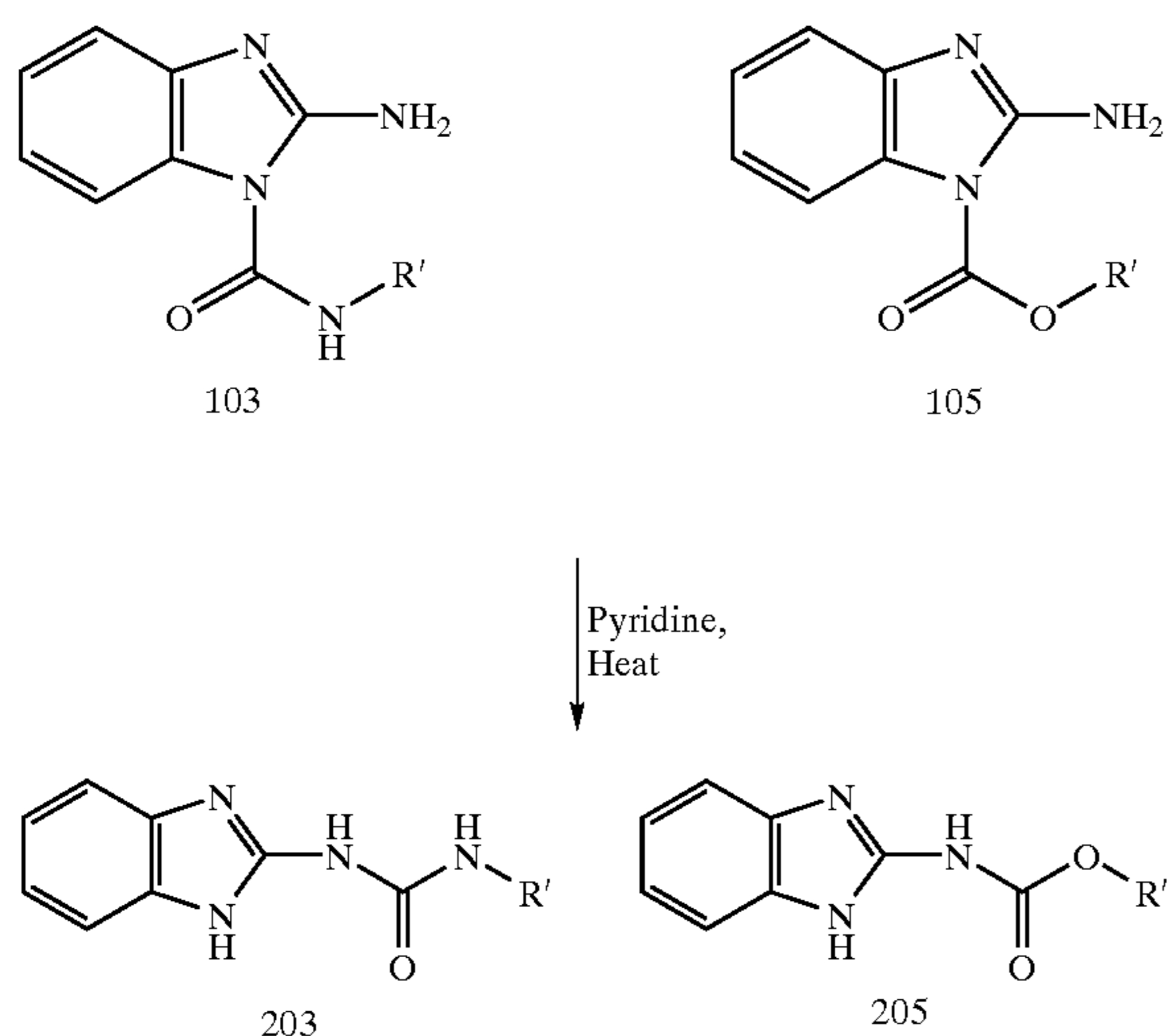
Reaction Scheme 2:
