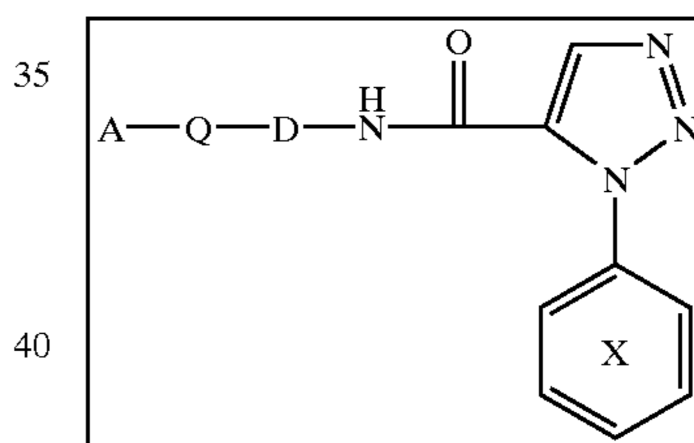
Scheme 3
