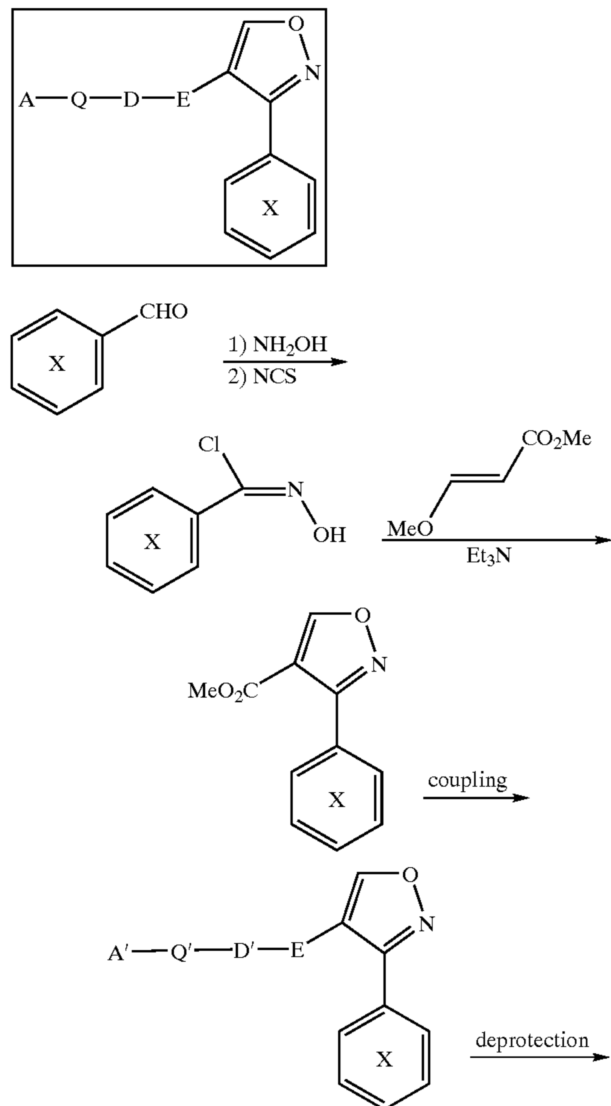
Scheme 6
