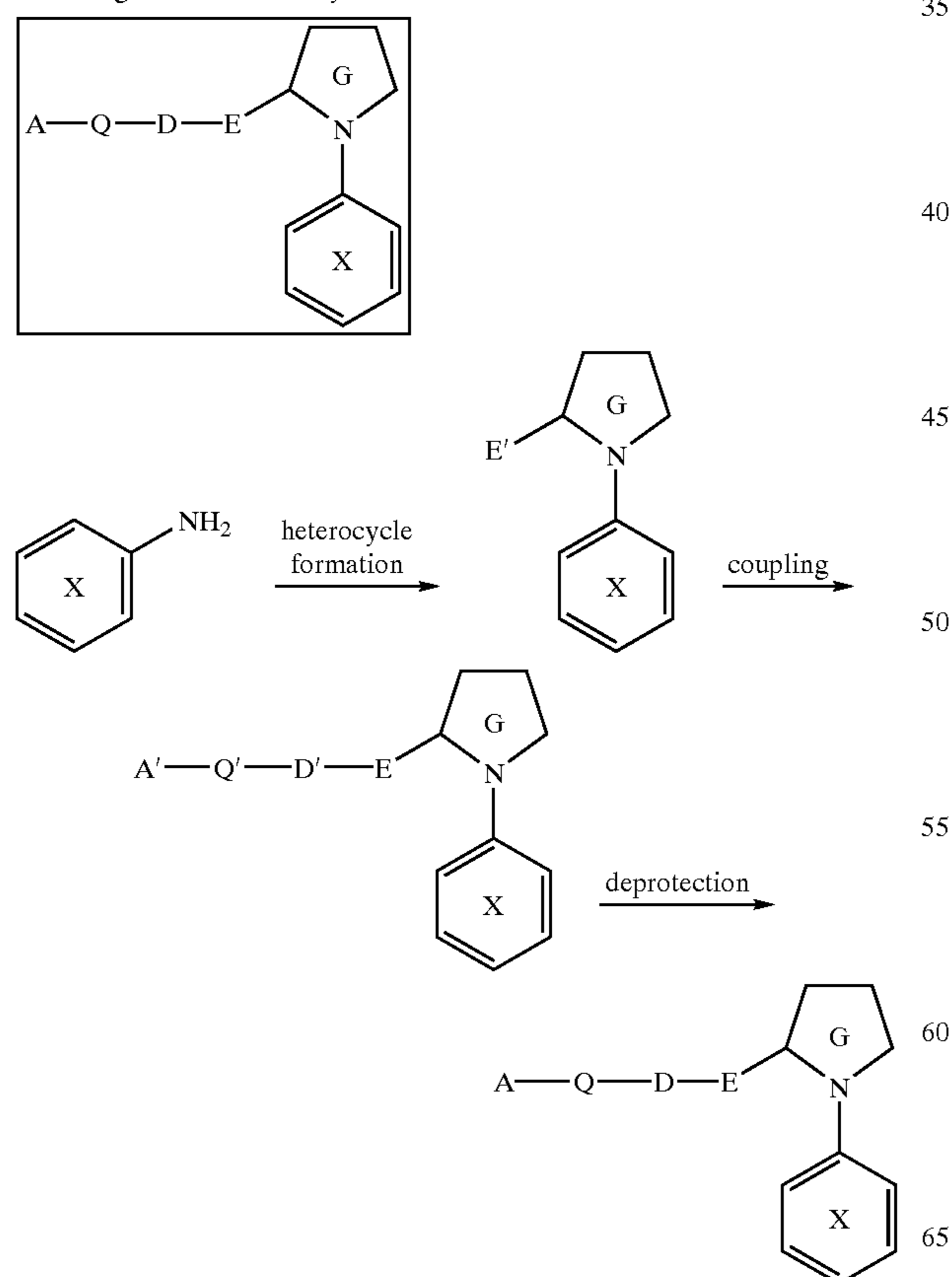
Scheme 1
