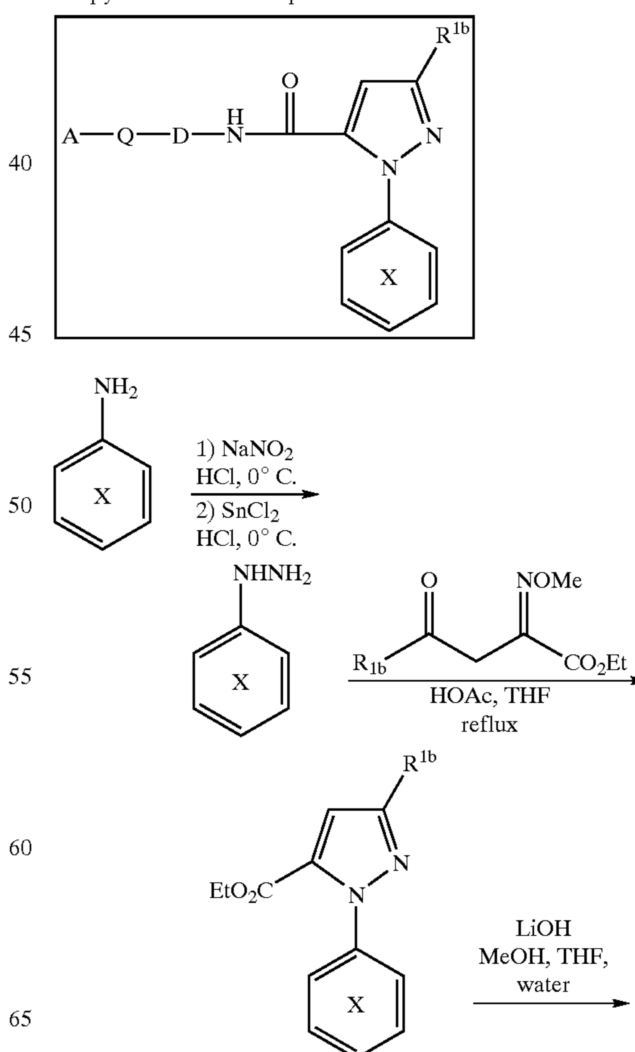
Scheme 2
