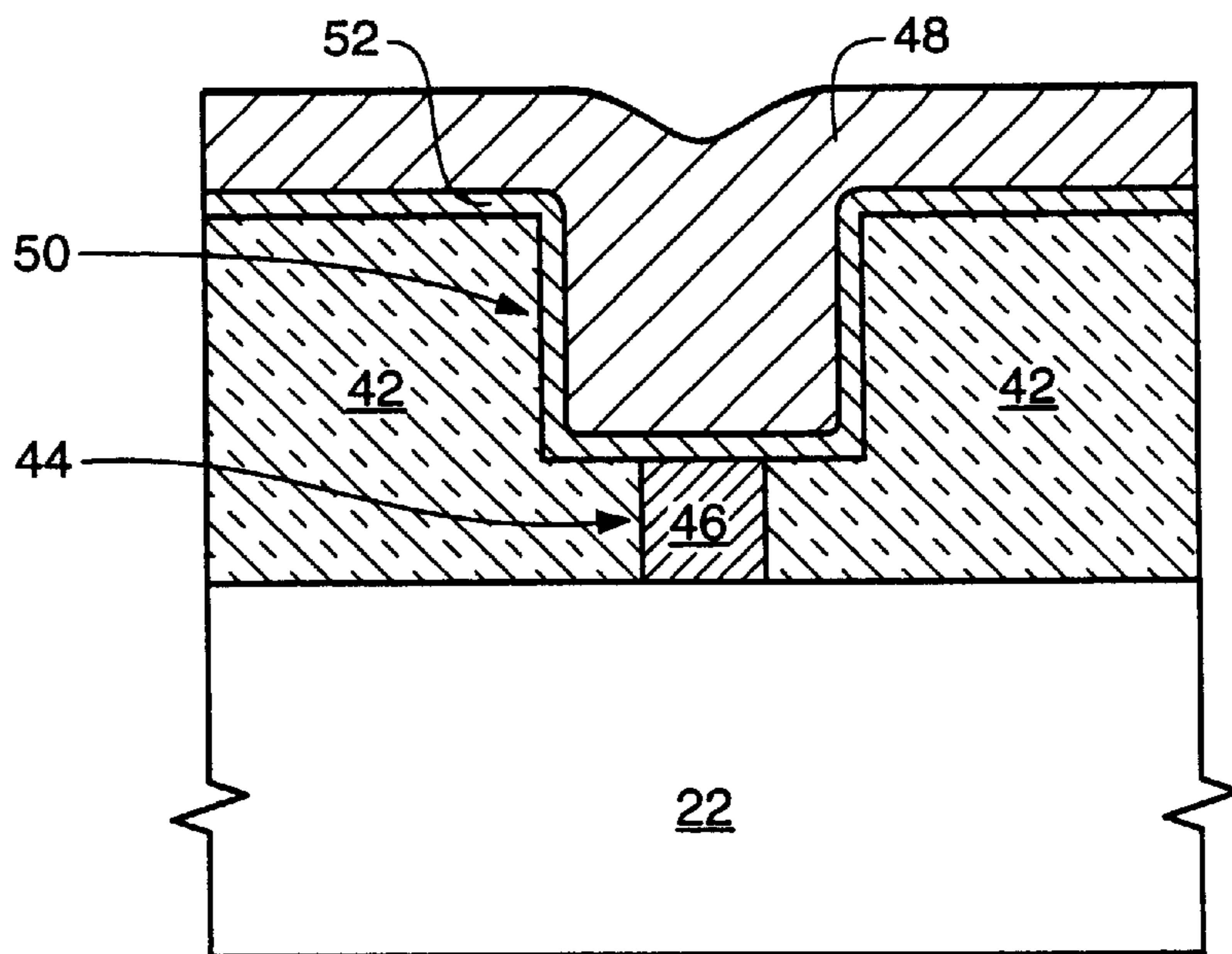
FIG. 7 (PRIOR ART)
