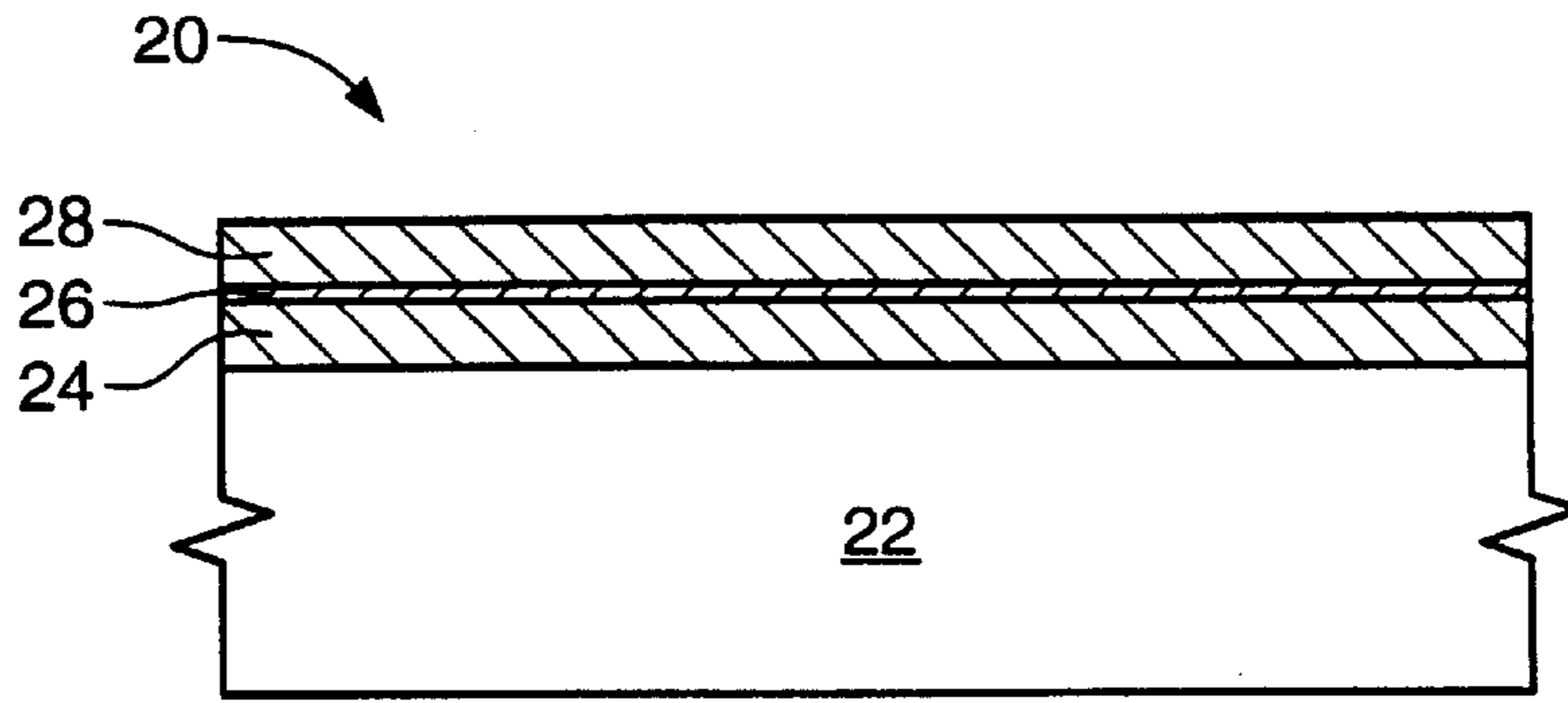
FIG. 1 (PRIOR ART)
