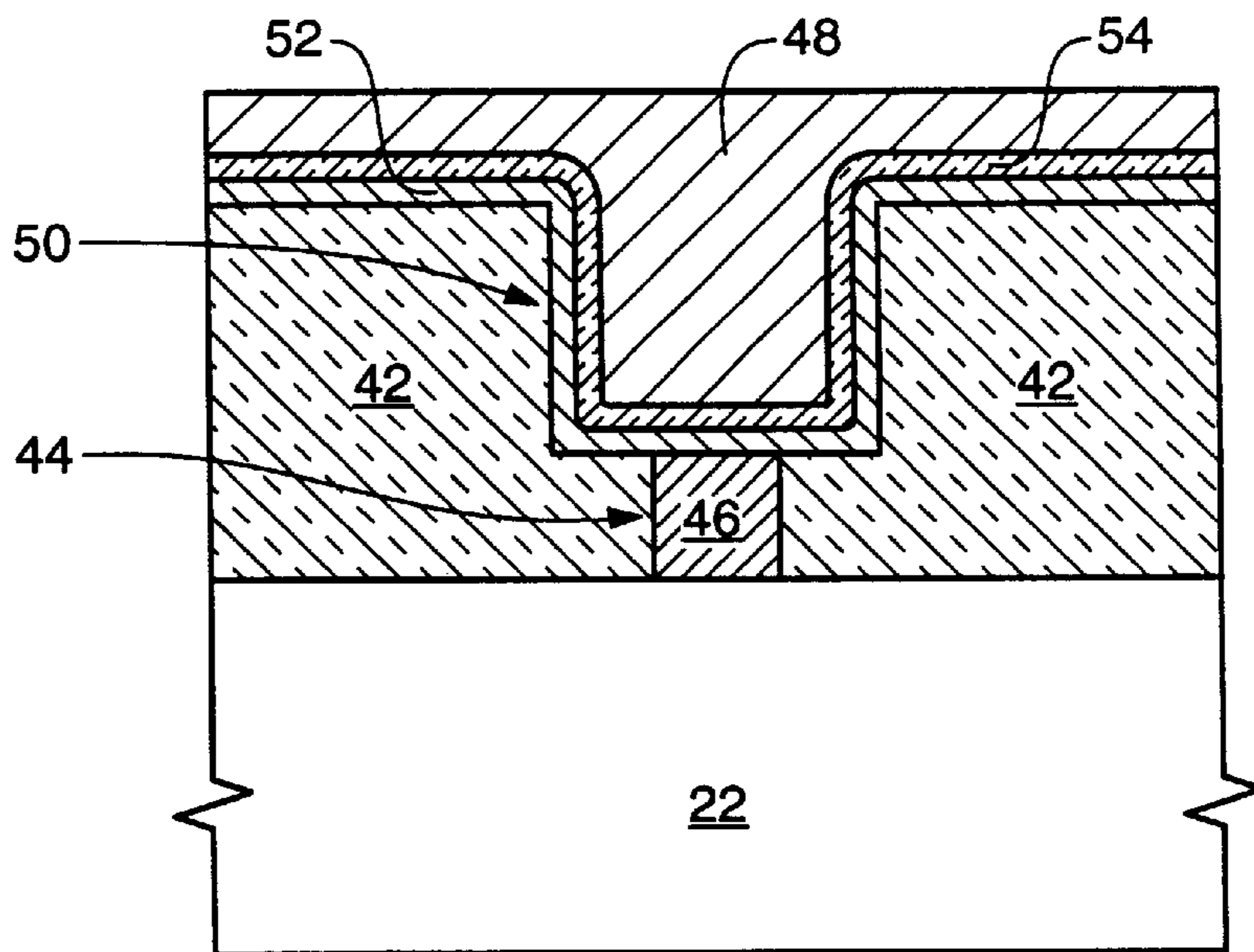
FIG. 8 (PRIOR ART)
