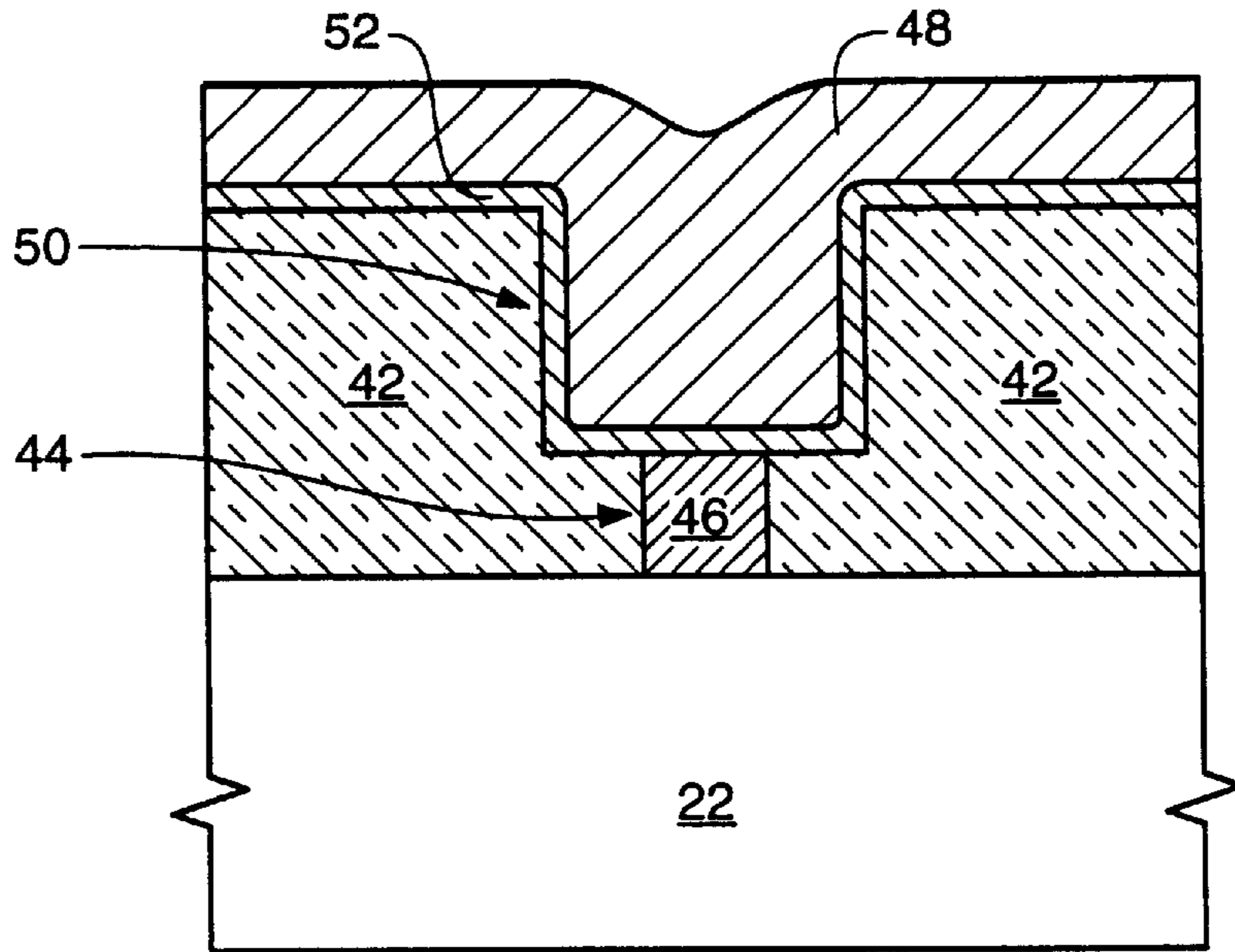
FIG. 7 (PRIOR ART)
