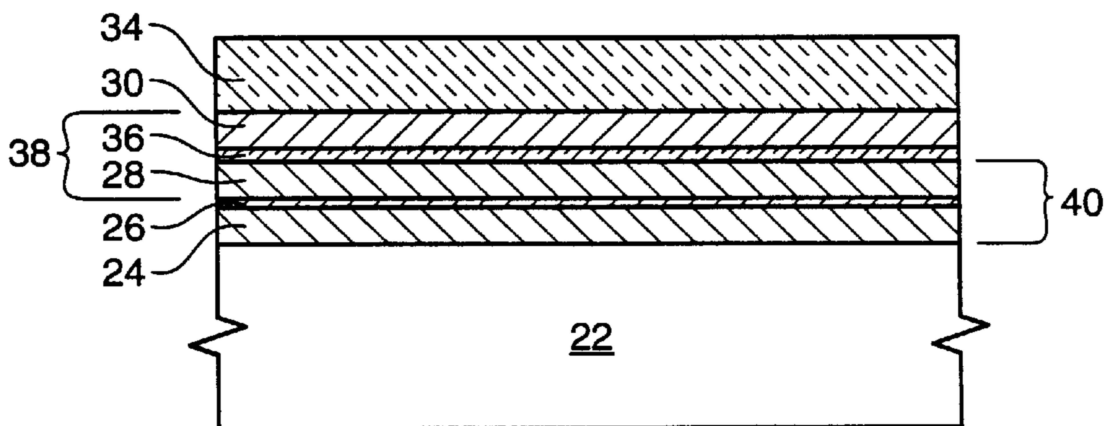
FIG. 3 (PRIOR ART)
