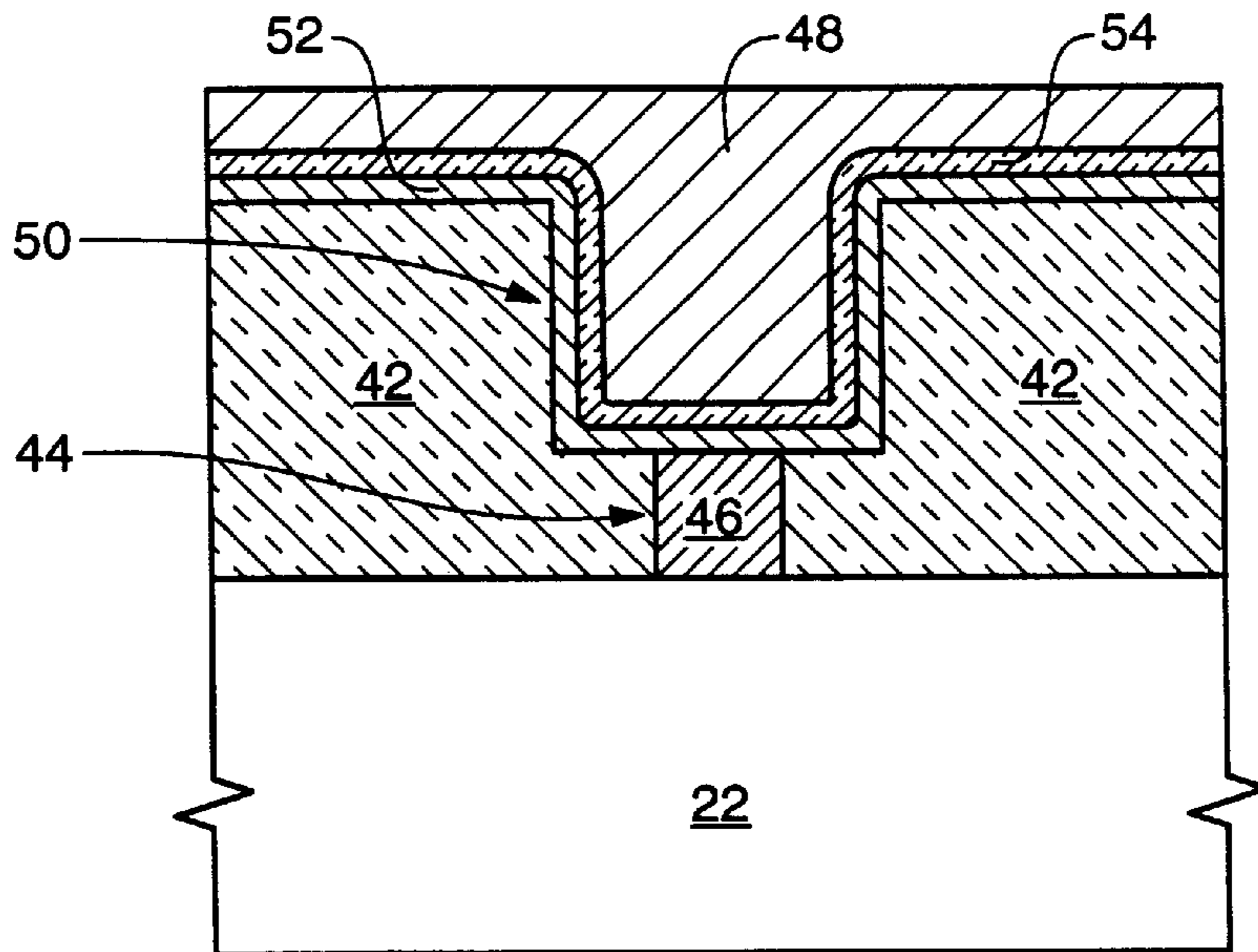
FIG. 8 (PRIOR ART)
