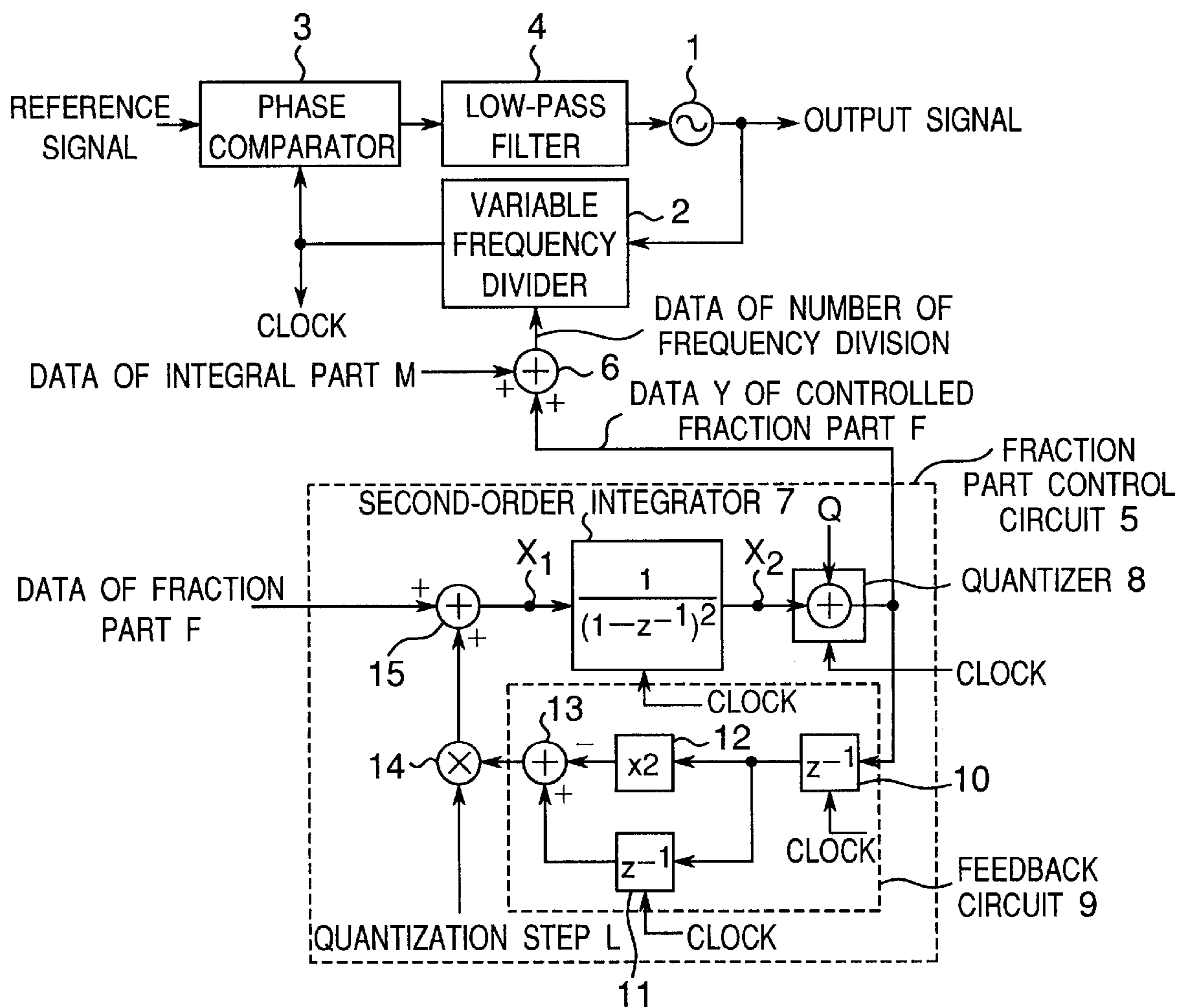
FIRST PREFERRED EMBODIMENT FREQUENCY SYNTHESIZER APPARATUS
