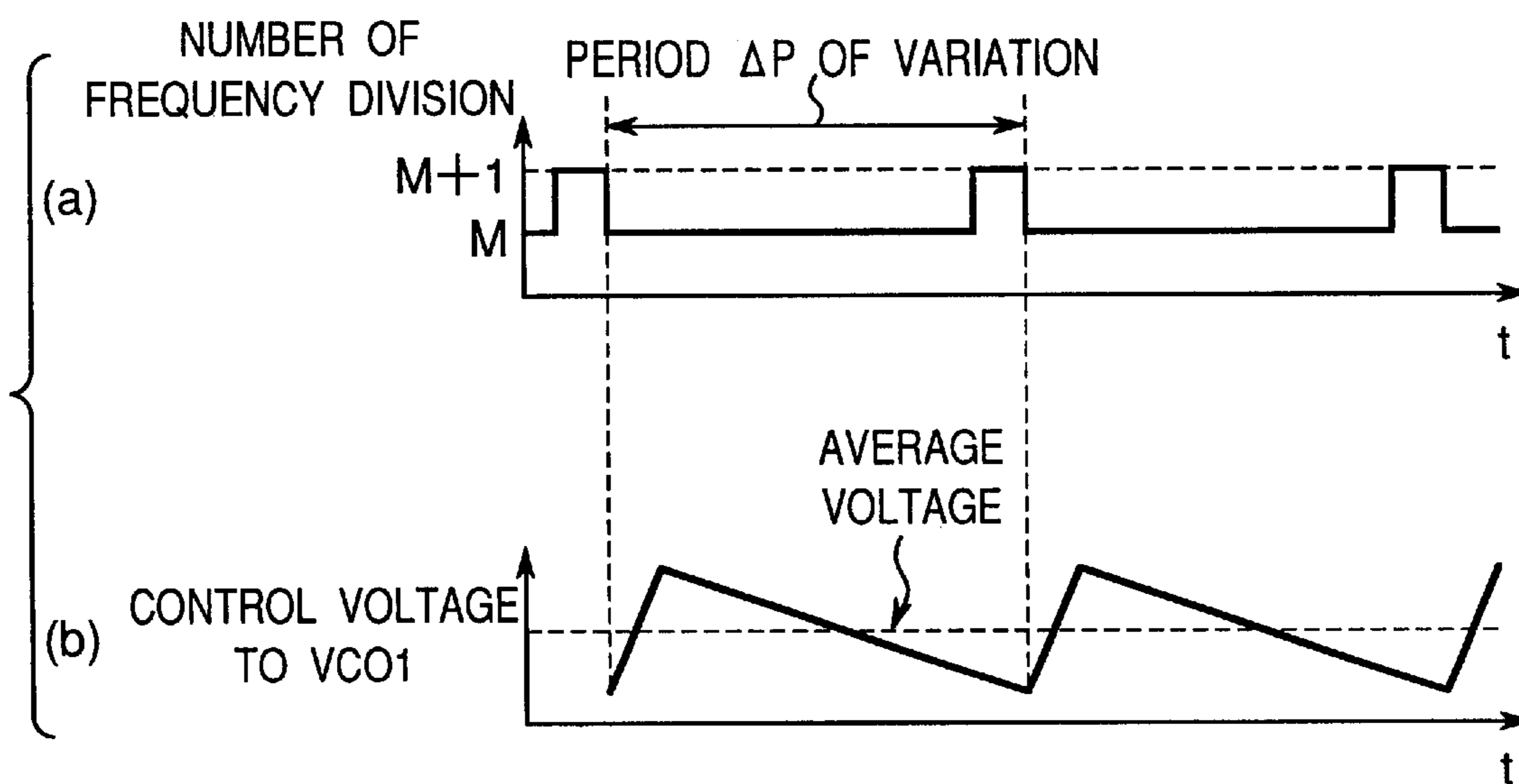
Fig.21 PRIOR ART
