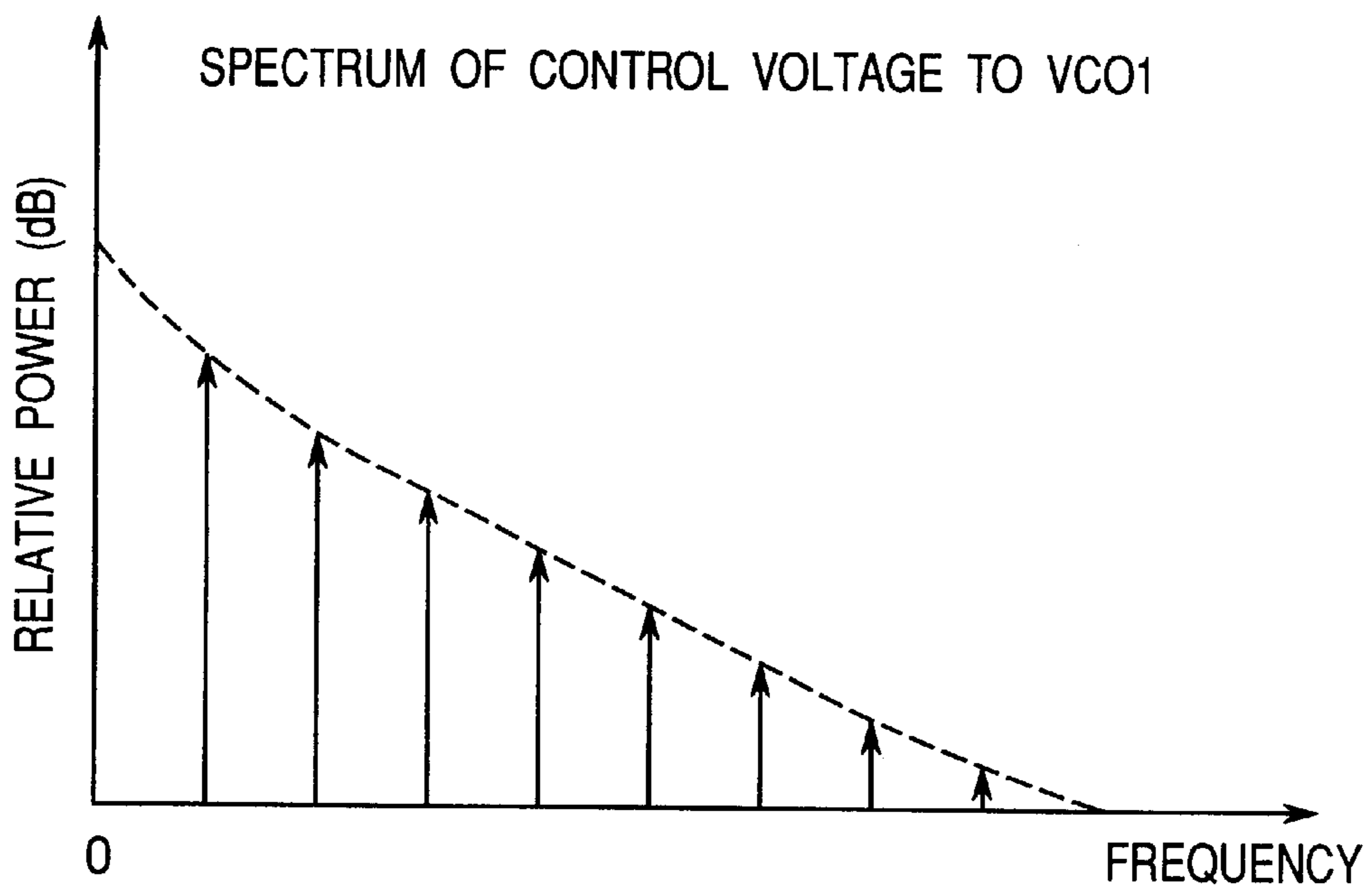
Fig.23 PRIOR ART
