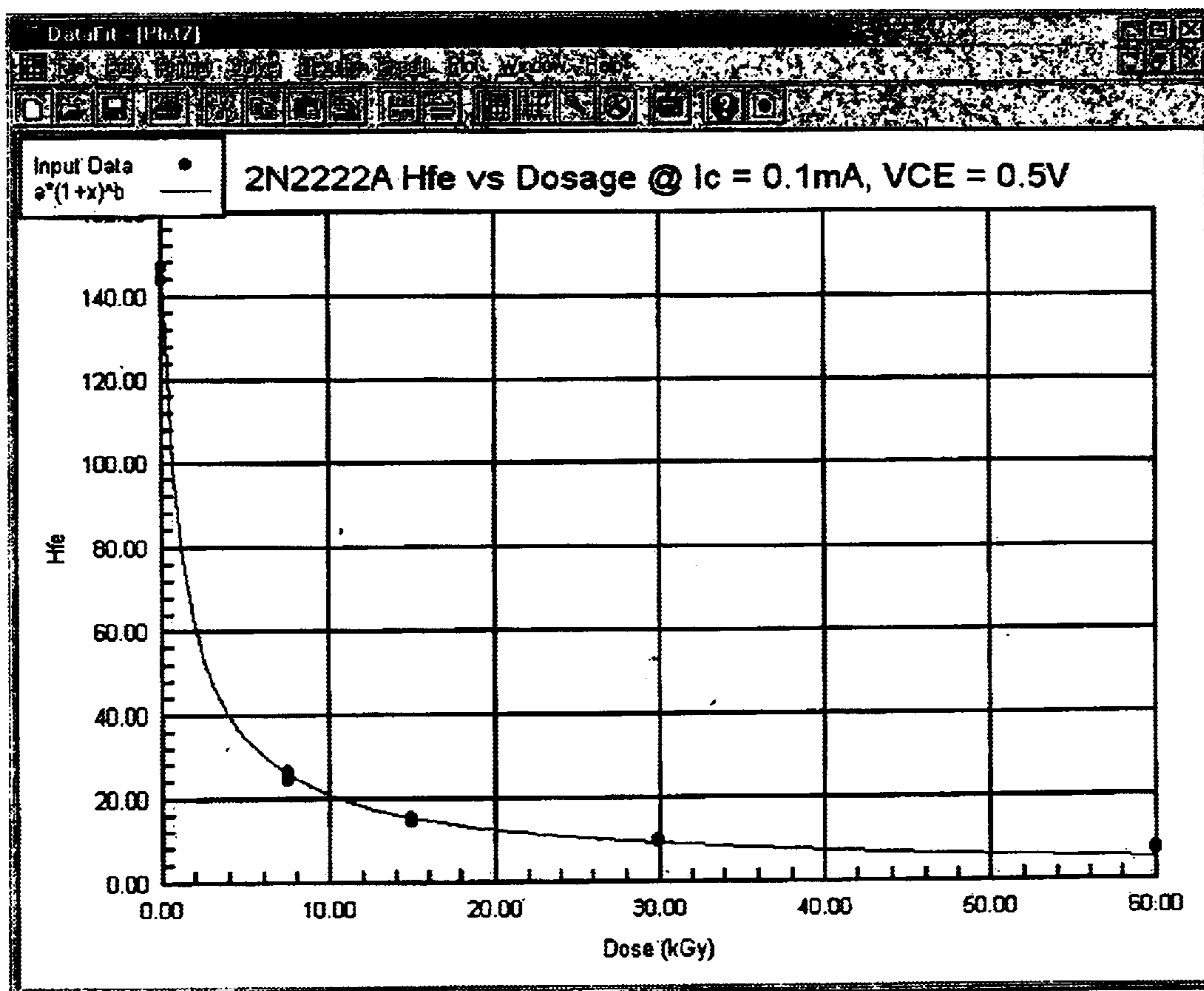
2N2222A Hfe vs. Total Dose.
