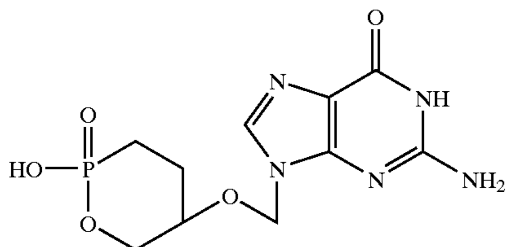
Ganciclovir cyclic phosphonate
