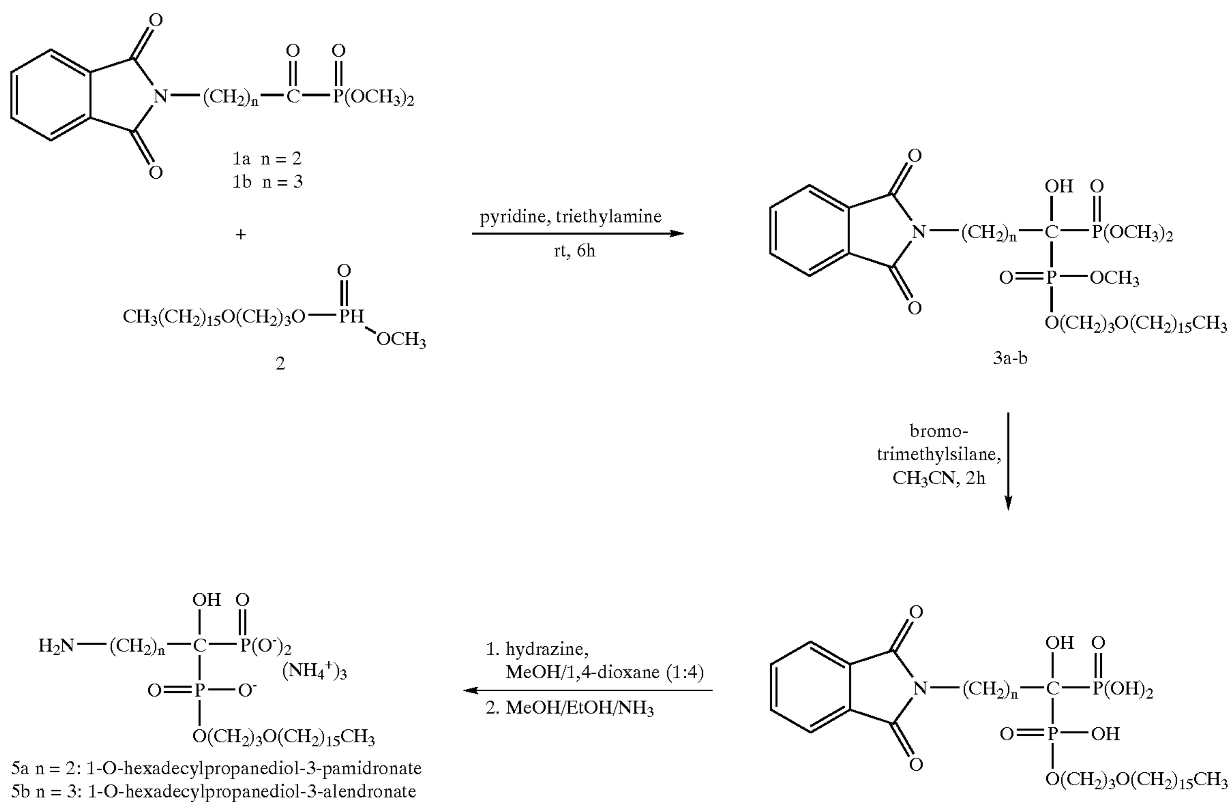
Scheme I
