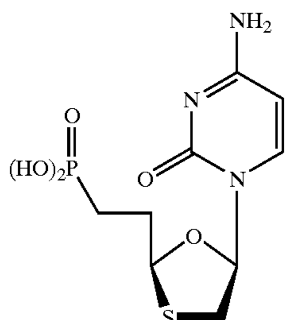
3'-thia-2',3'-dideoxycytidine-5'-phosphonic acid
