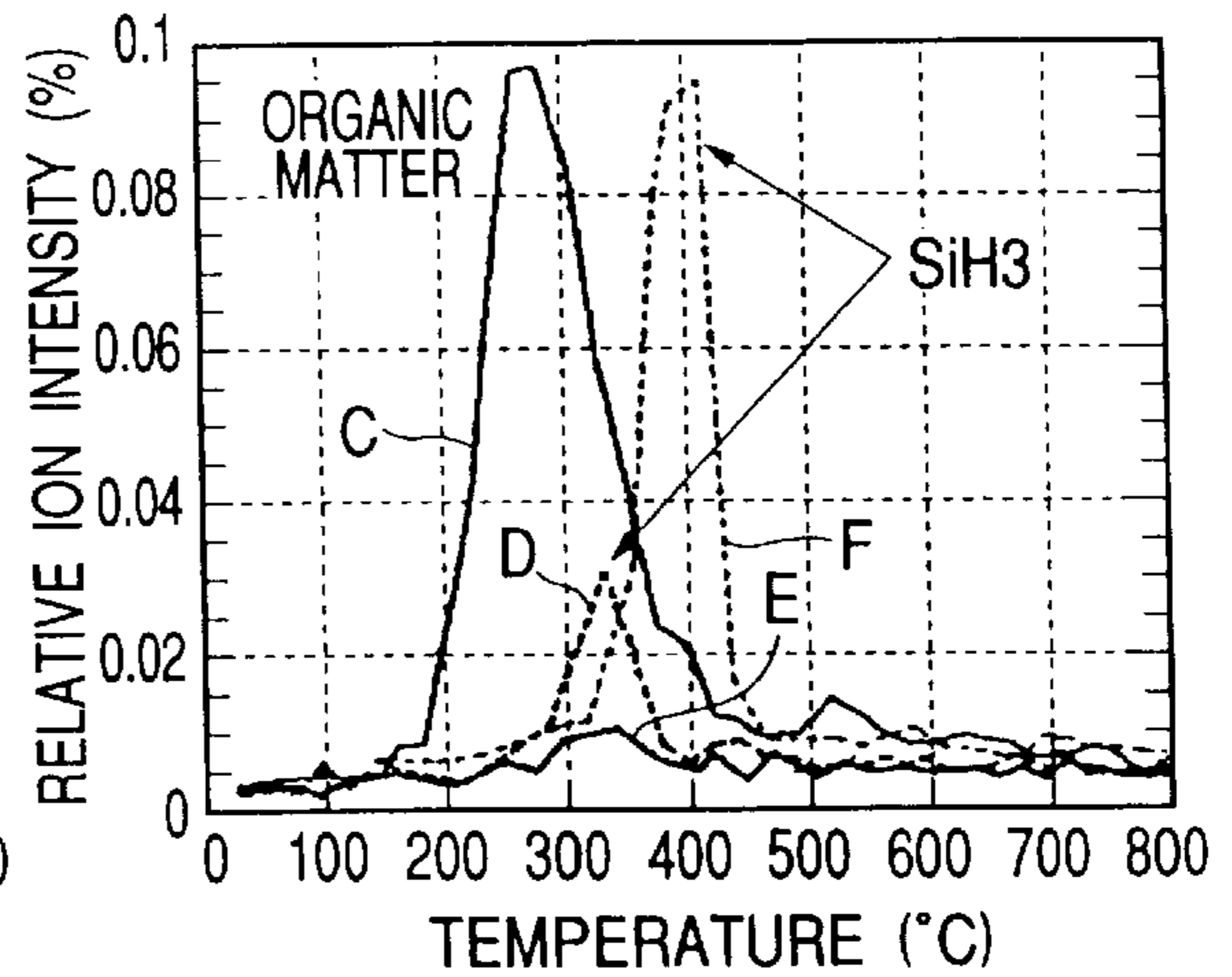
THERMAL ELIMINATION OF SiH 3 AND ORGANIC MATTER SiH 3 m/z=31
