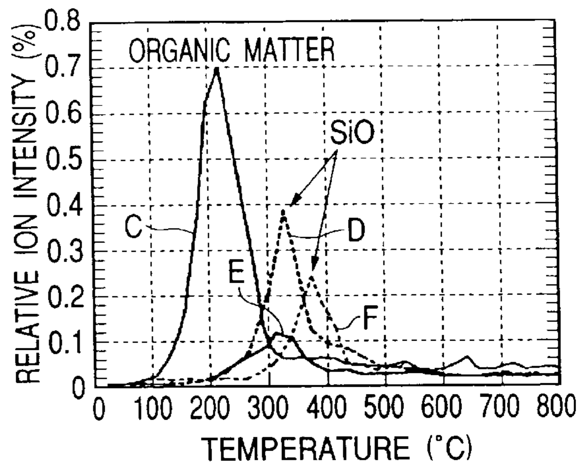
THERMAL ELIMINATION OF SiO AND ORGANIC MATTER SiO, C 3 H 6 m/z=44
