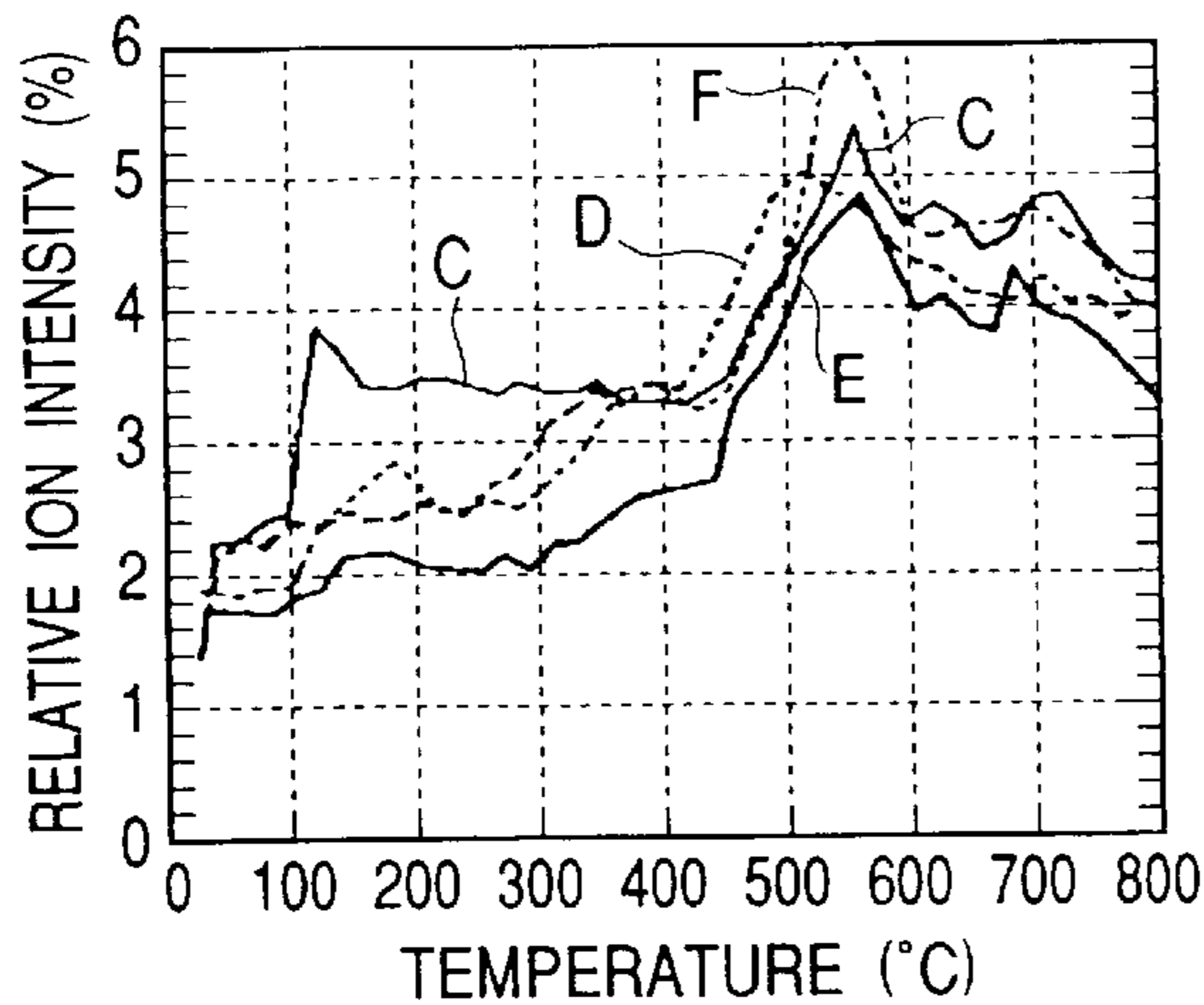
THERMAL ELIMINATION OF HYDROGEN Ar-H m/z=41
