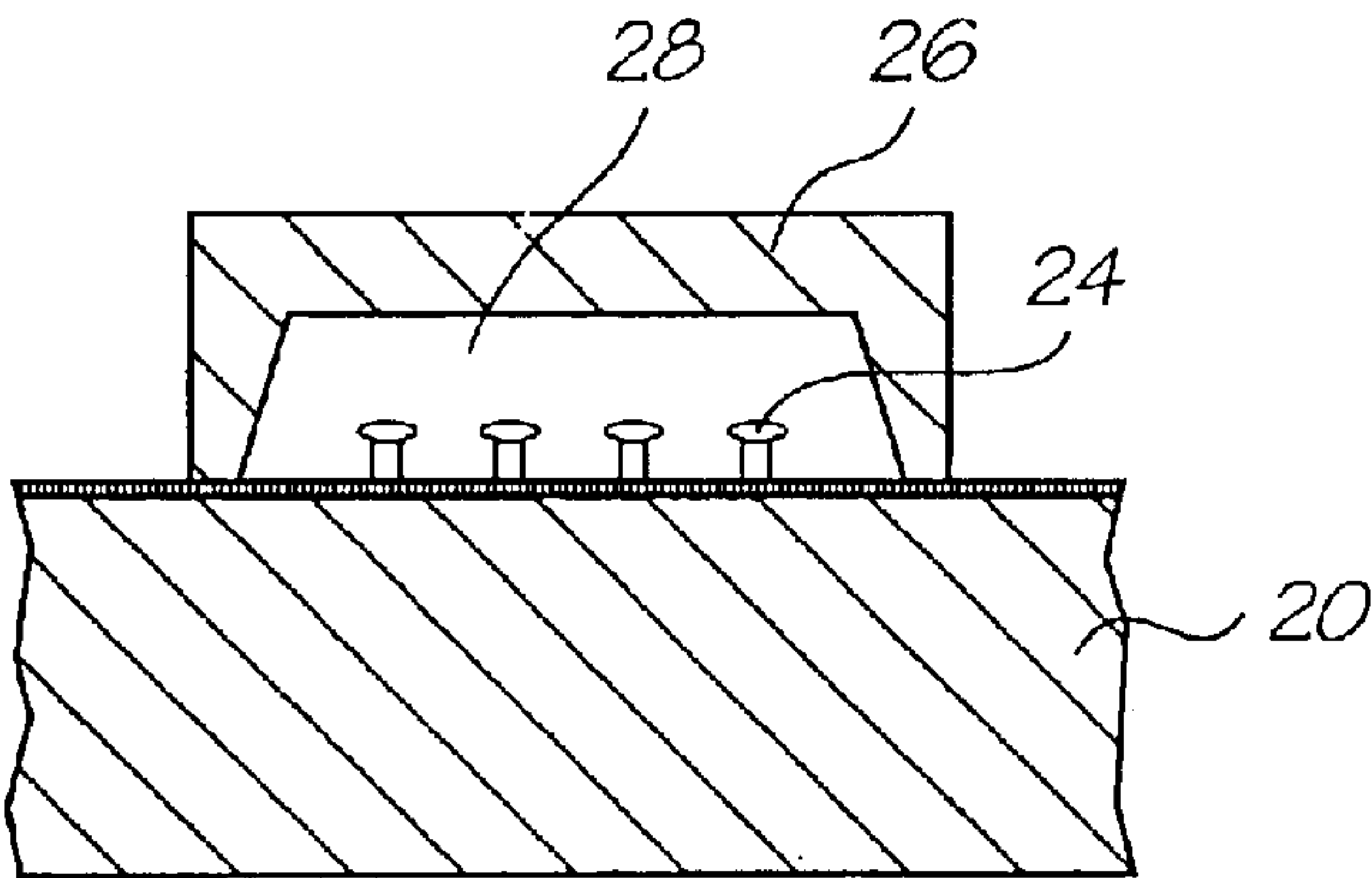
FIG. 3 (Prior Art)
