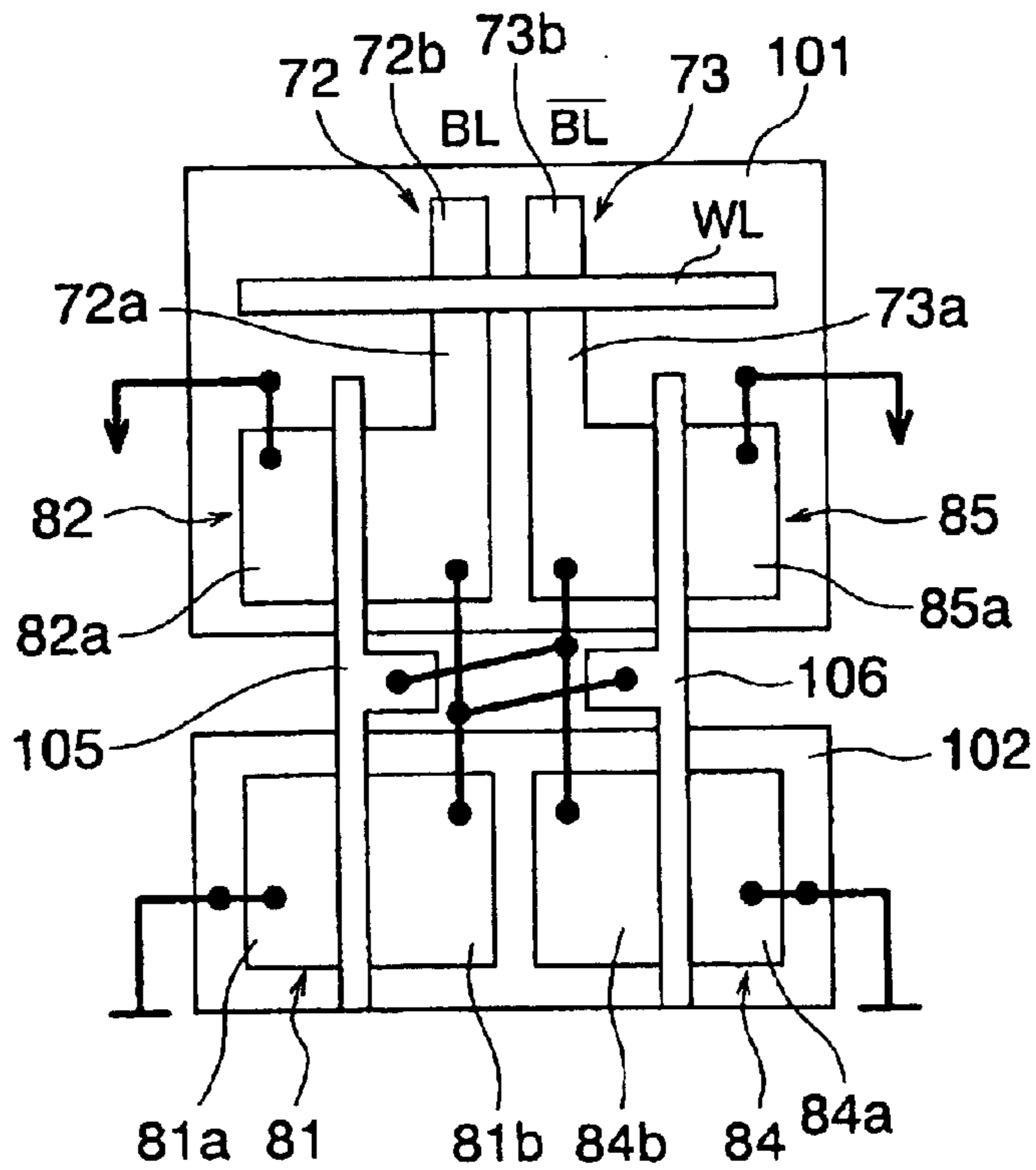
PRIOR ART FIG. 9
