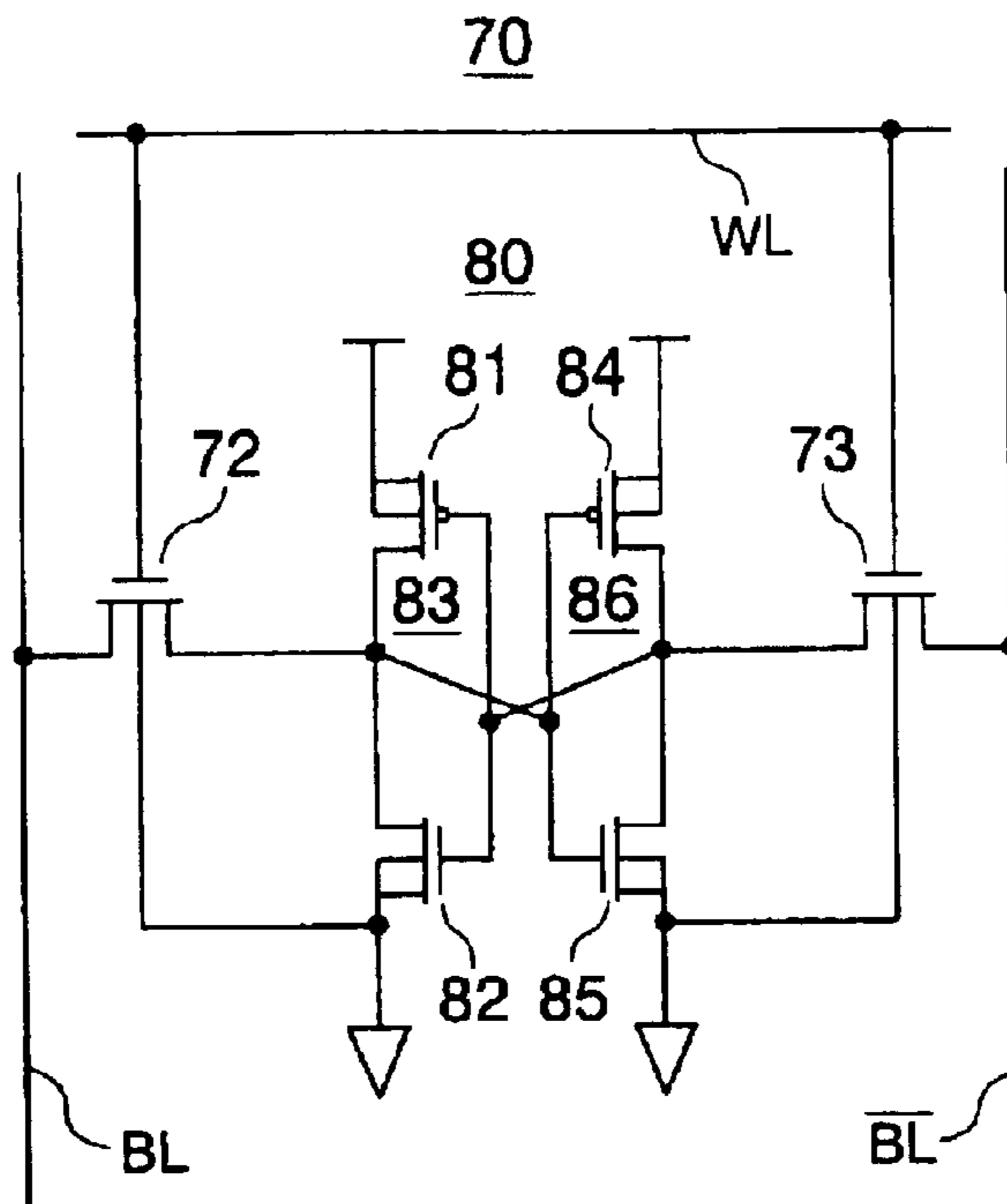
PRIOR ART FIG. 8
