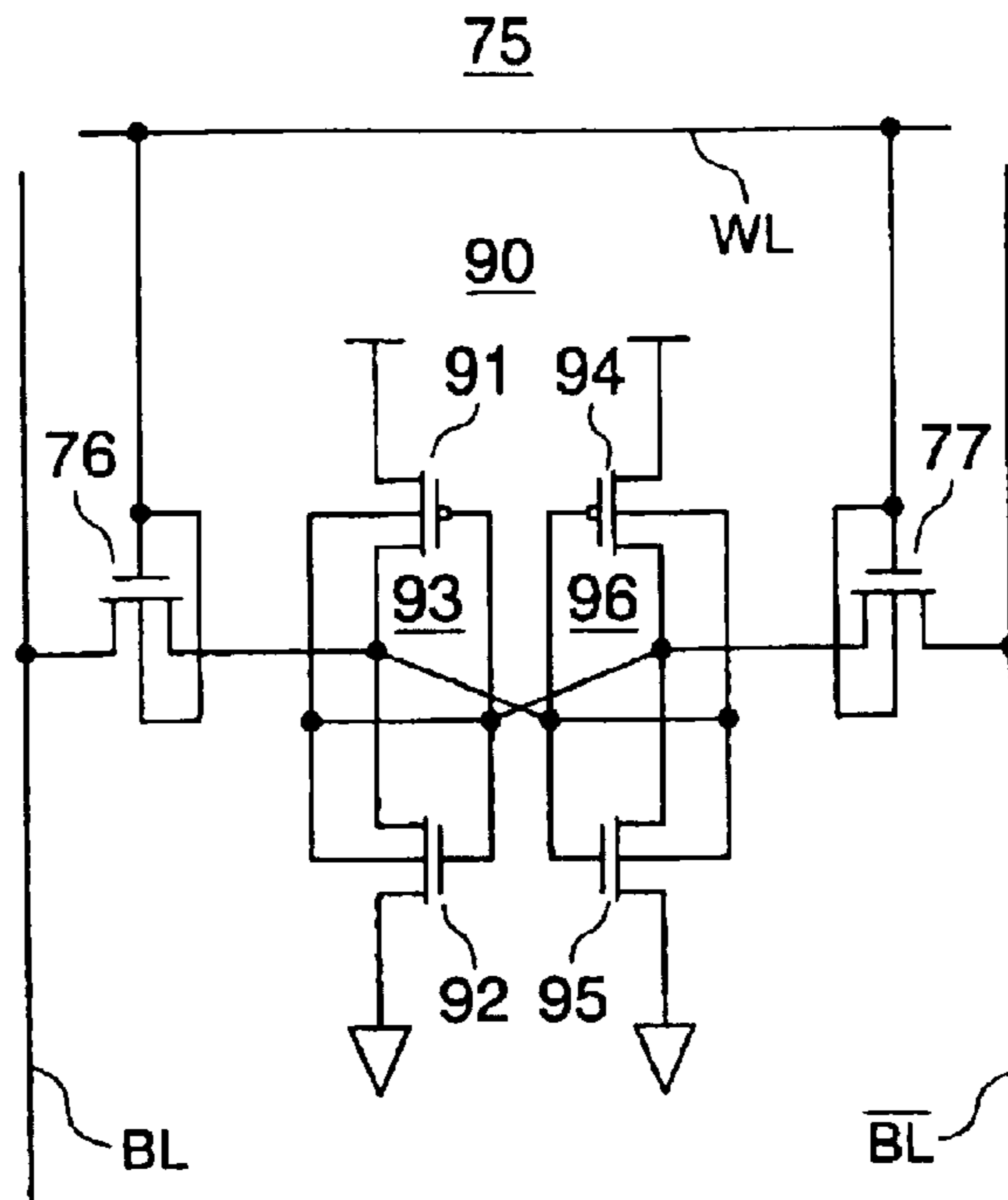
PRIOR ART FIG. 10
