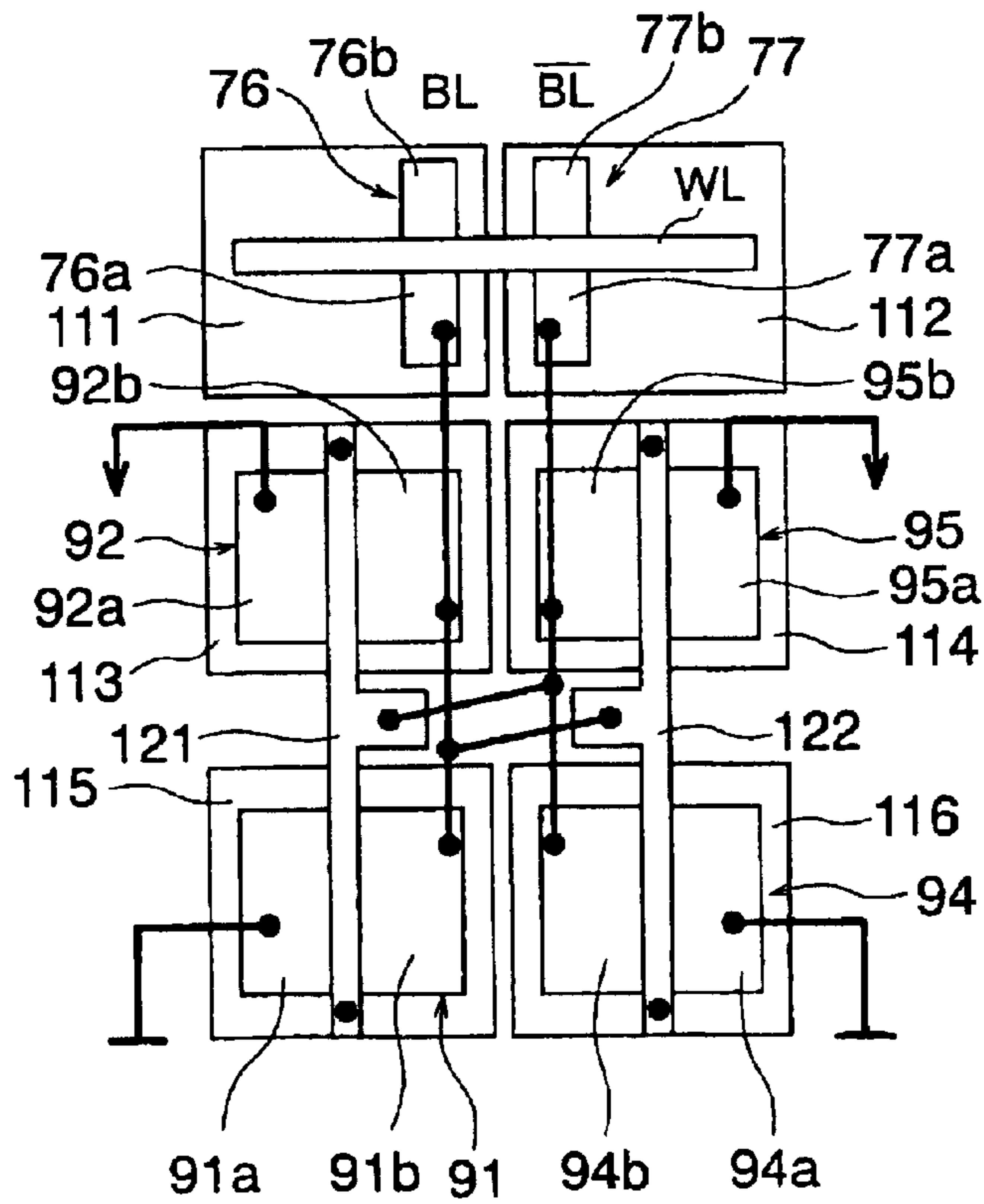
PRIOR ART FIG. 11
