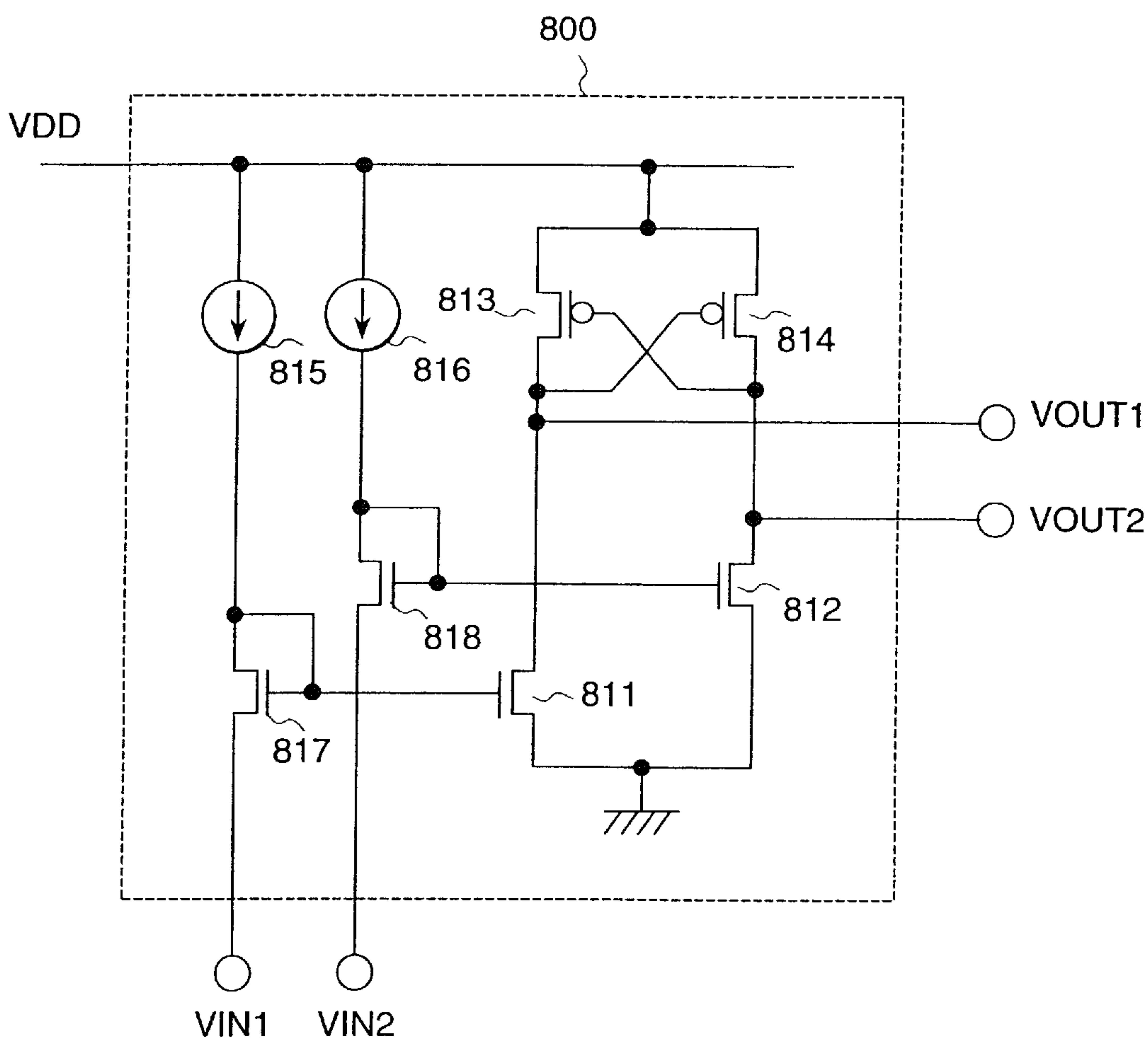
FIG. 9 (PRIOR ART)
