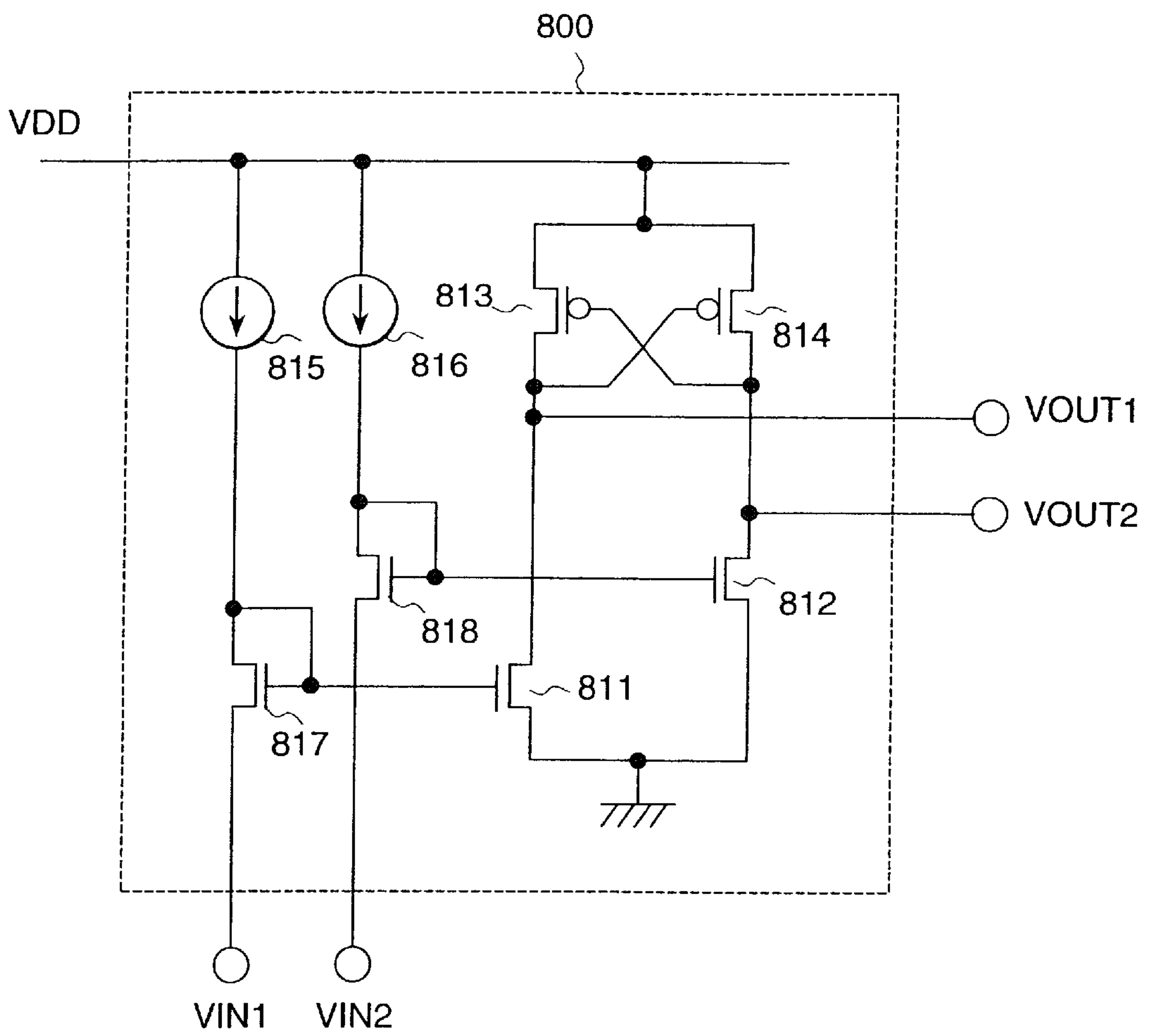
FIG. 9 (PRIOR ART)
