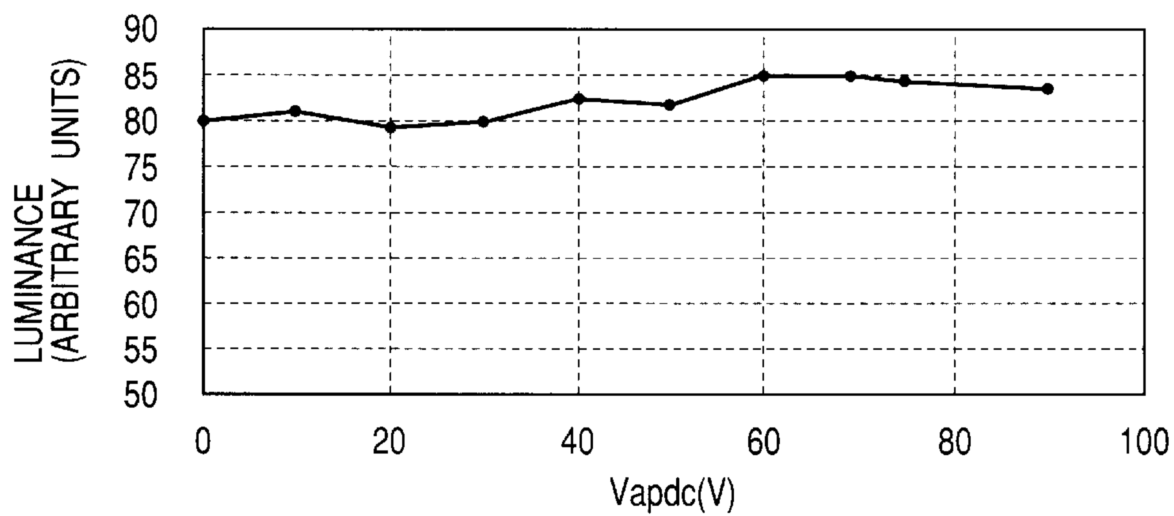
Vapdc DEPENDENCY OF LUMINANCE
