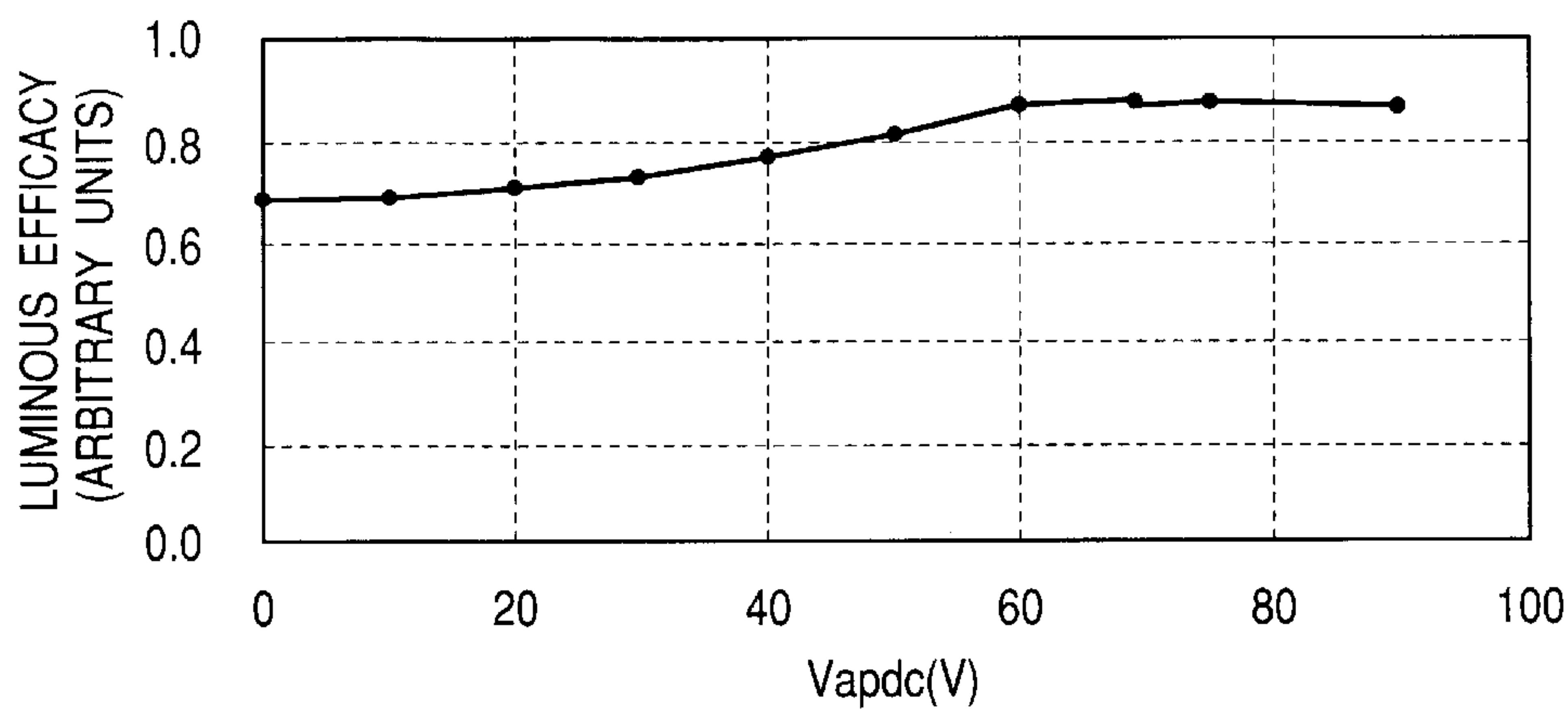
Vapdc DEPENDENCY OF LUMINOUS EFFICACY
