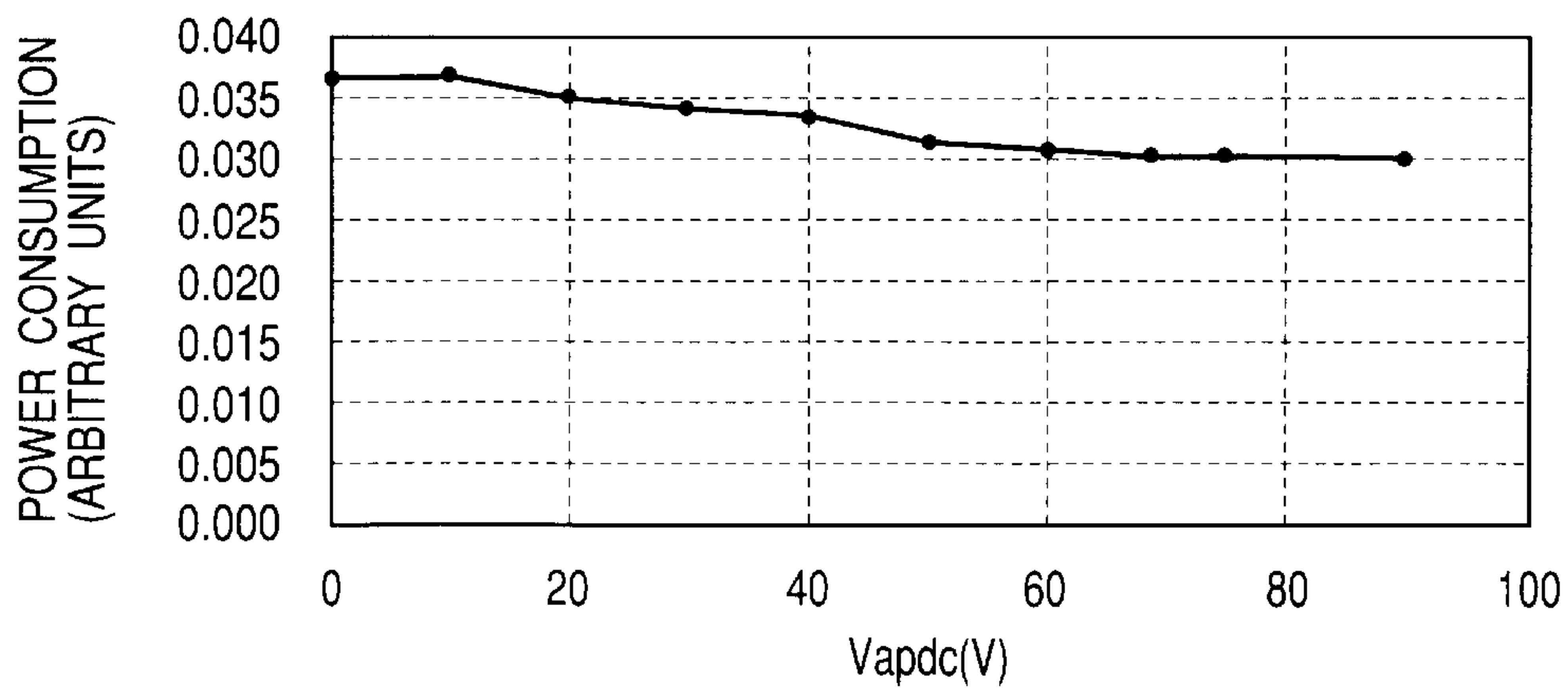
Vapdc DEPENDENCY OF POWER CONSUMPTION
