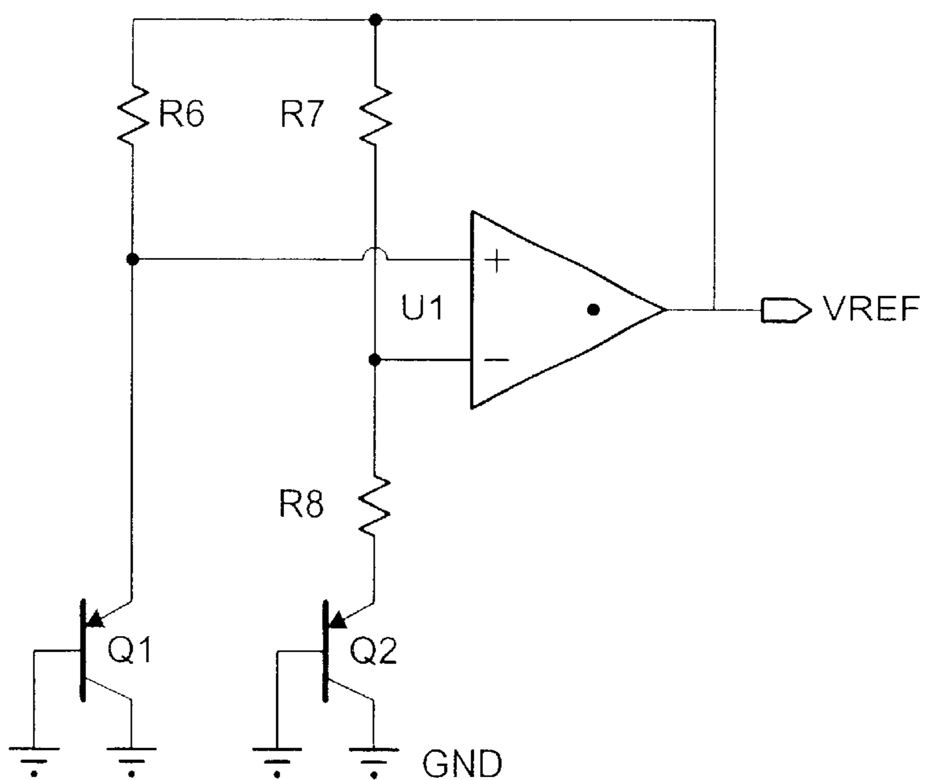
Bandgap Voltage Reference FIG. 7D (Prior Art)
