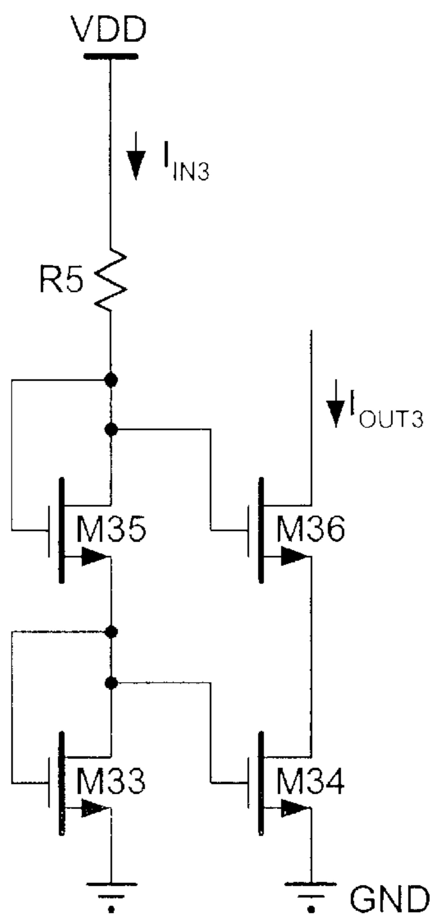
Cascode Current Mirror FIG. 7B (Prior Art)
