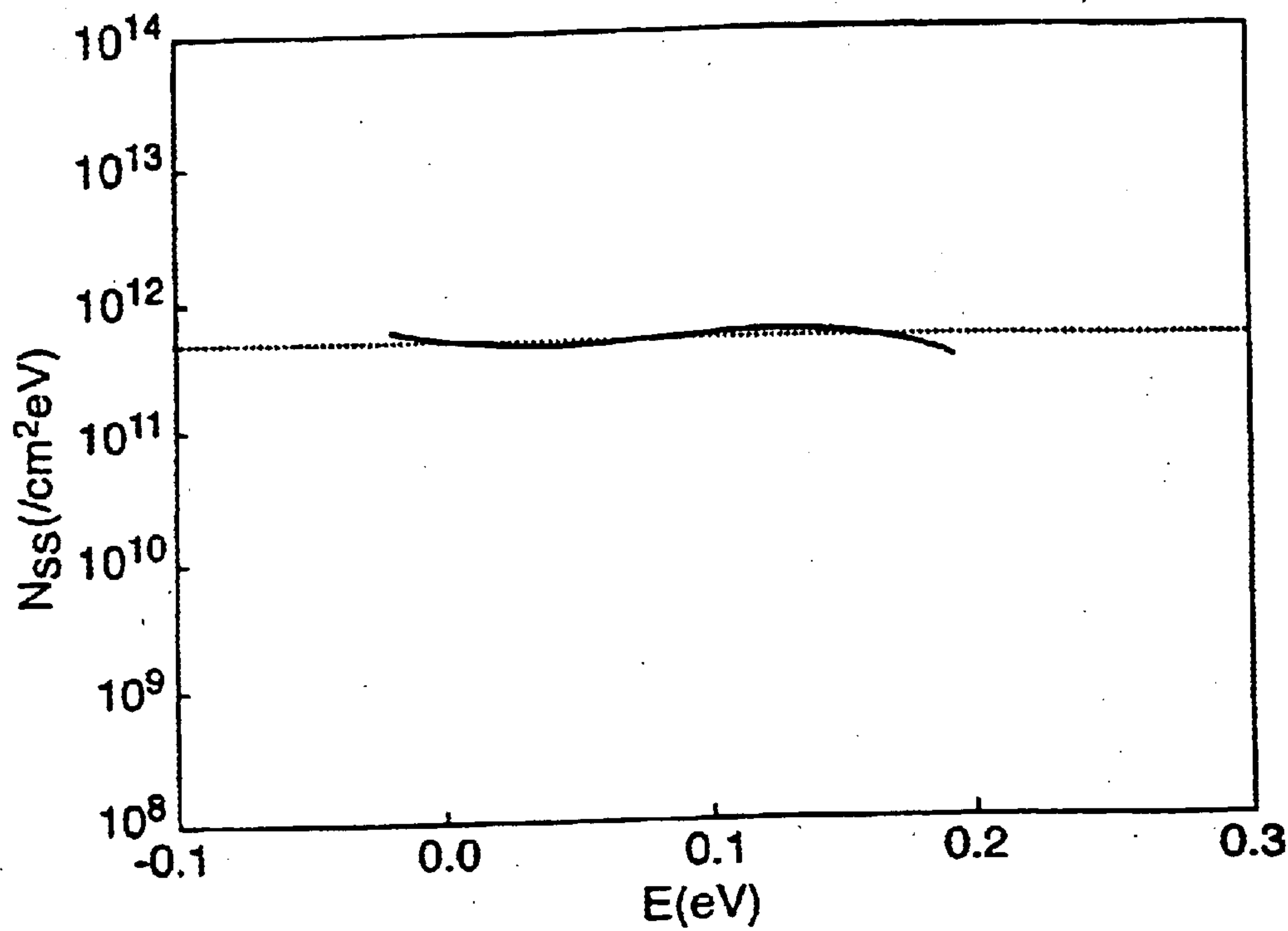
Fig.11. PRIOR ART
