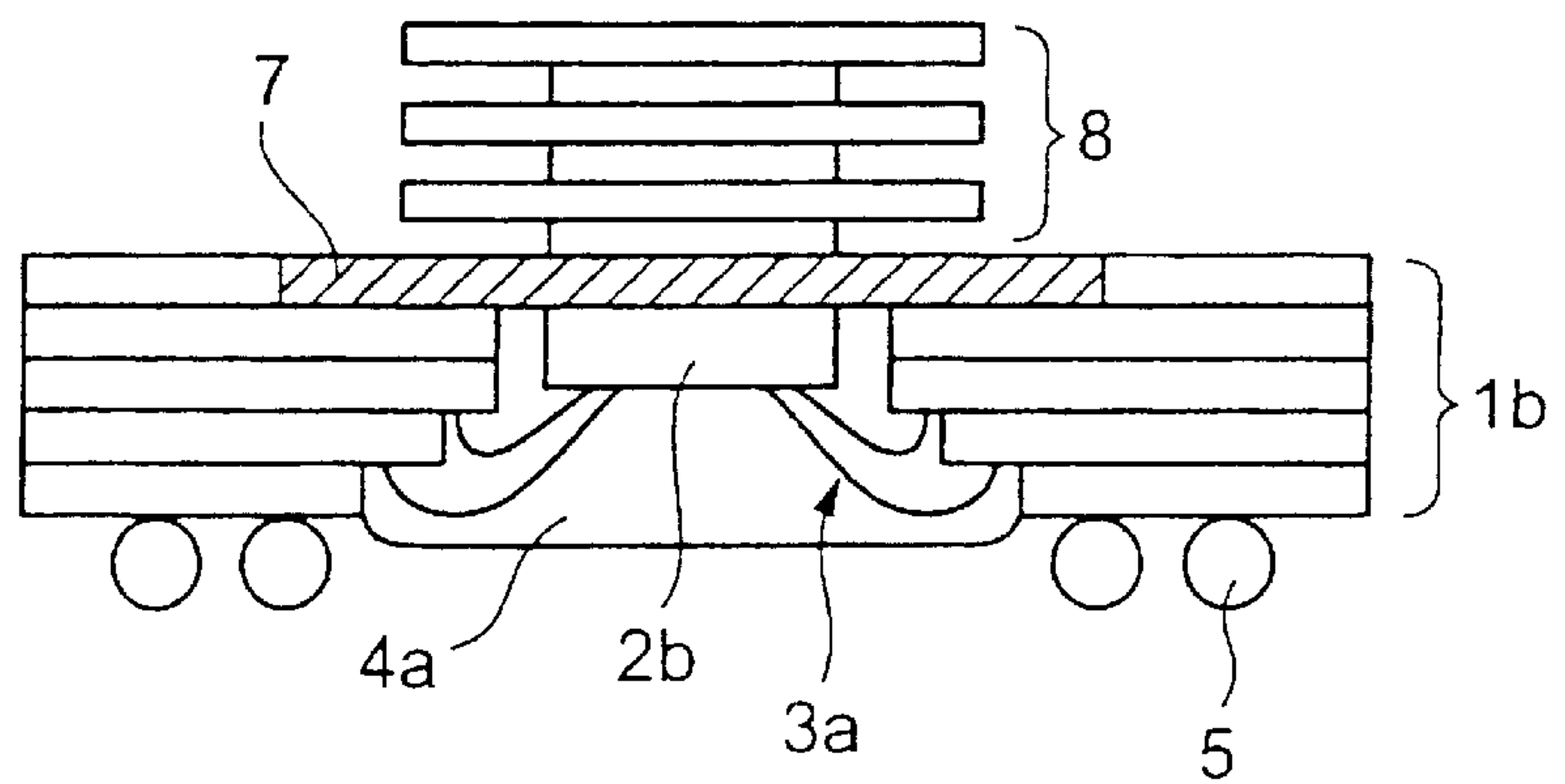
FIG. 1C PRIOR ART
