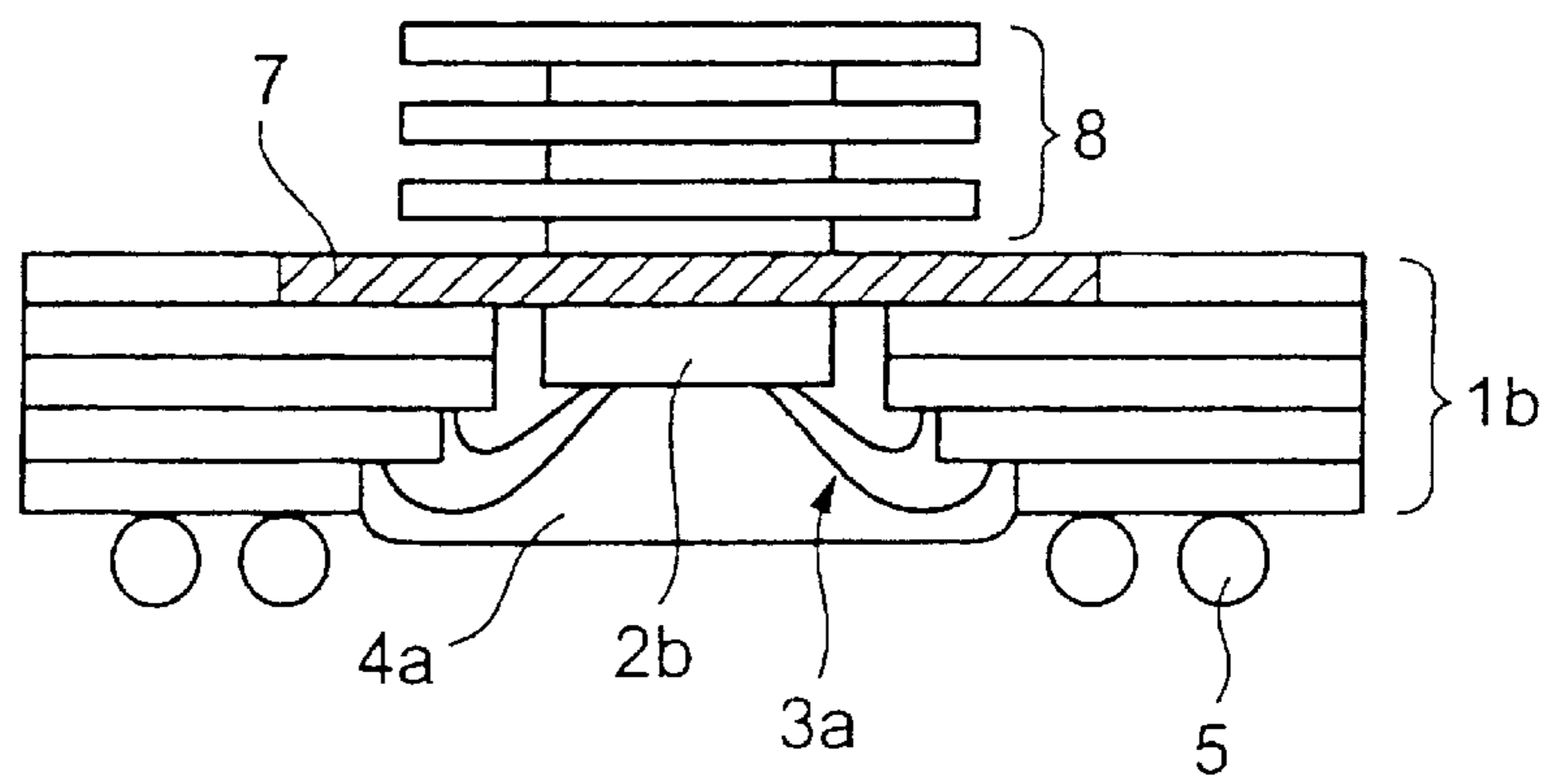
FIG. 1C PRIOR ART
