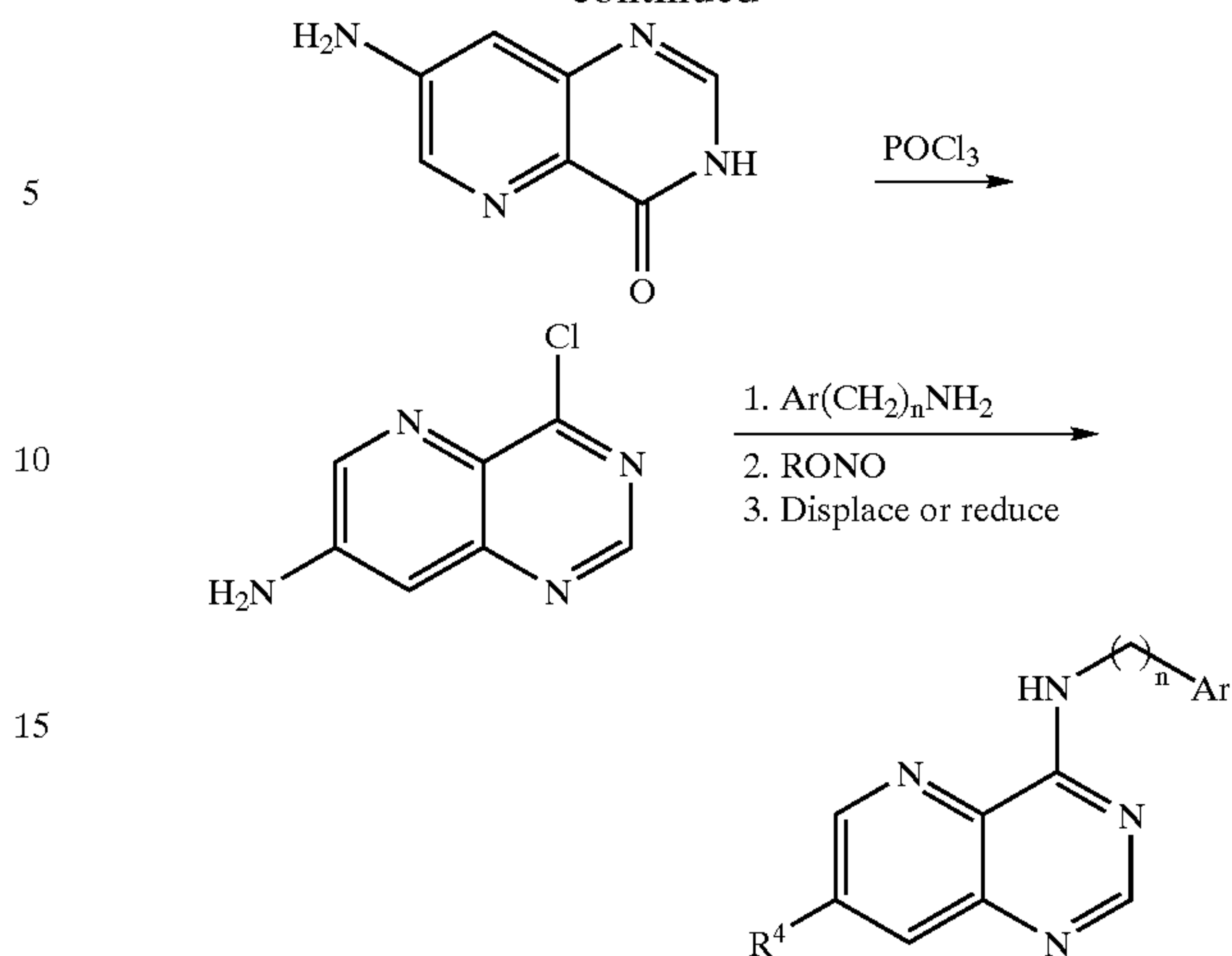
Scheme 3.
