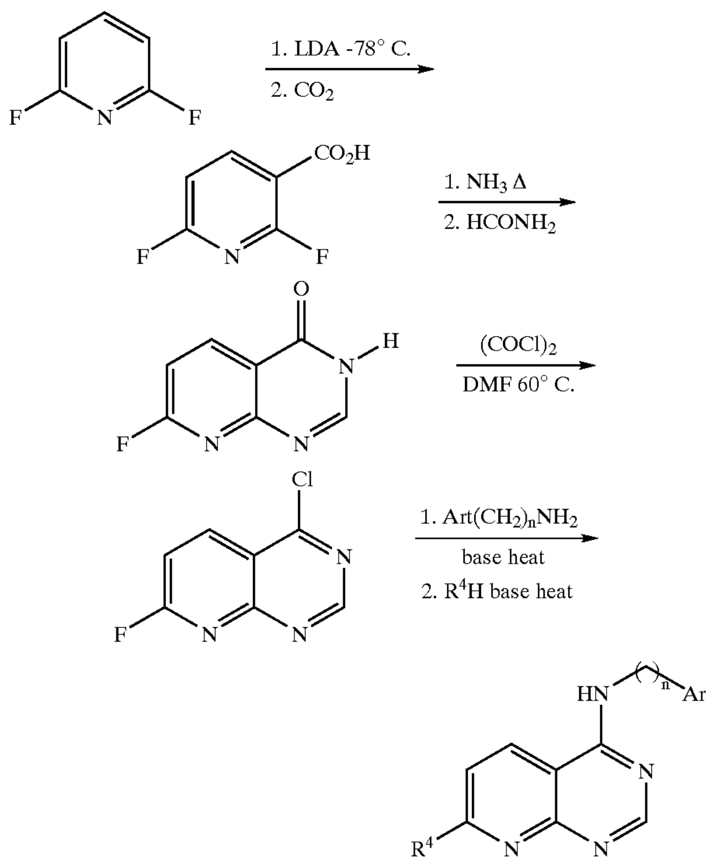
Scheme 11.
