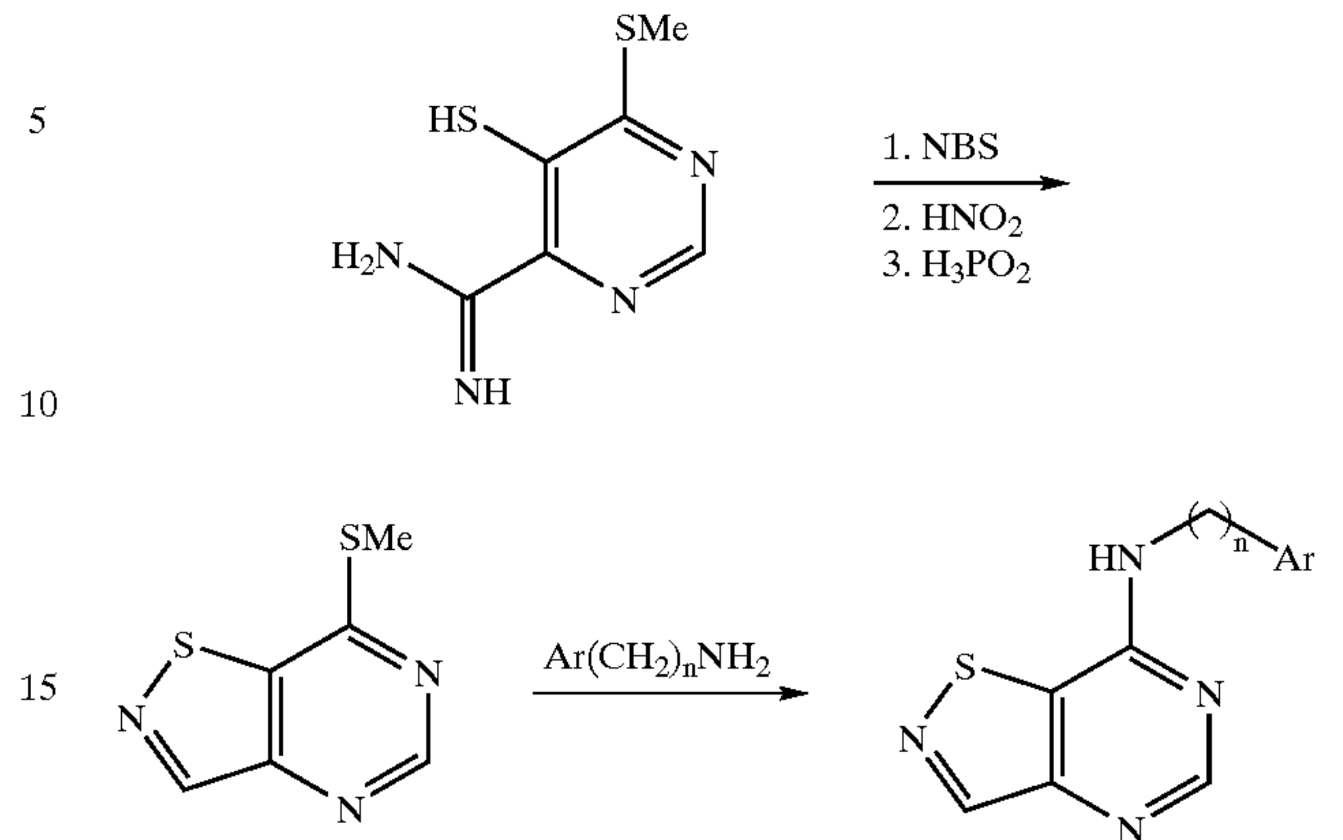
Scheme 32.
