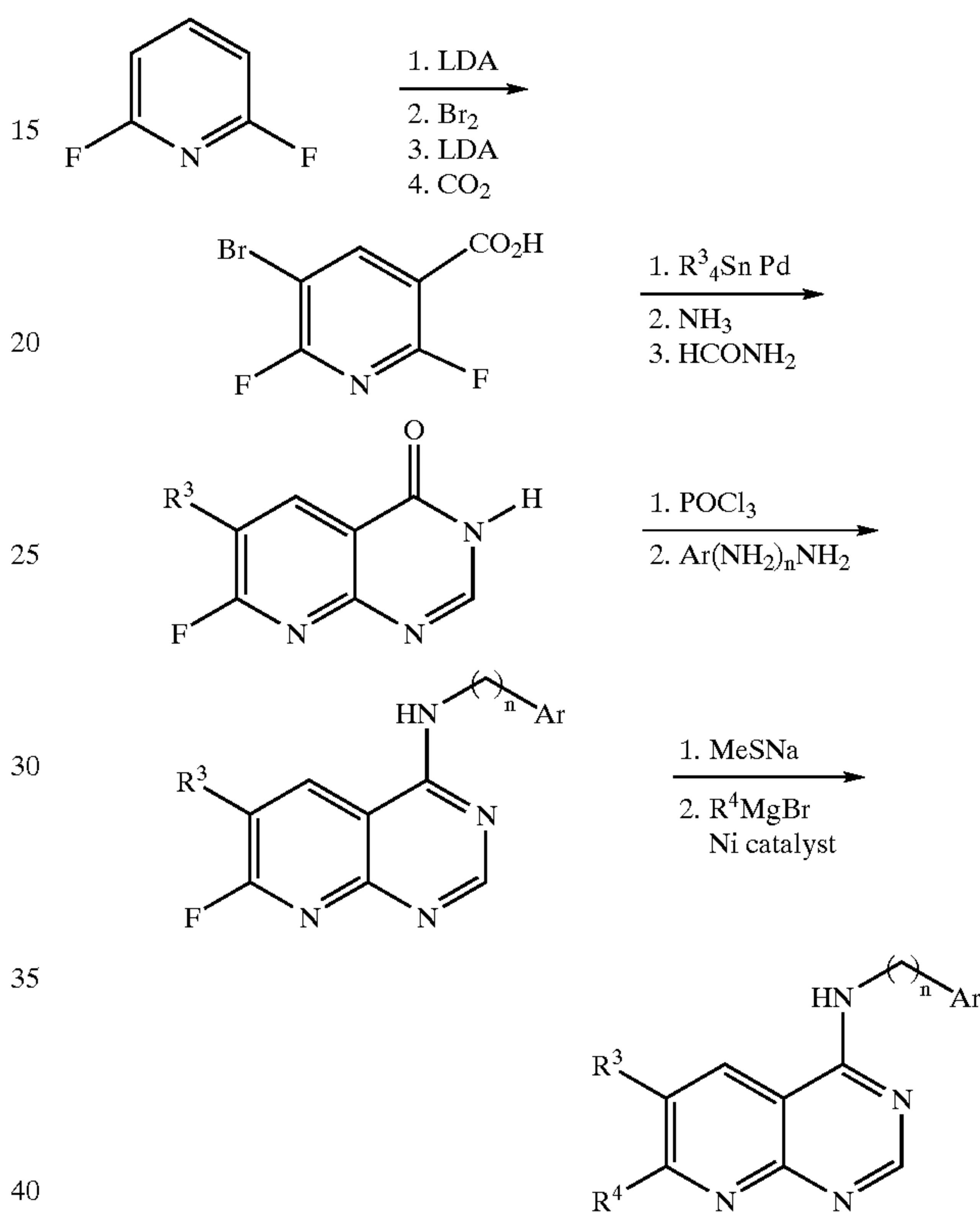
Scheme 13.
