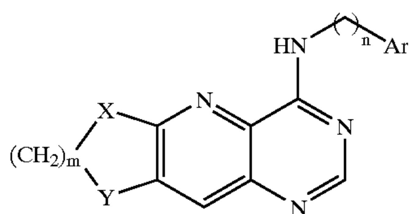
Scheme 7.
