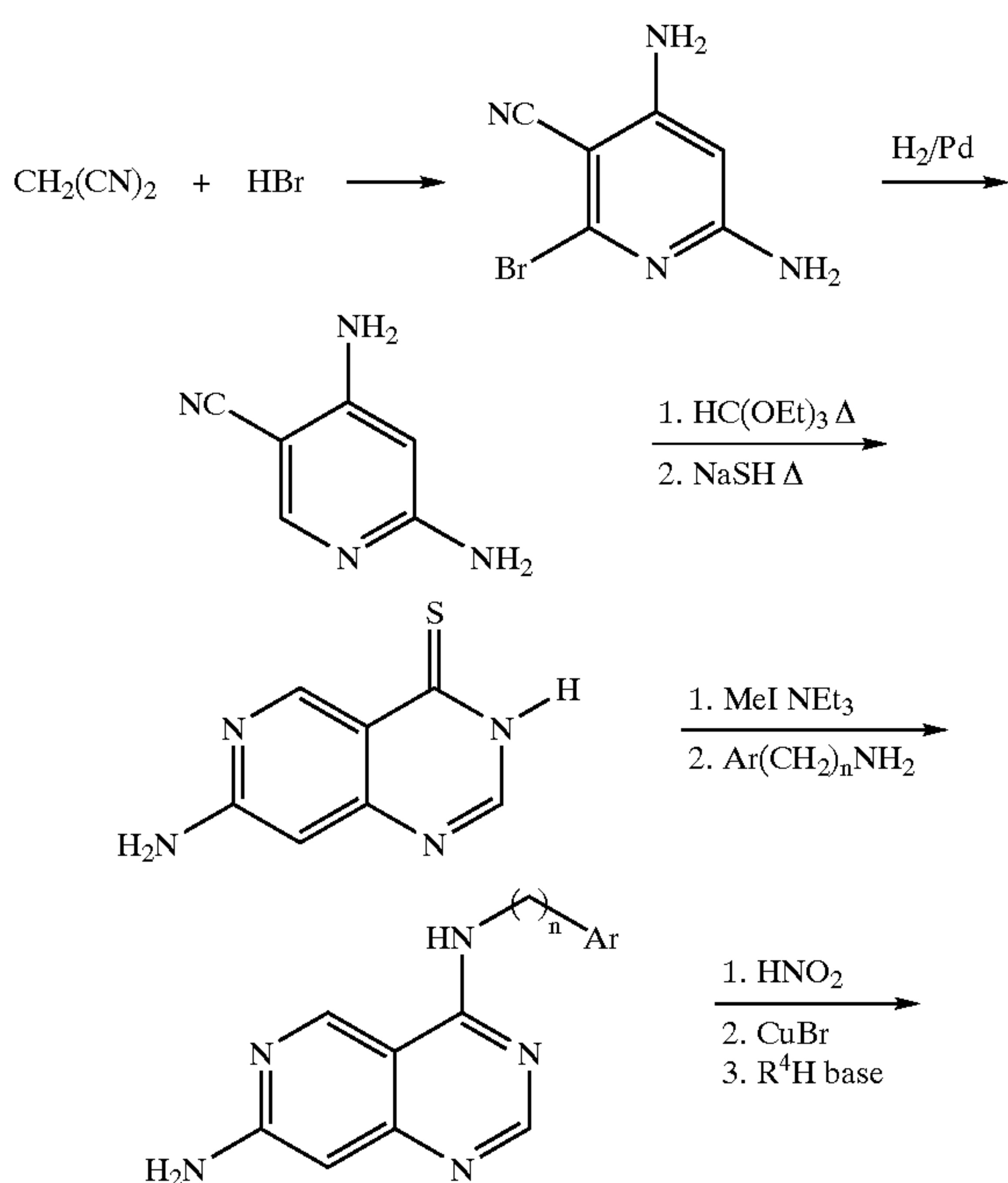
Scheme 7.
