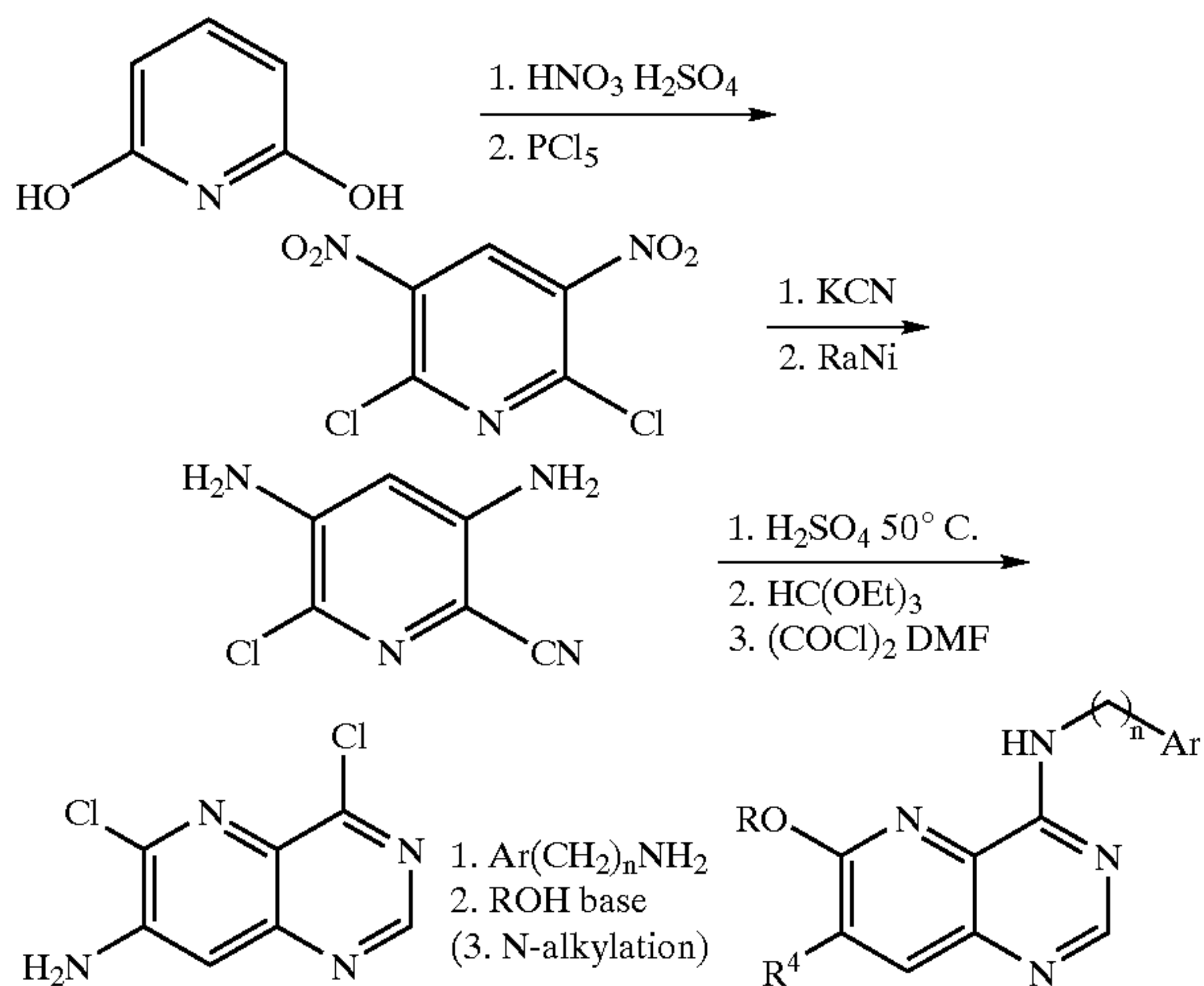
Scheme 6.
