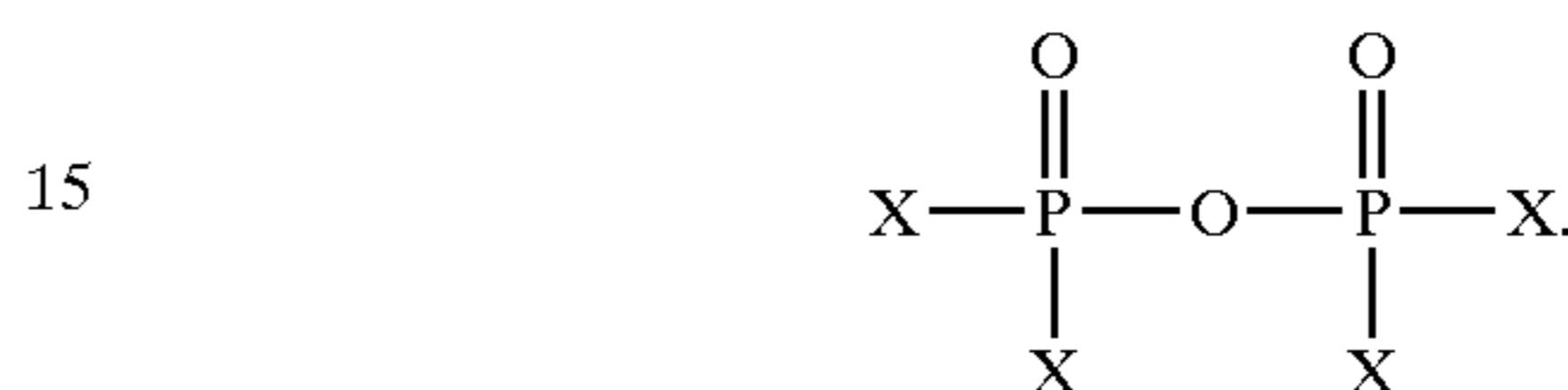
Formula IVb: Diphosphorylating Agents
