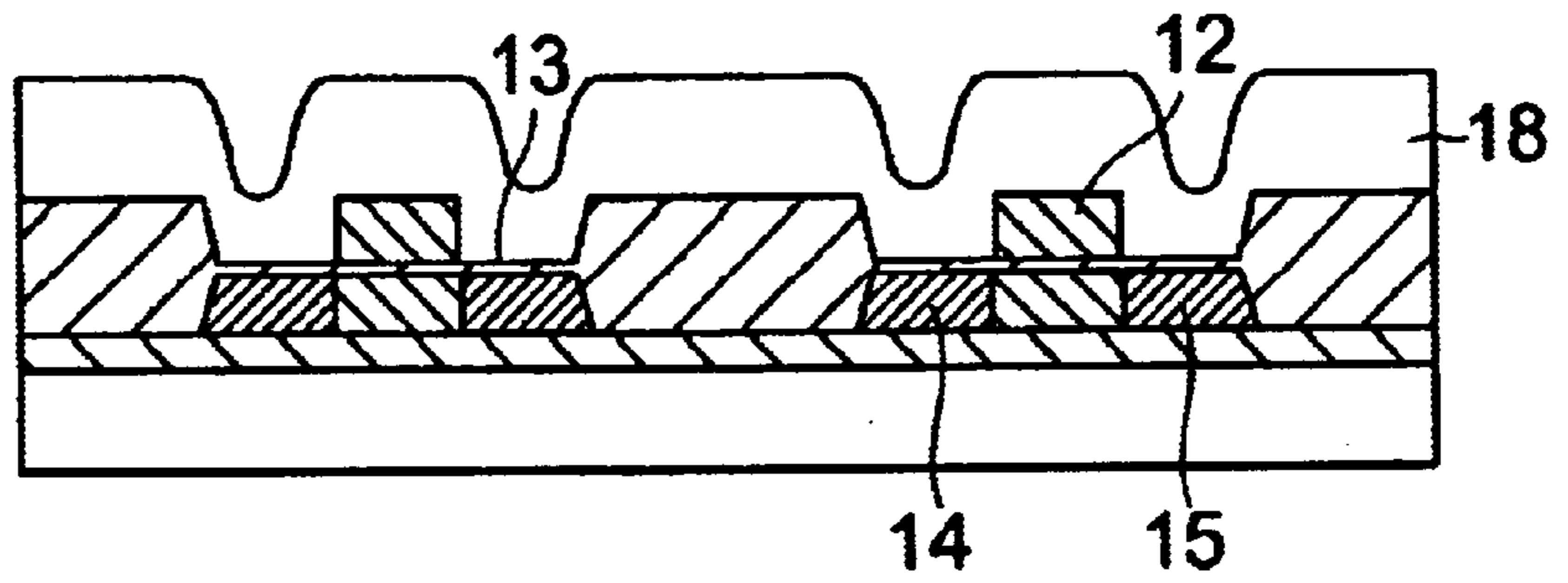
FIG.4C PRIOR ART
