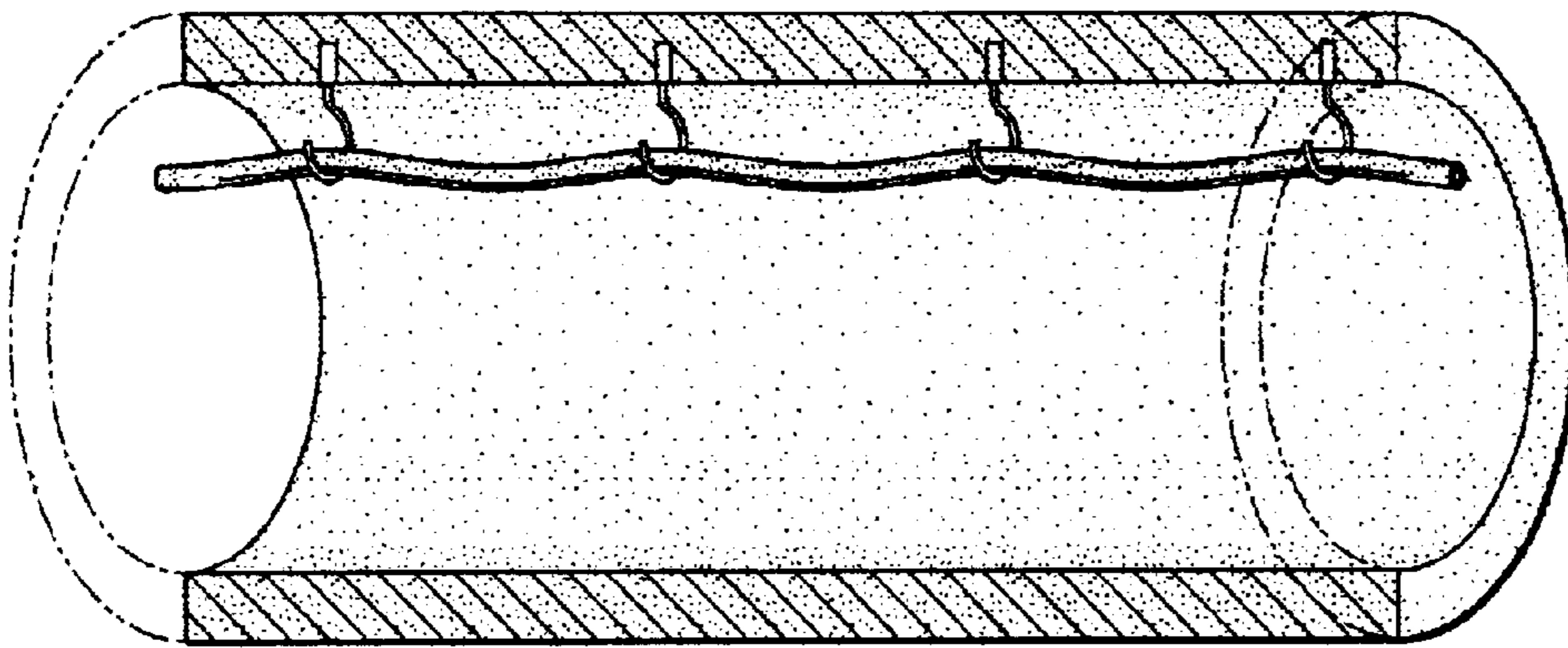
Fig. 1 (PRIOR ART)
