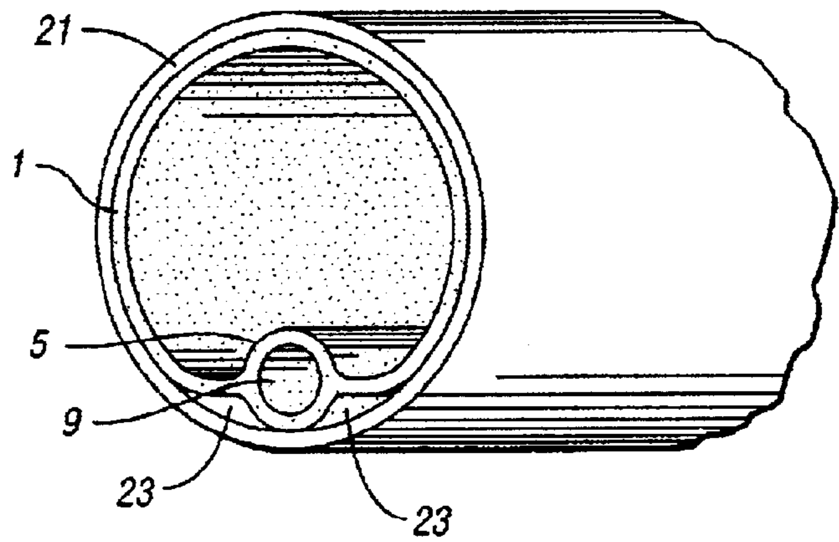
Fig. 2 (PRIOR ART)
