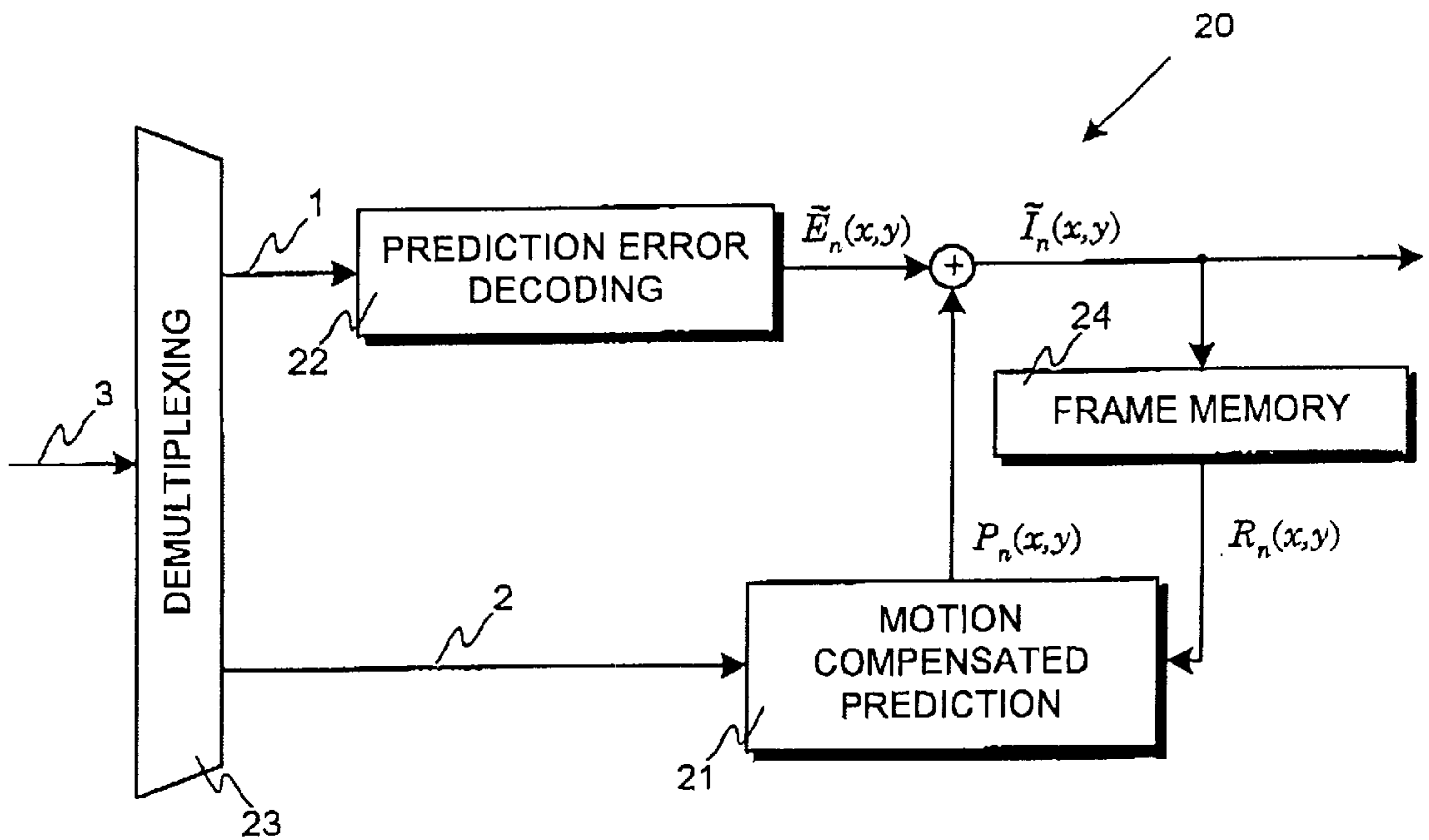
FIG. 2 PRIOR ART
