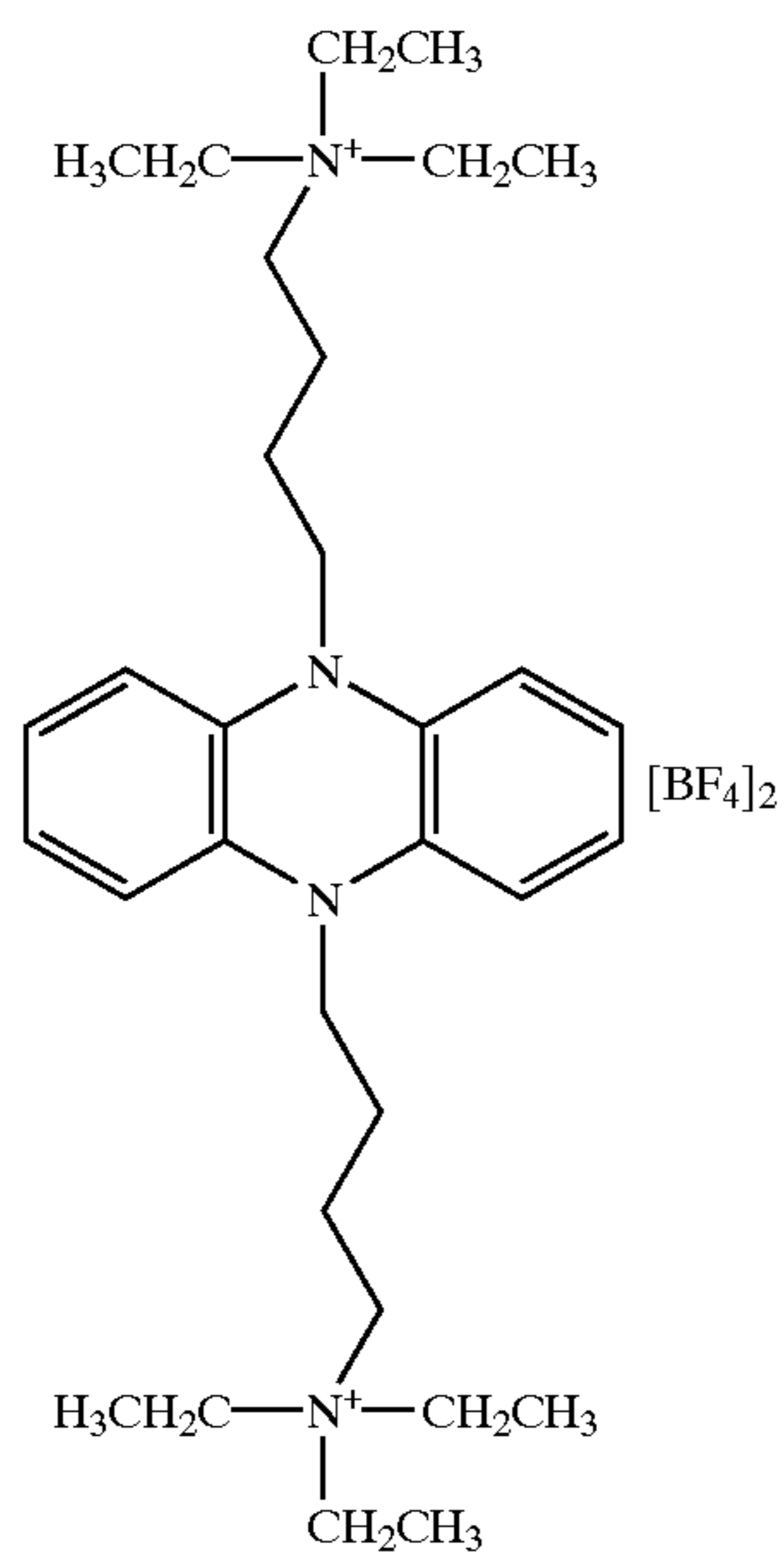
Bis-5,10-[4-(triethylammonium)butyl]-5,10-dihydrophenazine bis(tetrafluoroborate)
