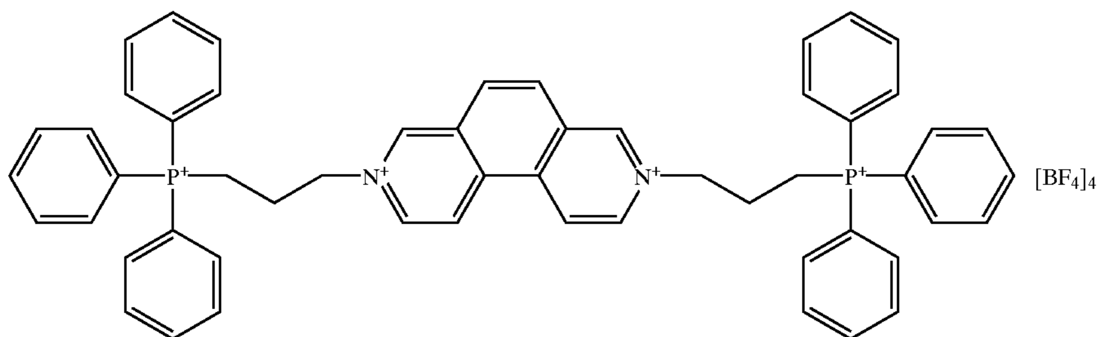
N,N'-bis(3-(triphenylphosphonium)propyl)-3,8-phenanthroline tetrakis(tetrafluoroborate)
