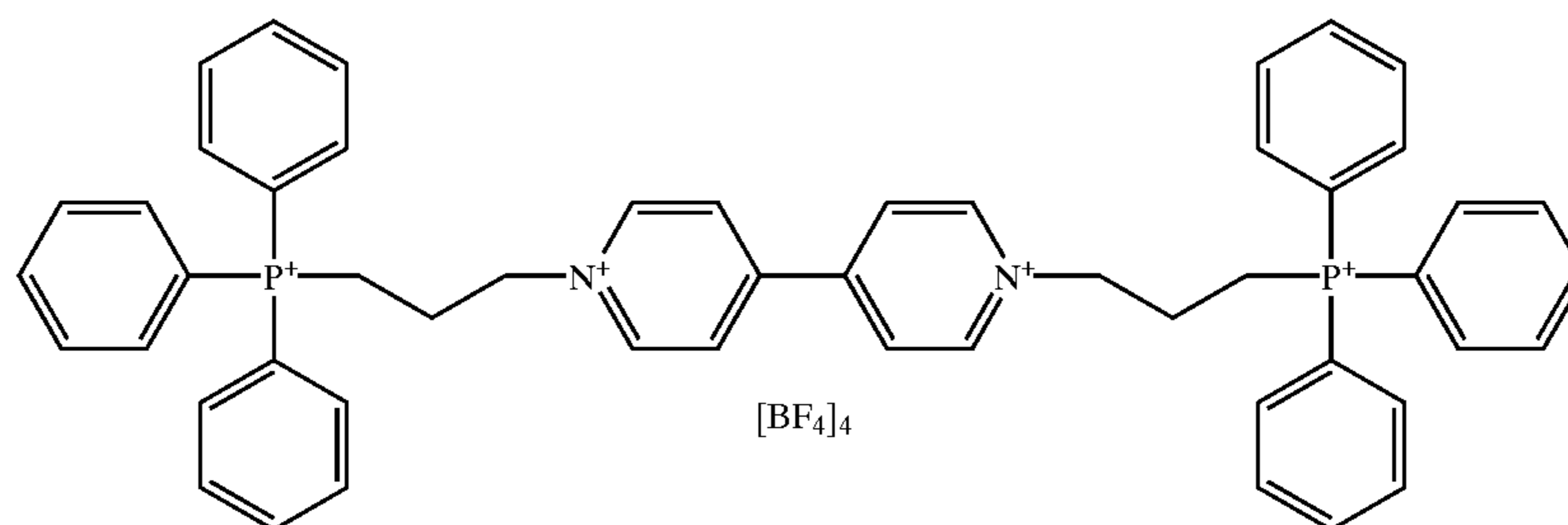
1,1'-bis(3-(triphenylphosphonium)propyl)-4,4'-dipyridinium tetrakis(tetrafluoroborate)
