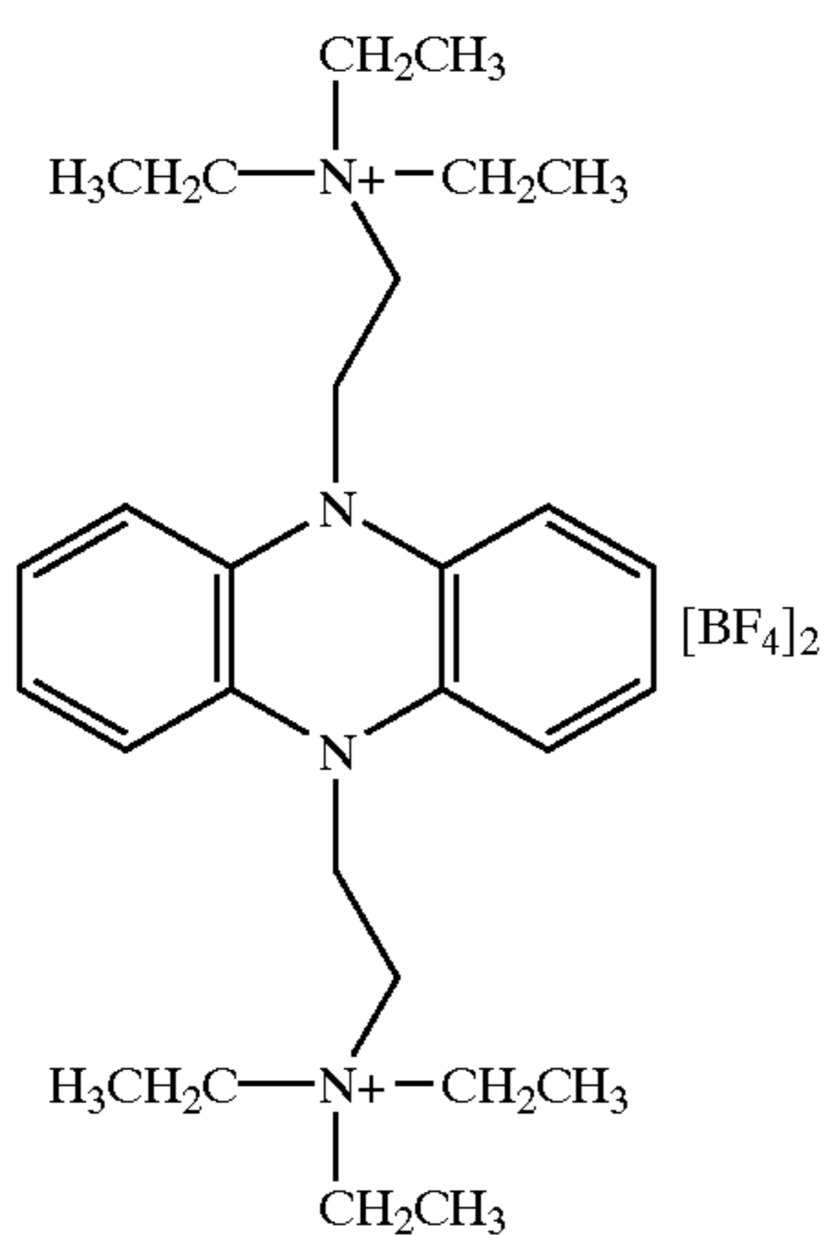
Bis-5,10-[2-(triethylammonium)ethyl]-5,10-dihydrophenazine bis(tetrafluoroborate)
