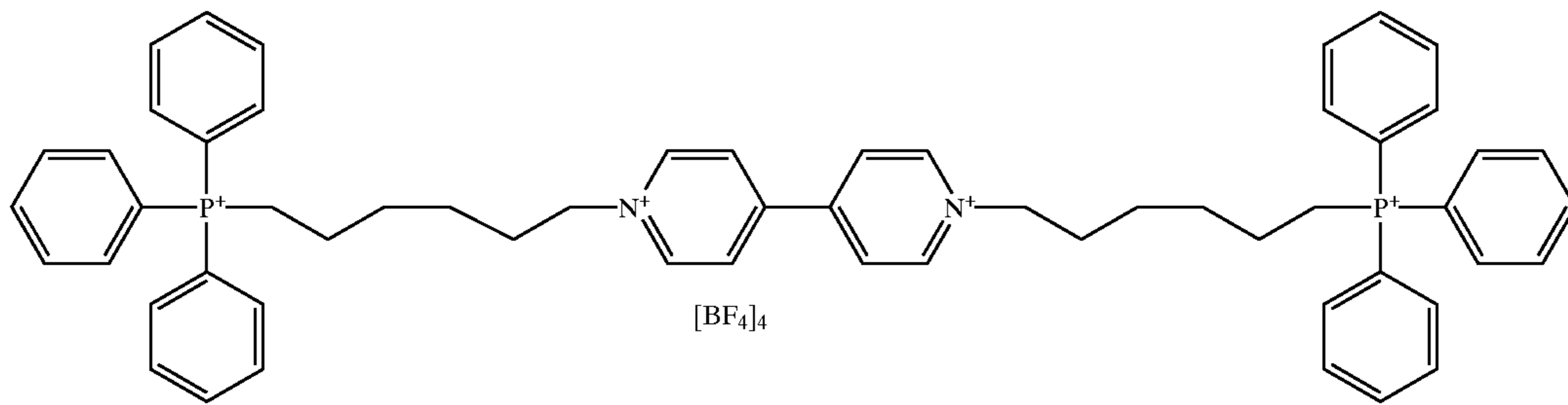
1,1'-bis(6-(triphenylphosphonium)hexyl)-4,4'-dipyridinium tetrakis(tetrafluoroborate)
