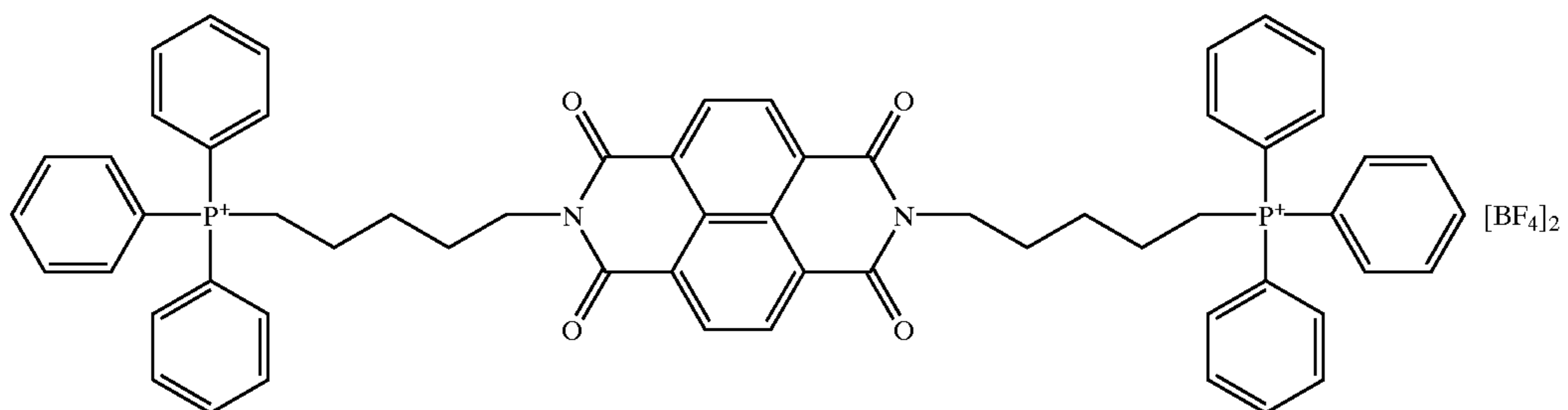
N,N'-bis(5-(triphenylphosphonium)pentyl)-1,4,5,8-naphthalenetetracarboxylic diimide bis(tetrafluoroborate)
