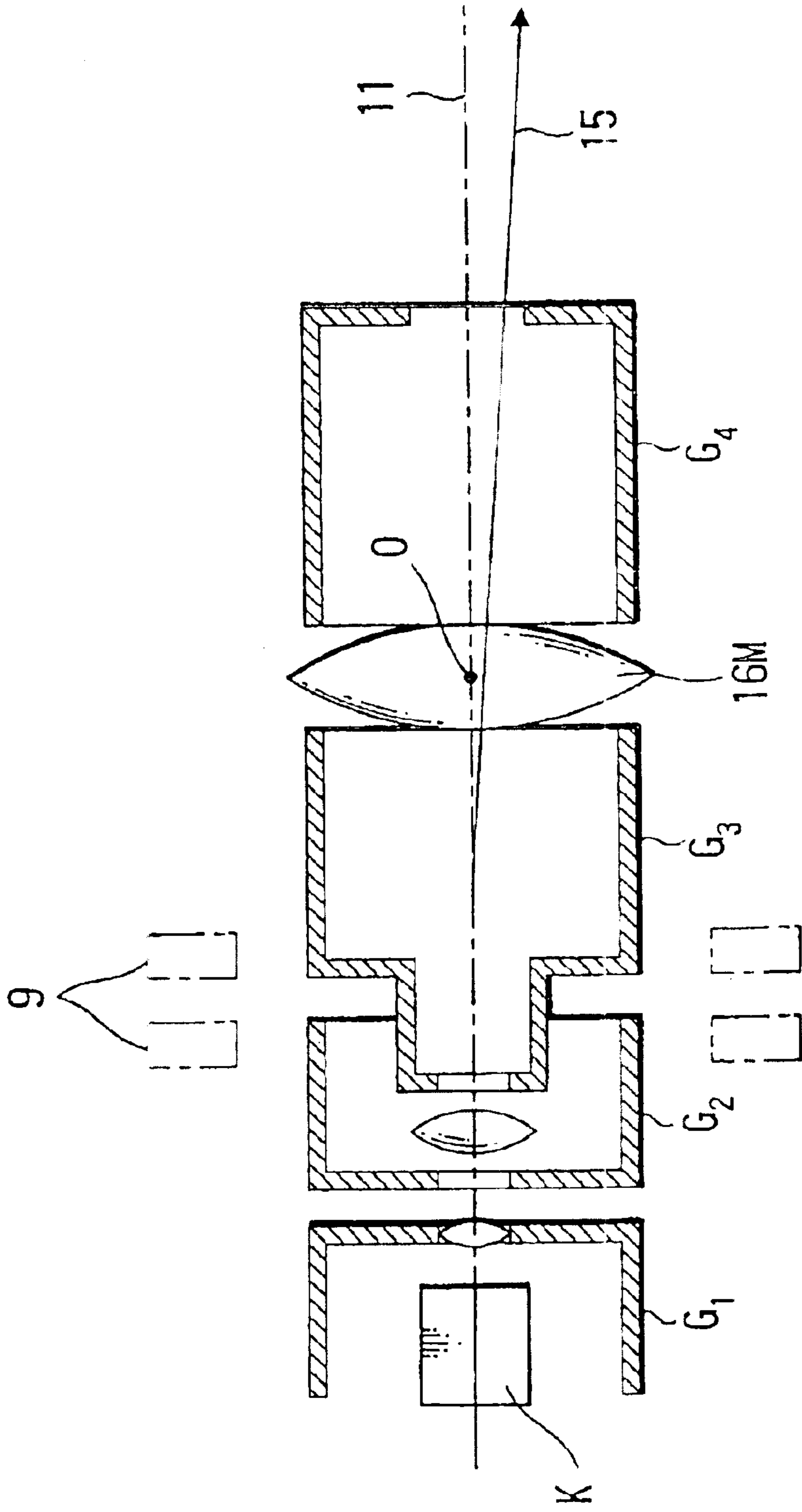
FIG. 3 (PRIOR ART)
