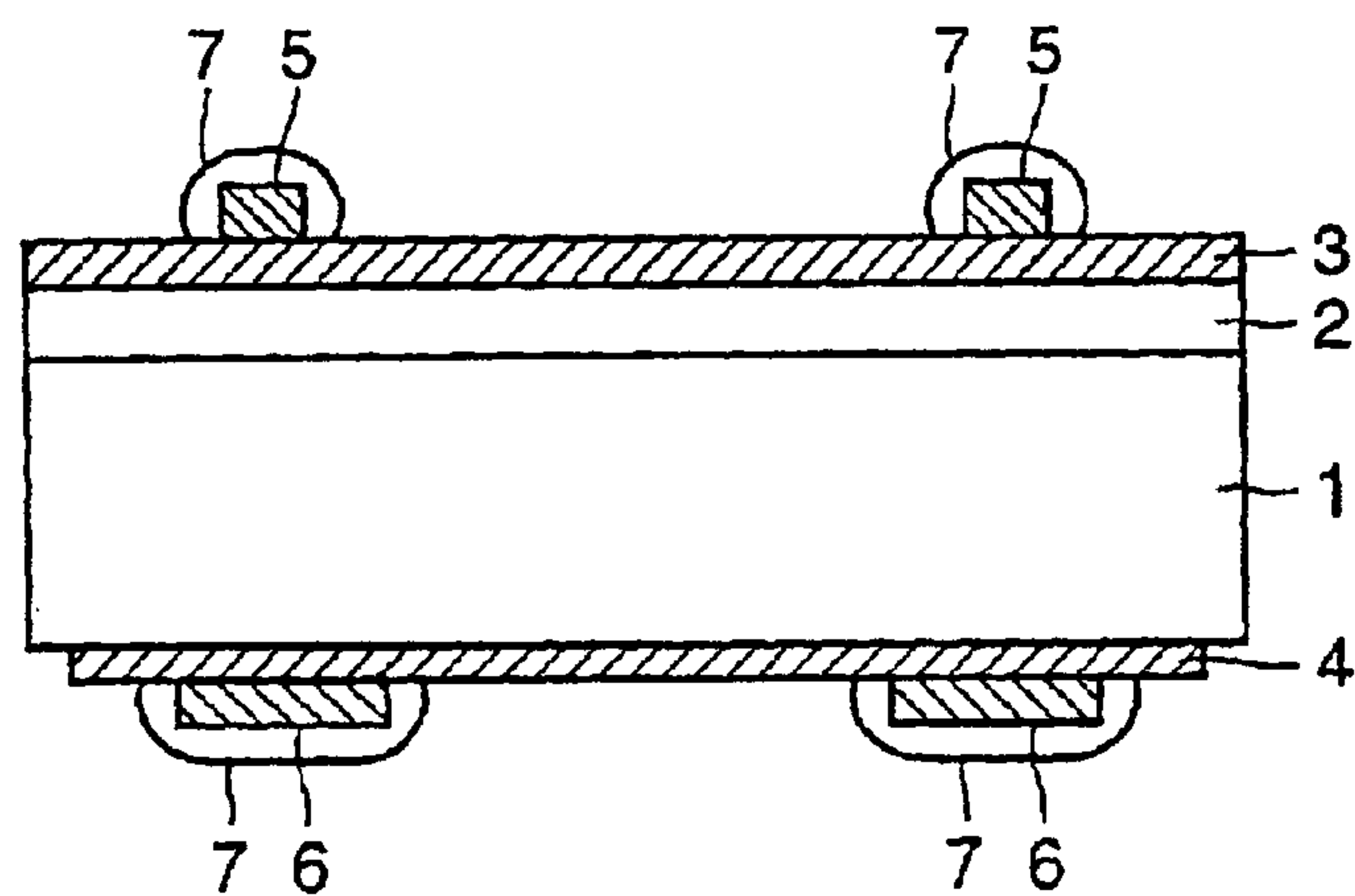
FIG.1 PRIOR ART
