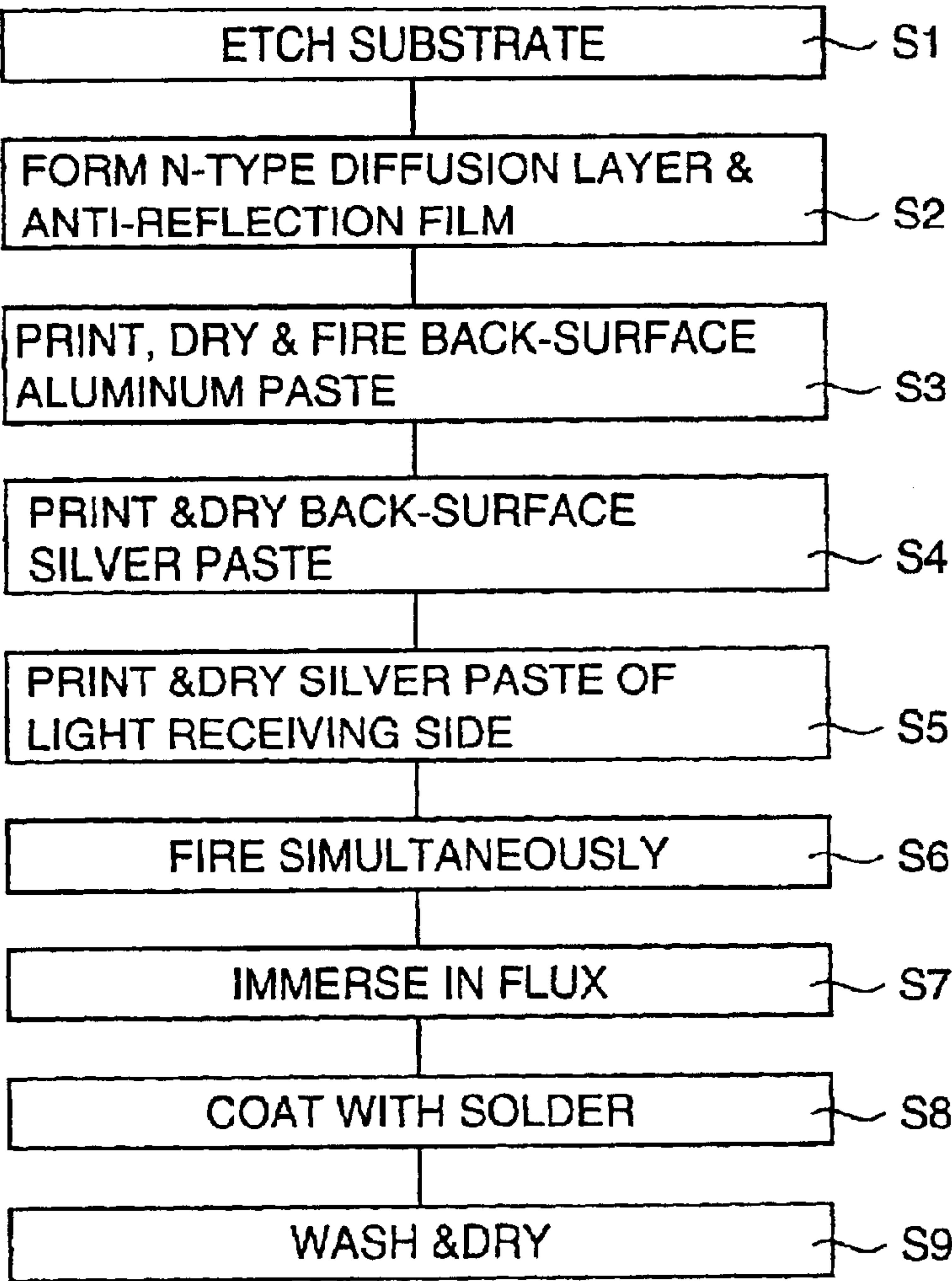
FIG.2 PRIOR ART
