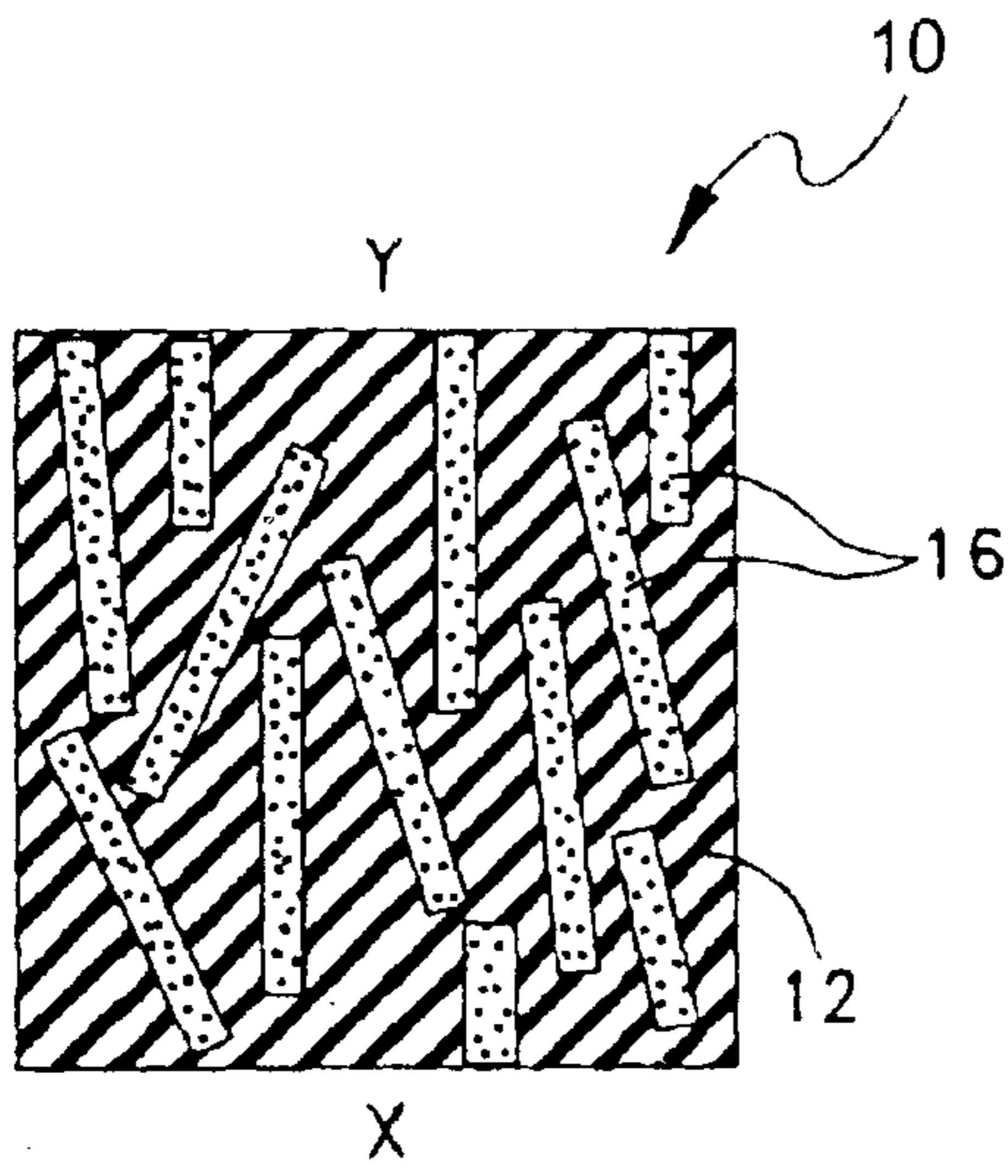
FIG. 1 (PRIOR ART)
