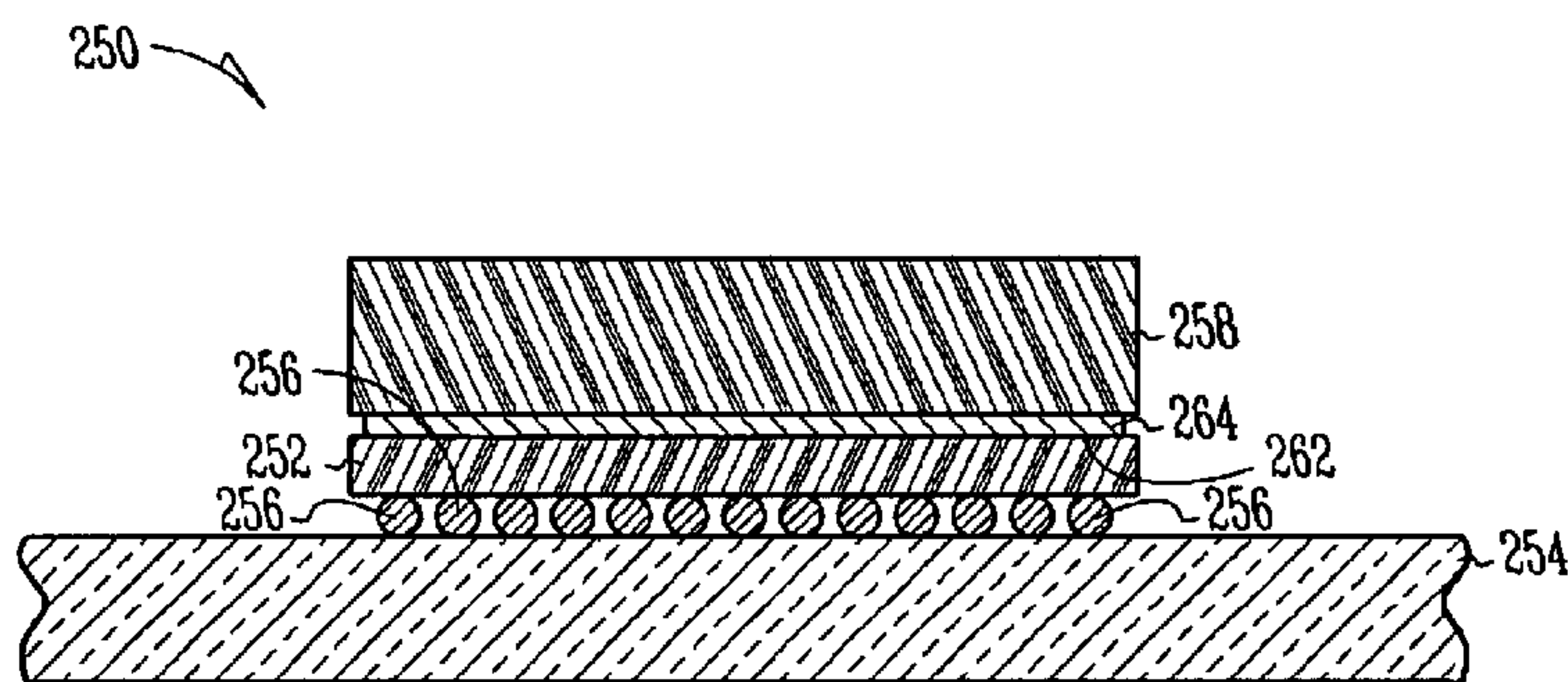
Fig. 29 (PRIOR ART)
