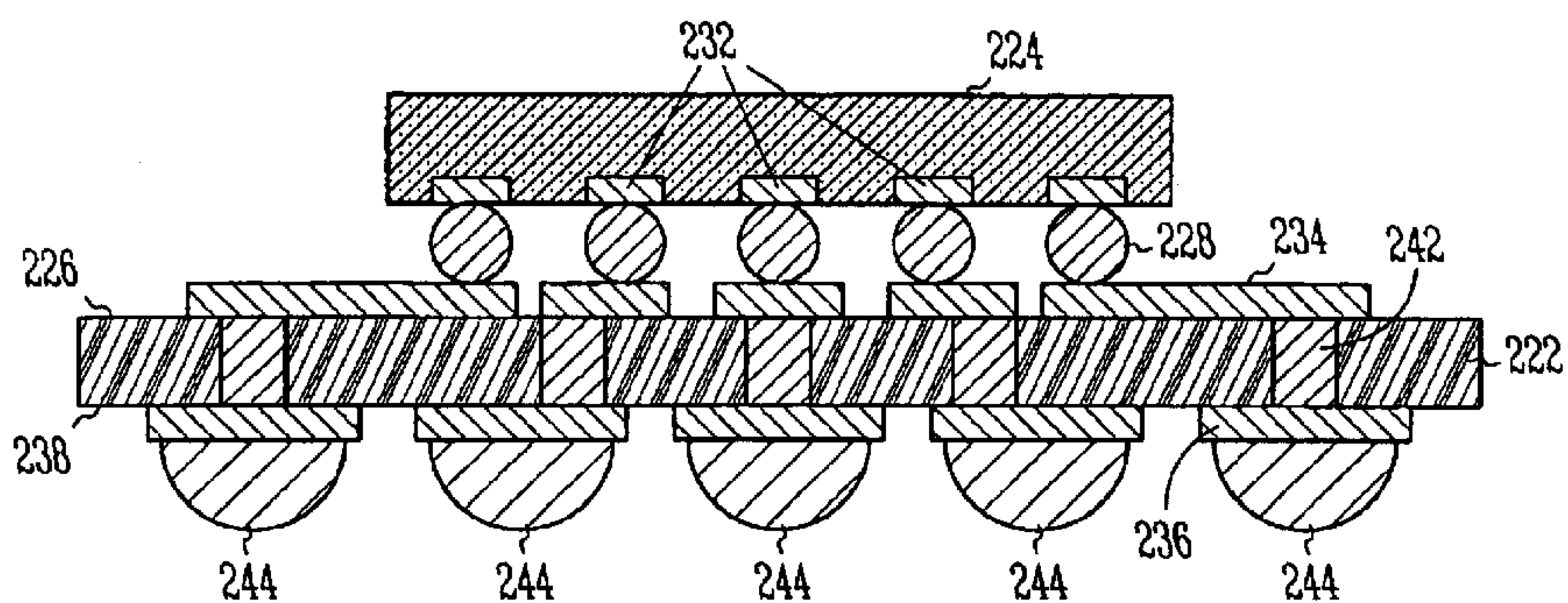
Fig. 28 (PRIOR ART)
