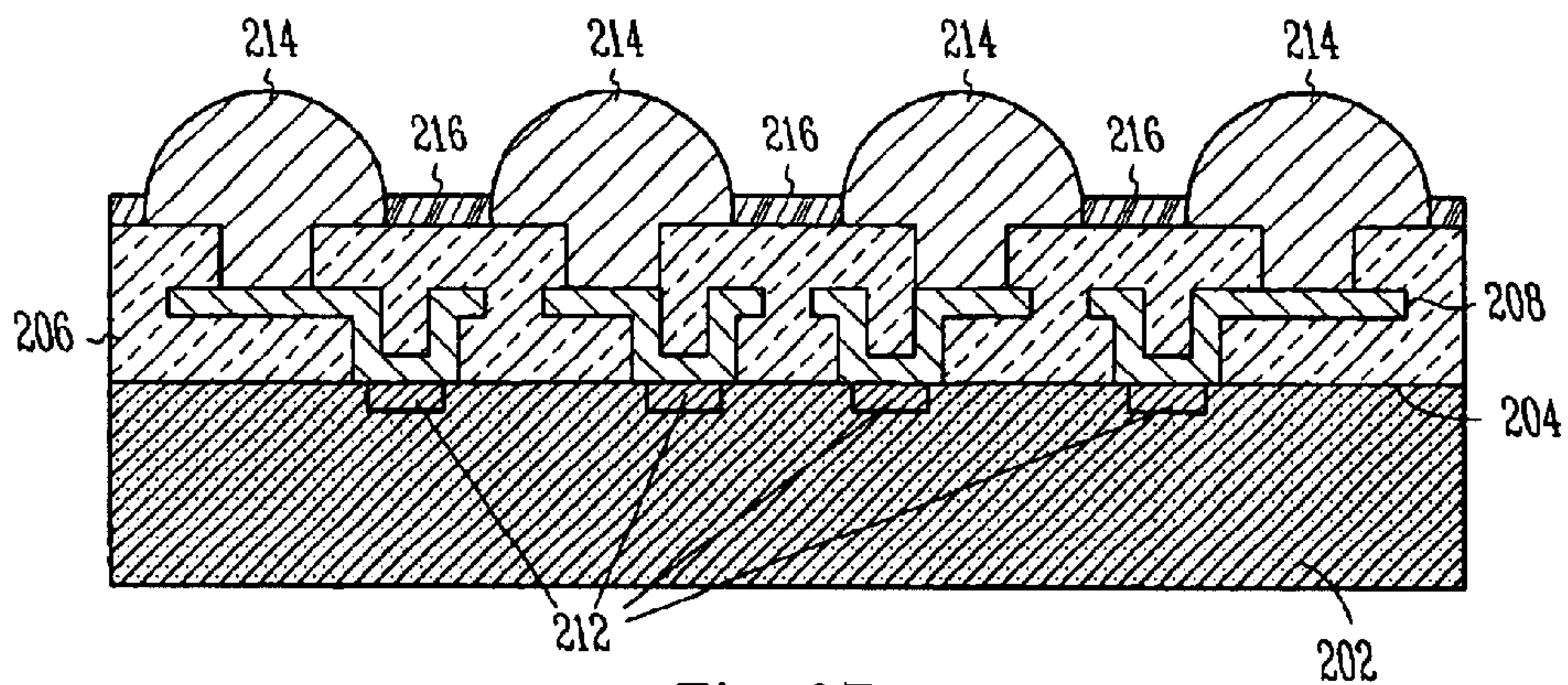
Fig. 27 (PRIOR ART)
