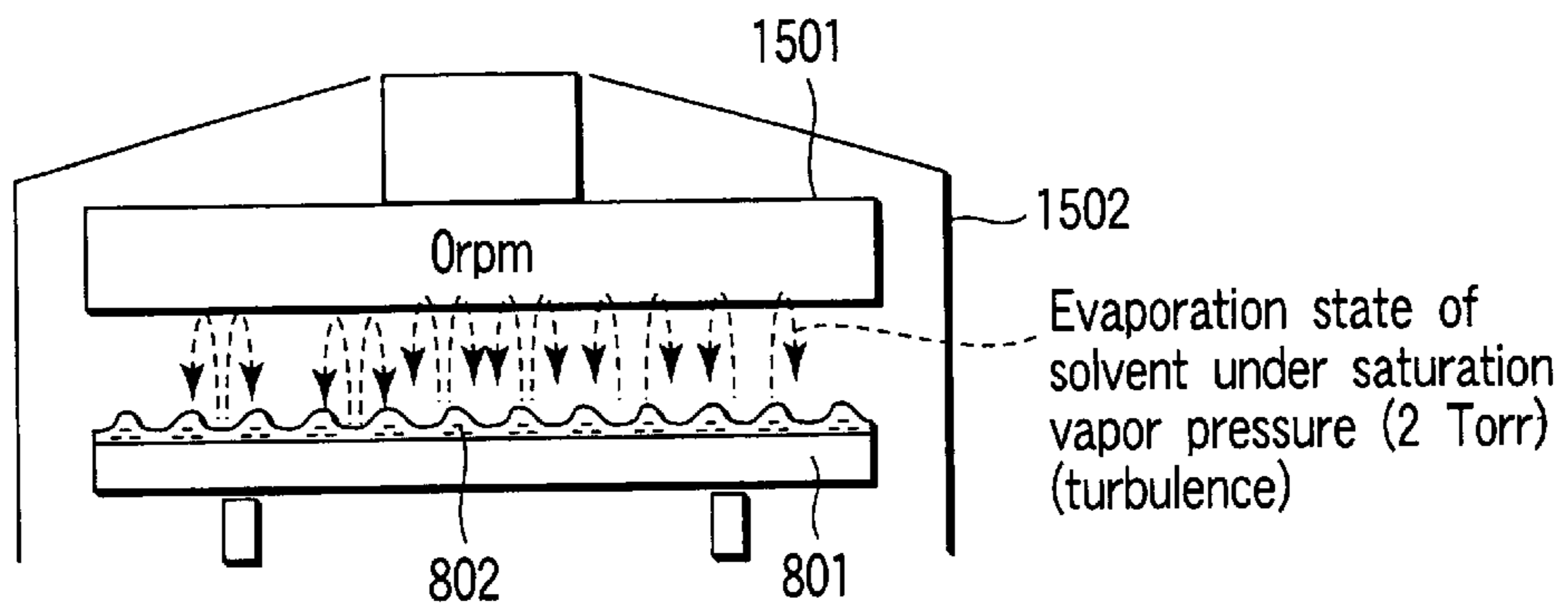
FIG. 16 PRIOR ART
