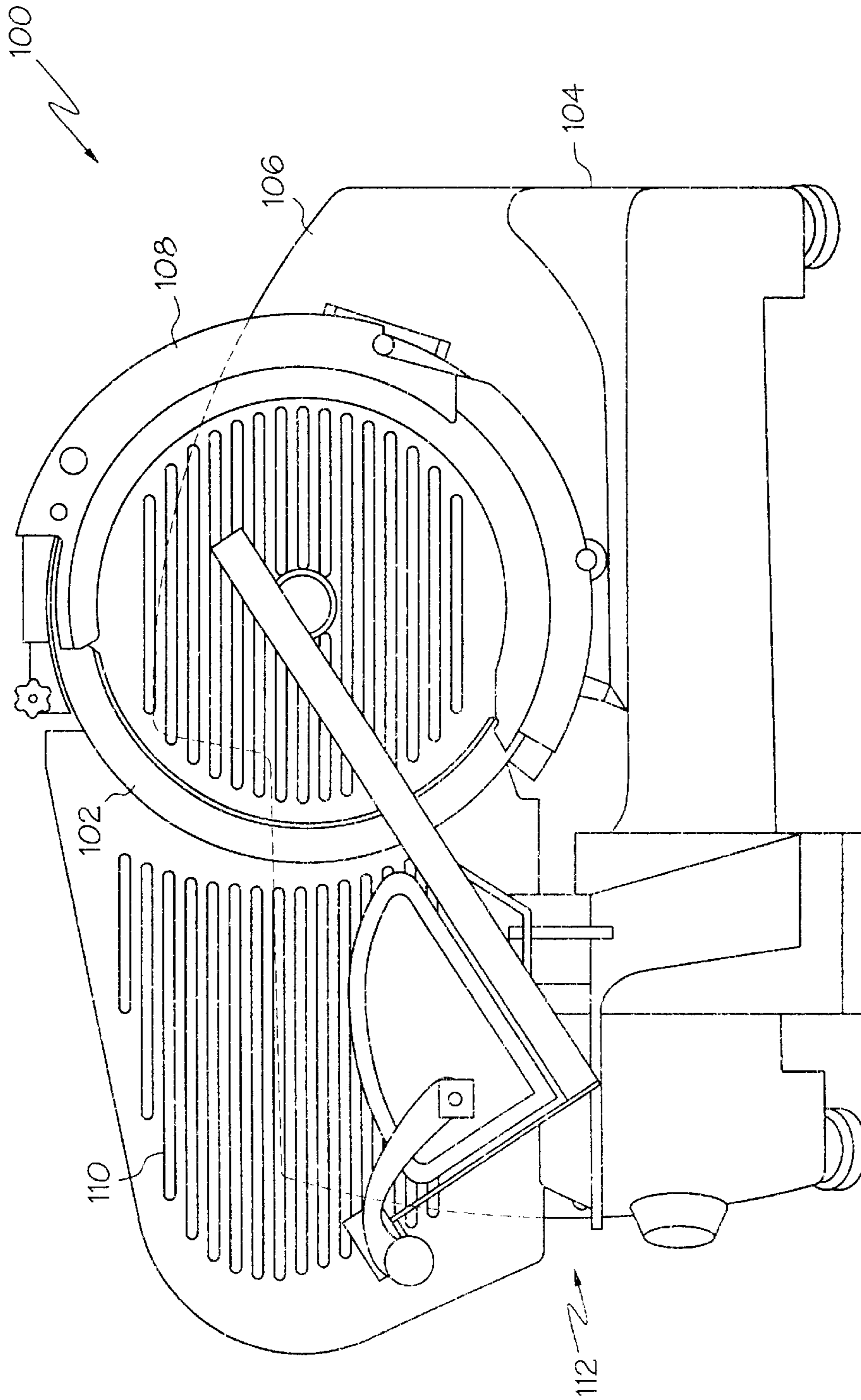
FIG. 1 PRIOR ART
