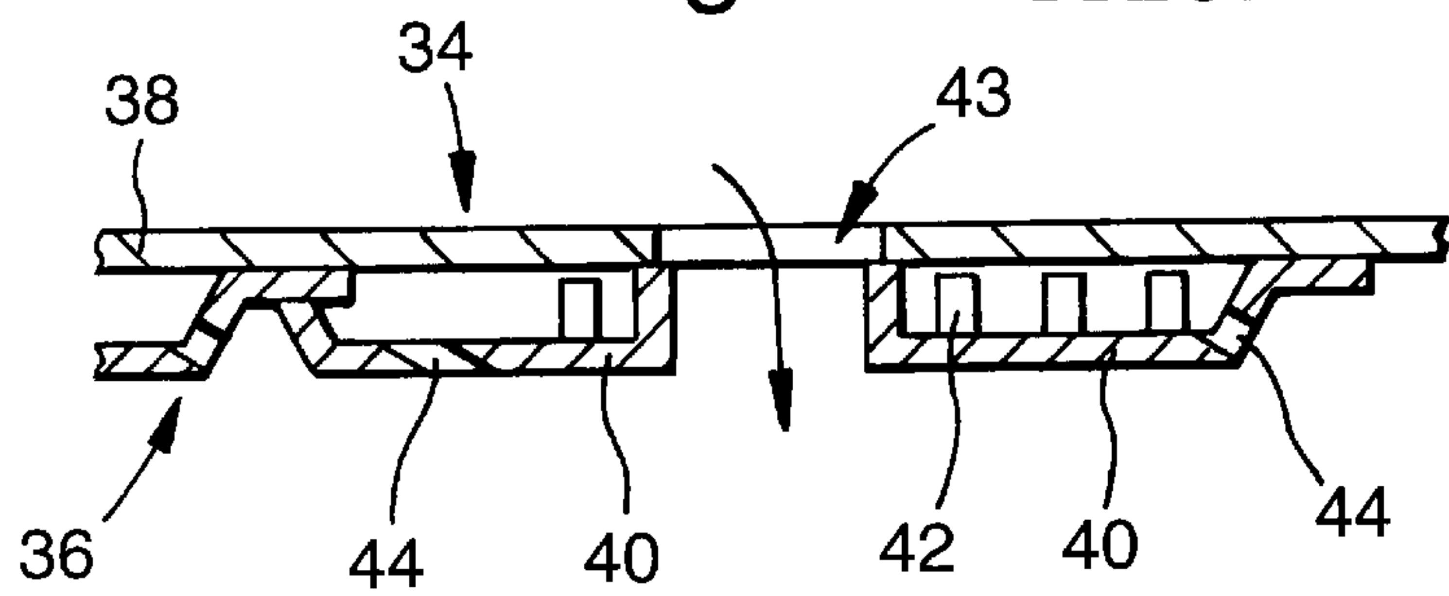
Fig.3. PRIOR ART
