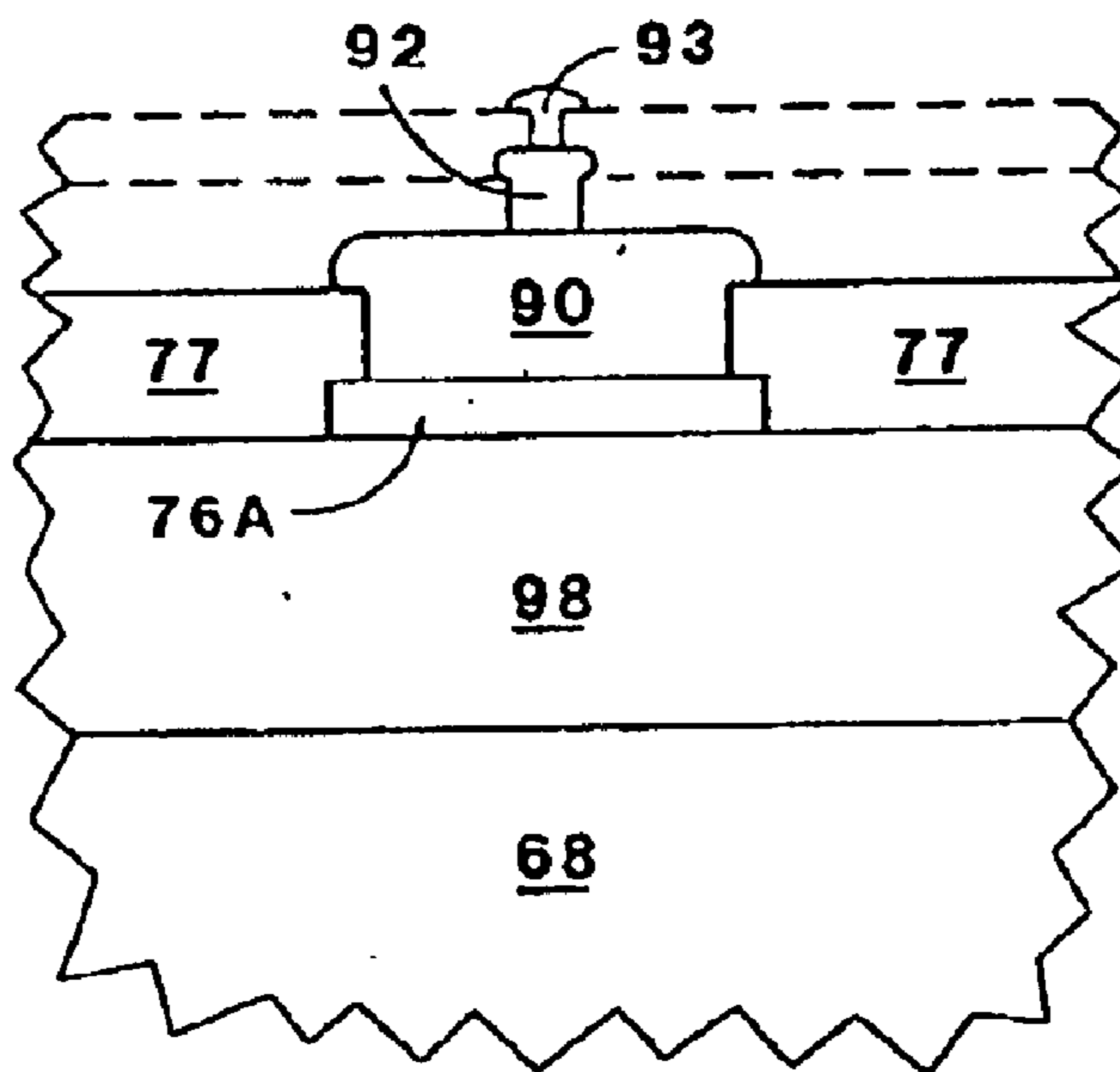
FIG. 11 PRIOR ART
