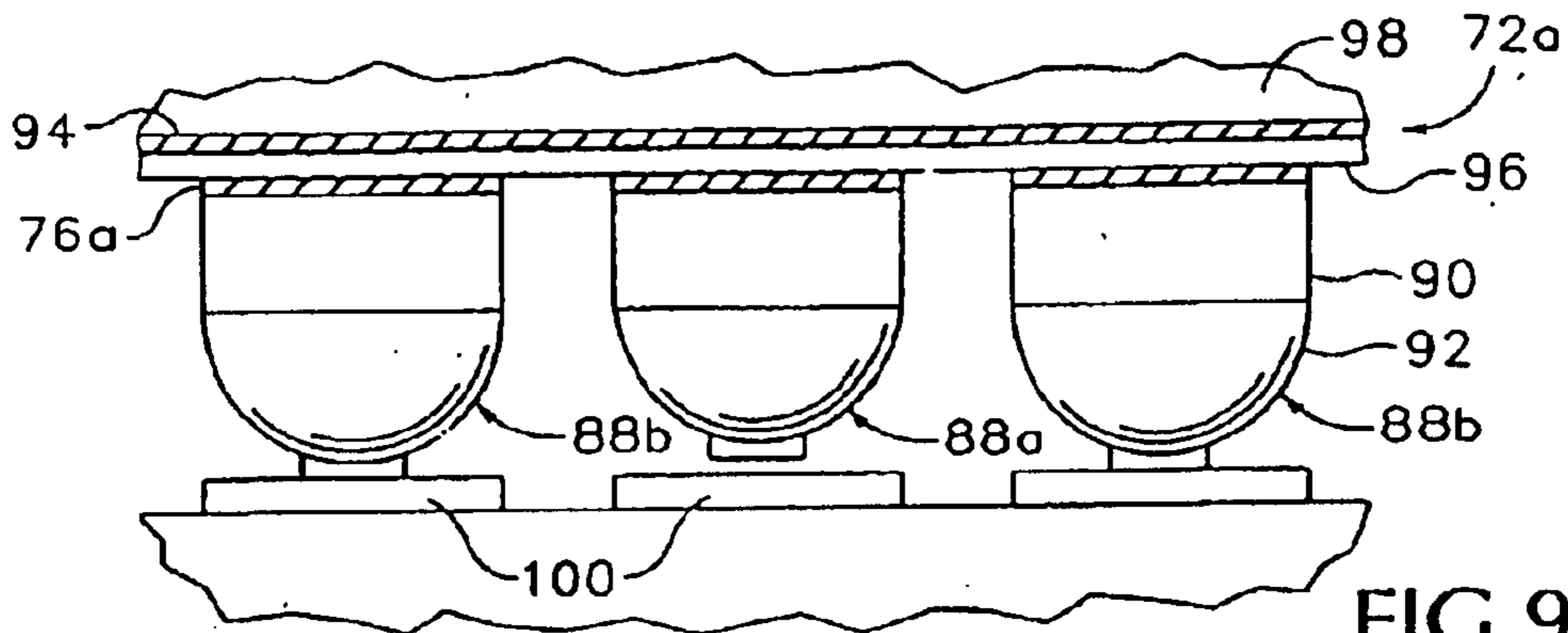
PRIOR ART
