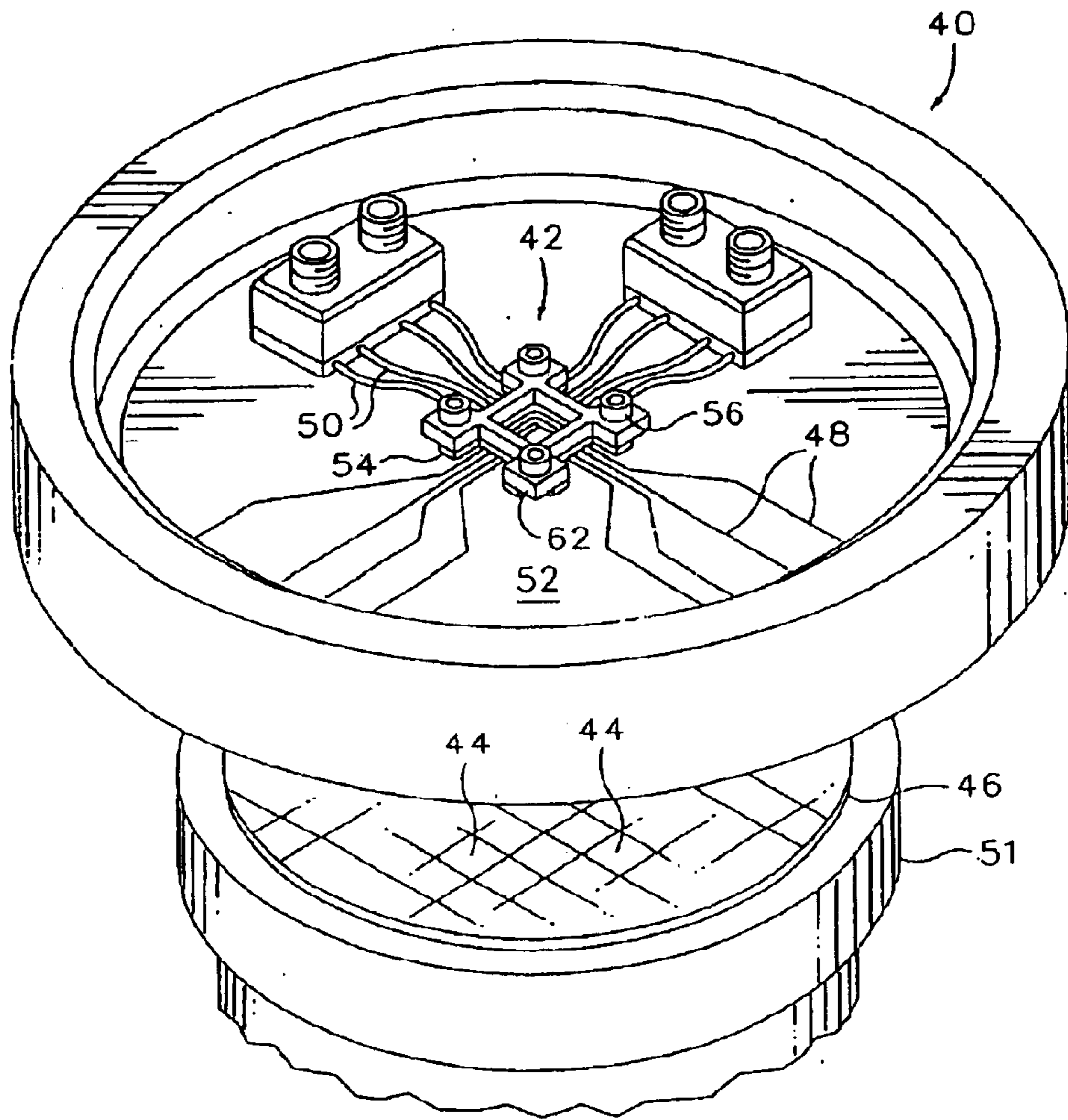
FIG.1 PRIOR ART
