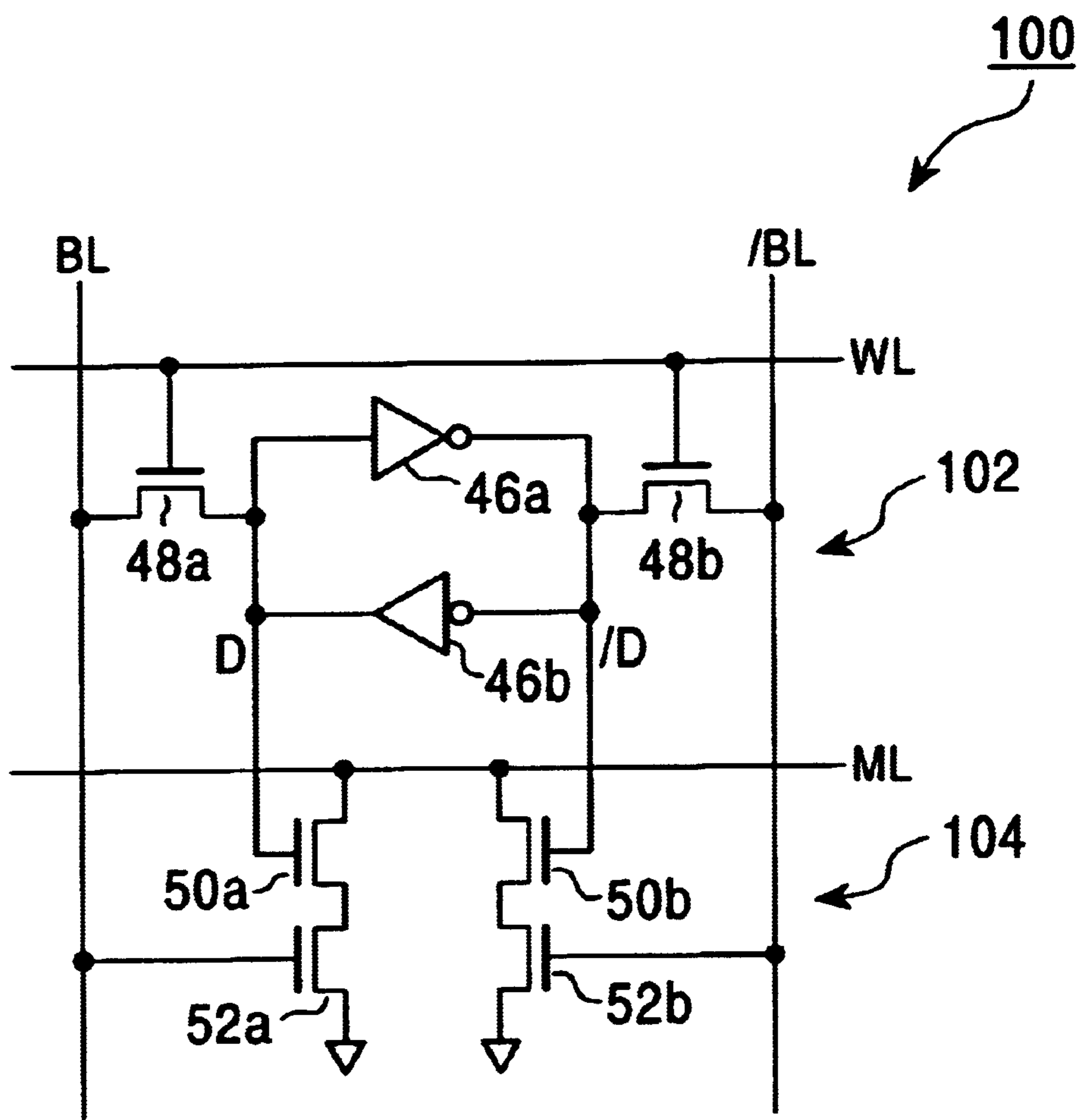
FIG. 11 PRIOR ART
