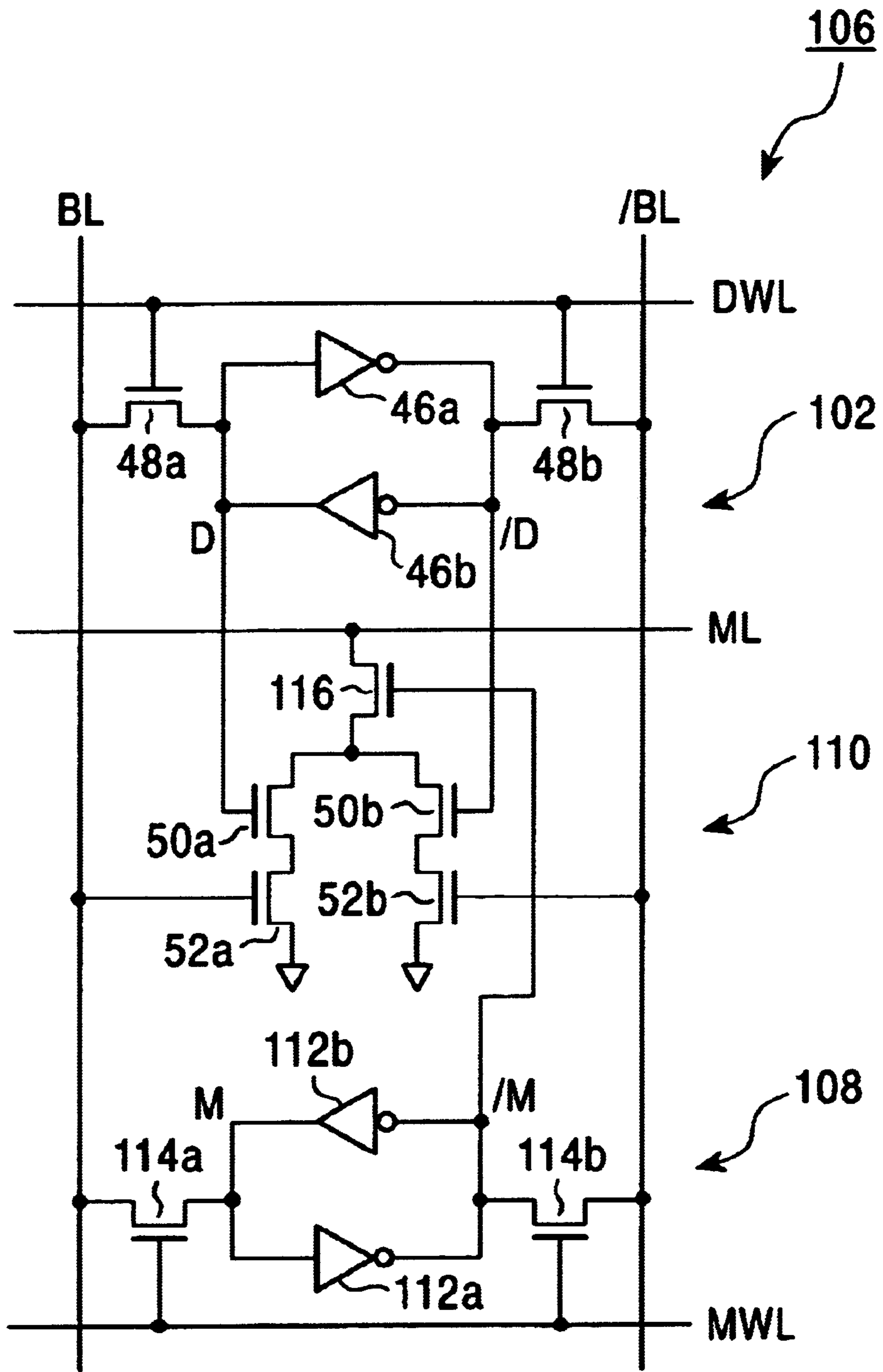
FIG. 12 PRIOR ART
