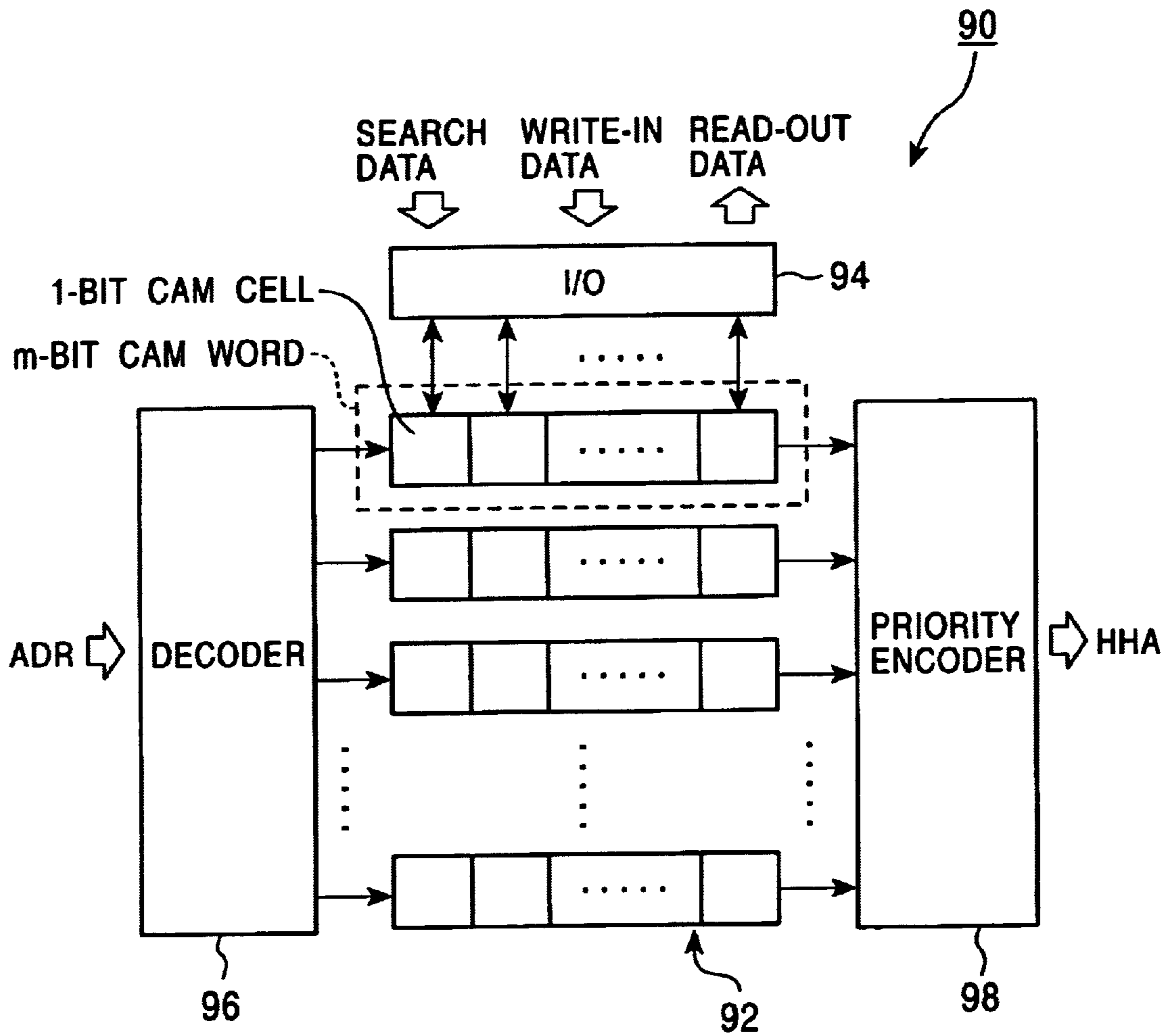
FIG. 10 PRIOR ART
