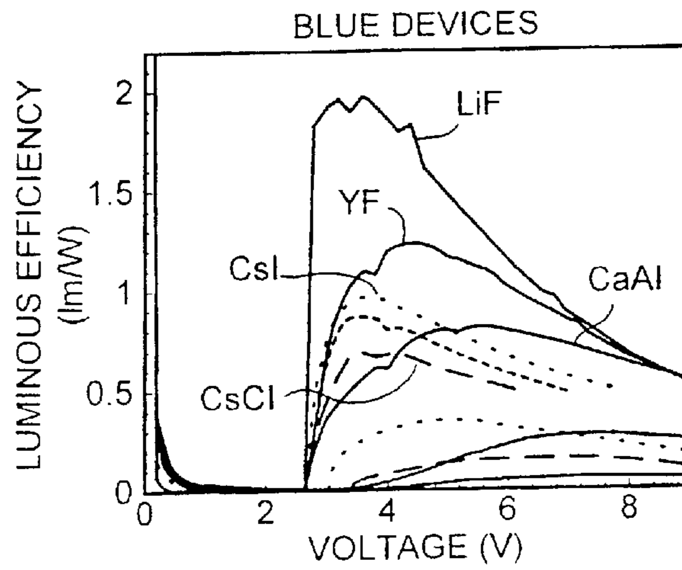
23691-23719: EL SPECTRA - xx/Ca/Al CATHODES
